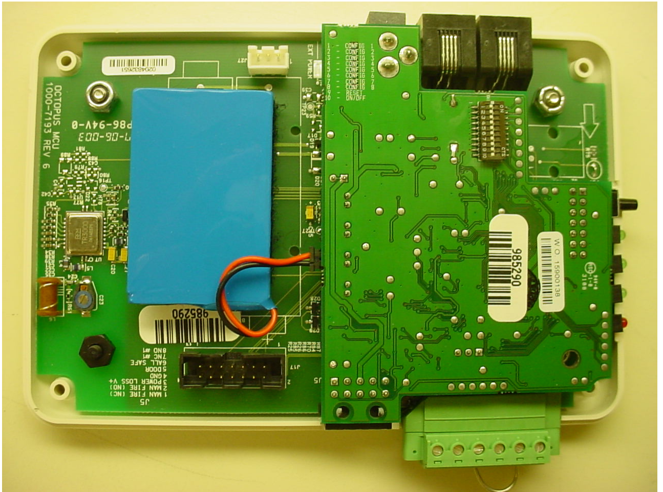
Figure 1: Assembled View
