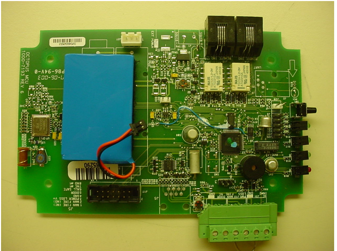
Figure 2: MCU PCB – Front
