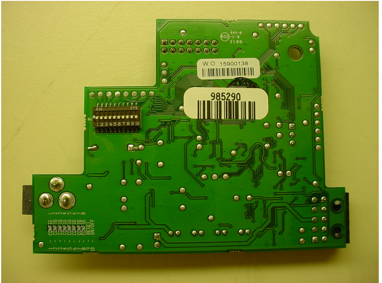
Figure 5: OEM PCB - Back
