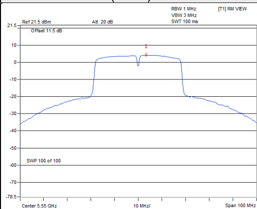
802.11n (HT40) / Chain 0 / Ch 110
