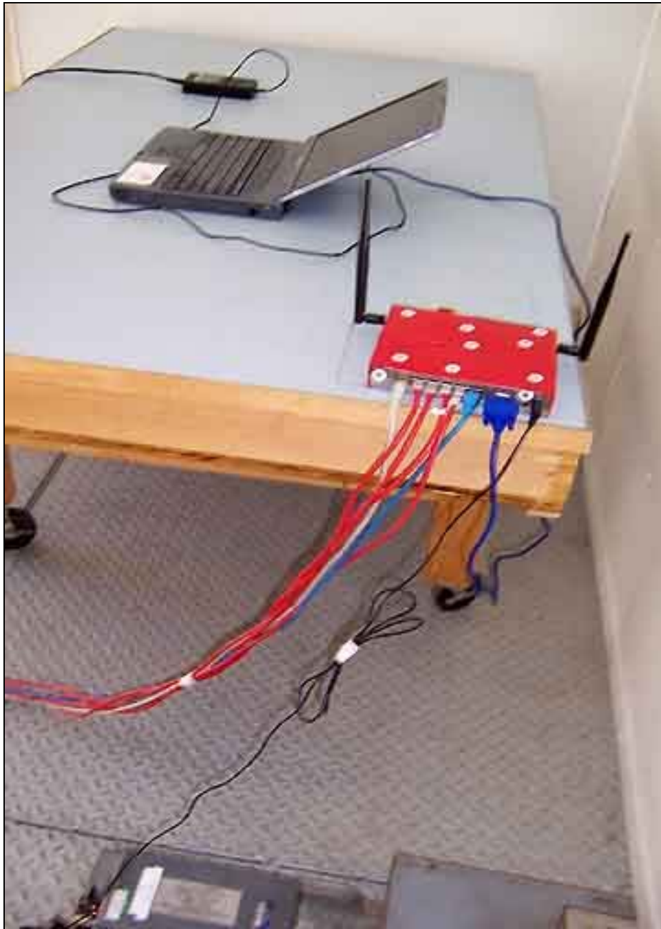
Mains Conducted Emissions - Side View
