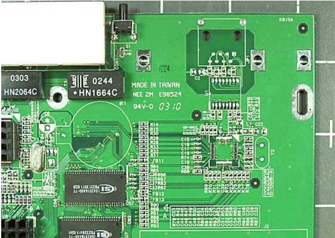
PCB Top #3
