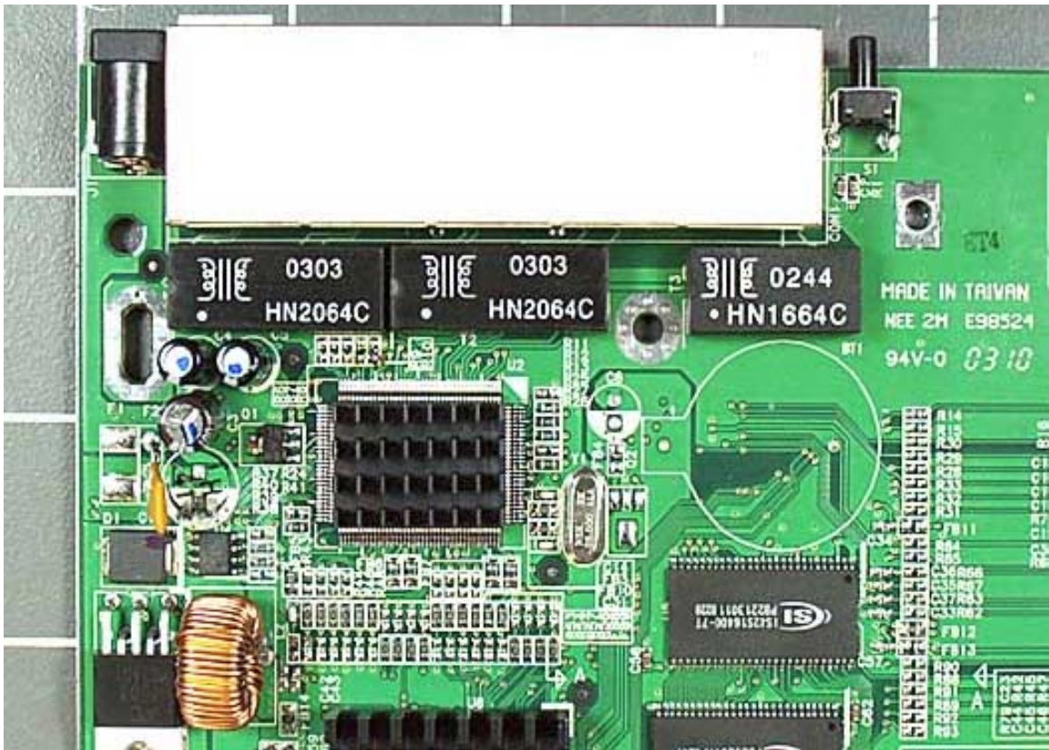
PCB Top #2
