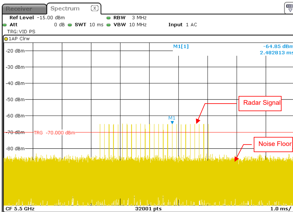
Radar Signal 2
