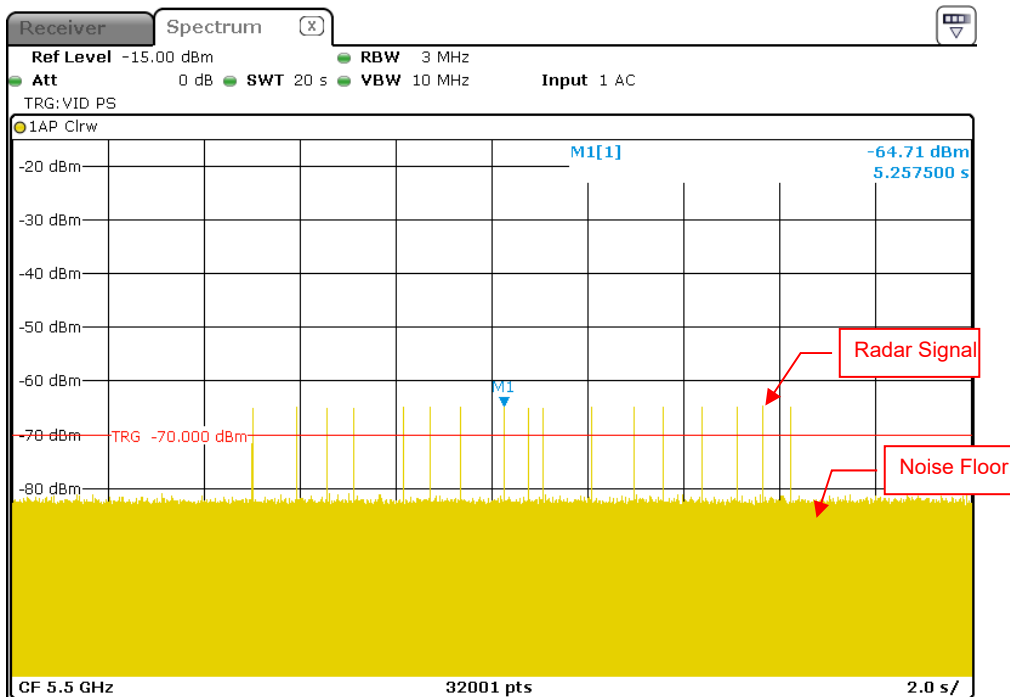
Radar Signal 5
