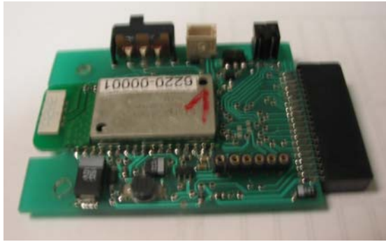
Head Unit RF top view
