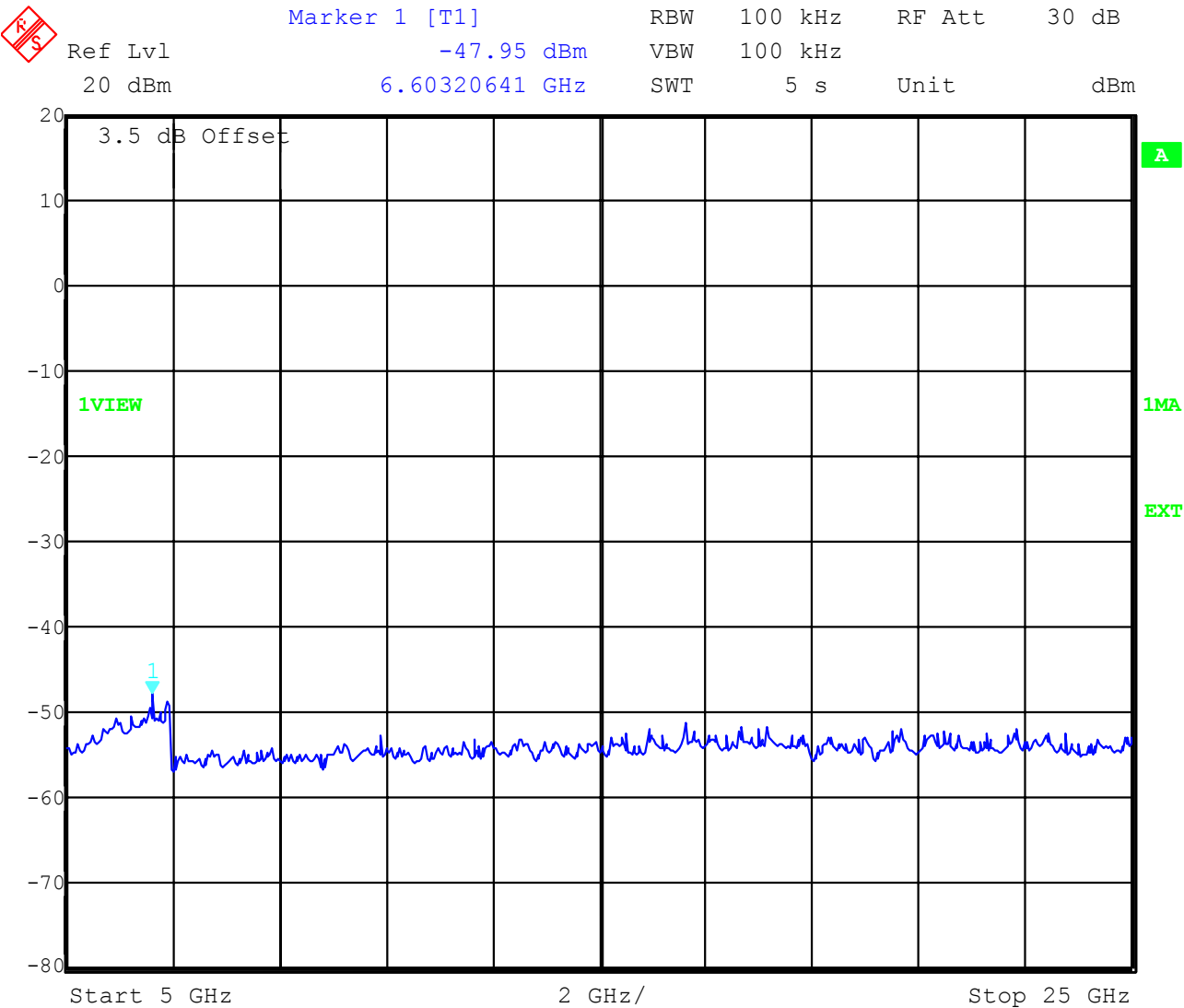
Plot 6, 2462 MHz
