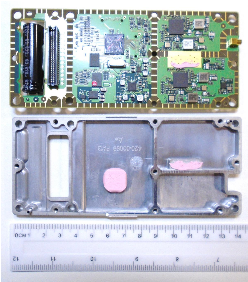
Figure 2 9770 – Bottom side lid removed showing inside of bottom side lid and bottom side of the SFX PCB (P3142-009a)
