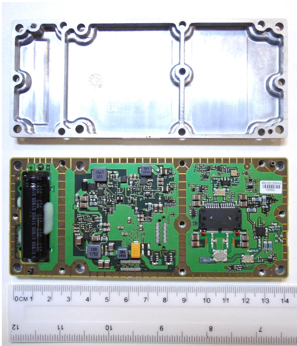
Figure 1 9770 – Top side lid removed showing inside of top side lid and top side of the SFX PCB (P3142-009a)
