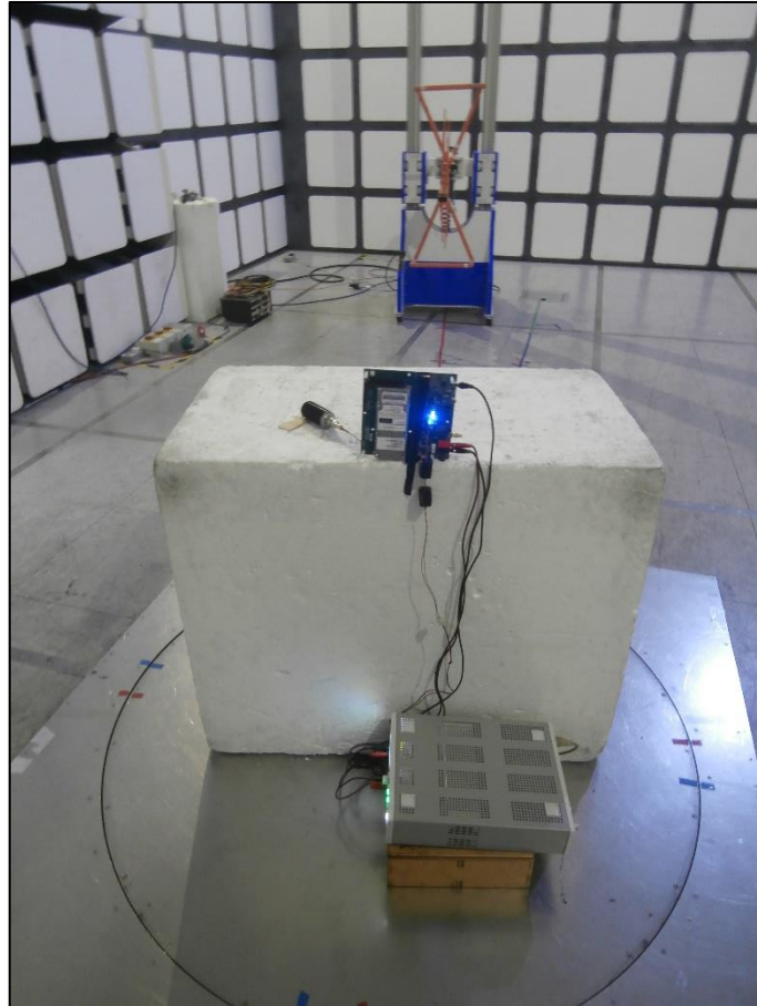
Figure 1 – Radiated Spurious Emissions - 30 MHz to 1 GHz
