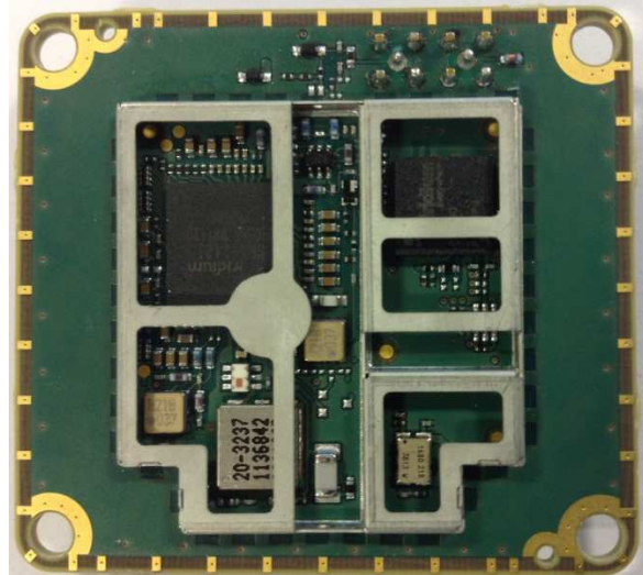
Figure 1 - Iridium 9602N top and bottom side views with bottom side screening can lid removed
