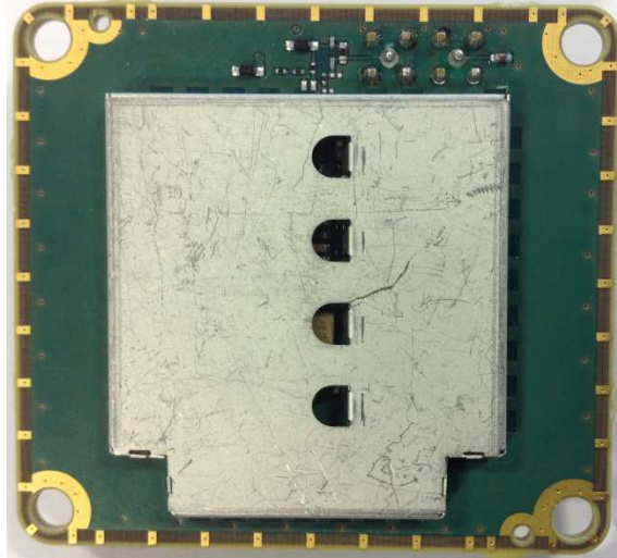
Figure 2 - Iridium 9602N bottom side view with screening can lid fitted
