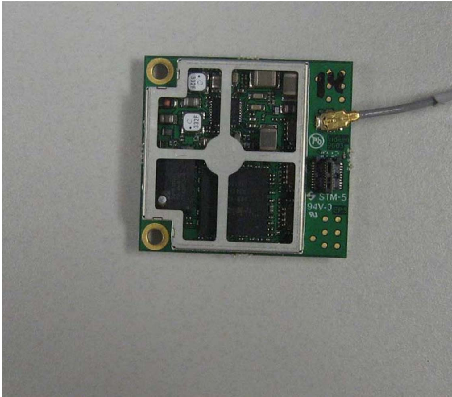
Internal Photos – Bottom Side with shield removed.
