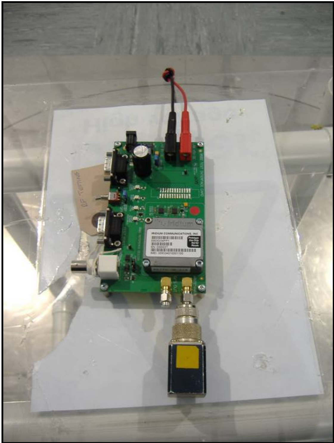
Radiated Emissions Test Setup – Close Up
