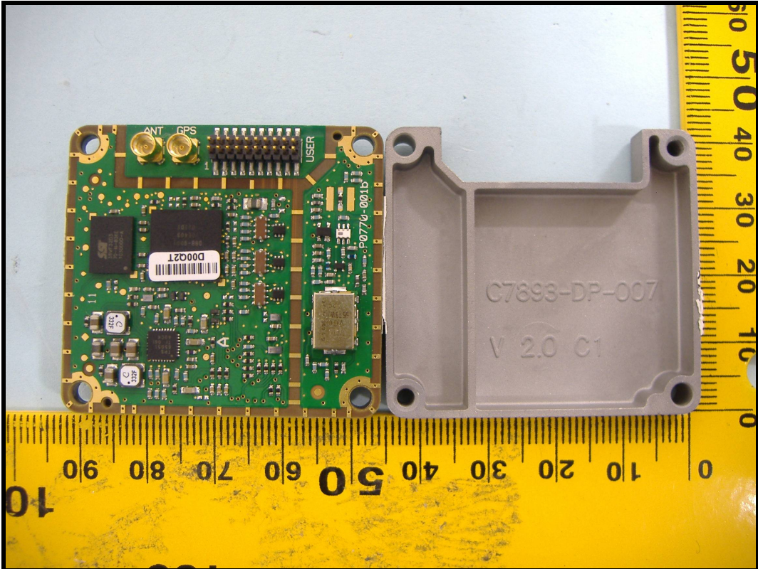
Bottom side of PCB Overview
