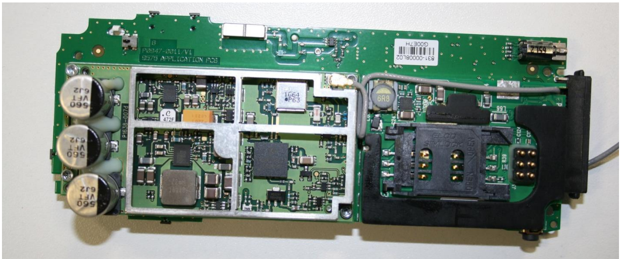
Figure 7 9575N – Bottom side of the Application Board PCB (P0947-001i/V1) with 9523N (P1638-007d) (screening can lid removed) and 9555g Satellite Phone SIM Board fitted
