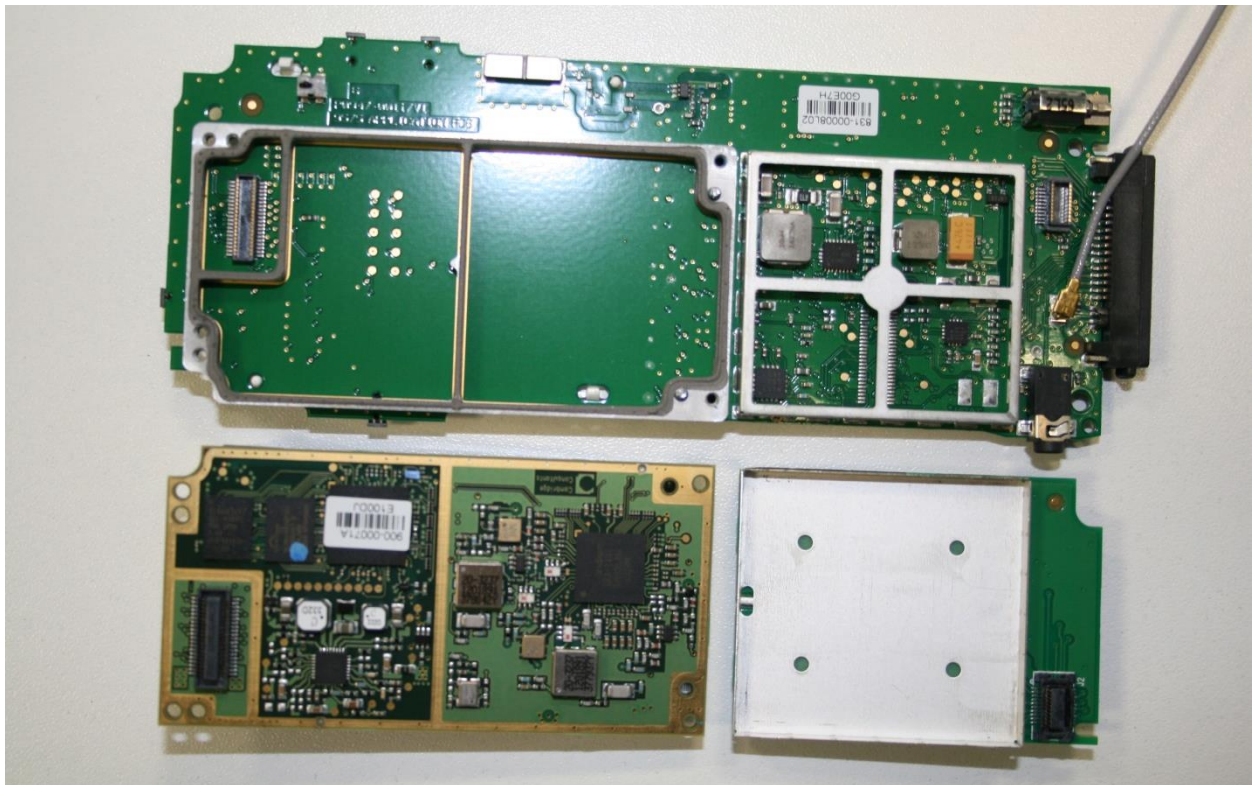
Figure 9 9575N – Bottom side of the Application Board PCB (P0947-001i/V1) with 9523N (P1638-007d) (bottom side) and 9555g Satellite Phone SIM Board (bottom side) removed
