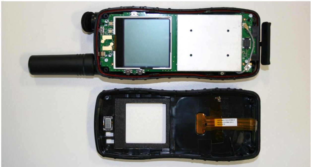
Figure 1 9575N – Front side lid removed showing top side of the Application Board PCB (P0947-001i/V1)
