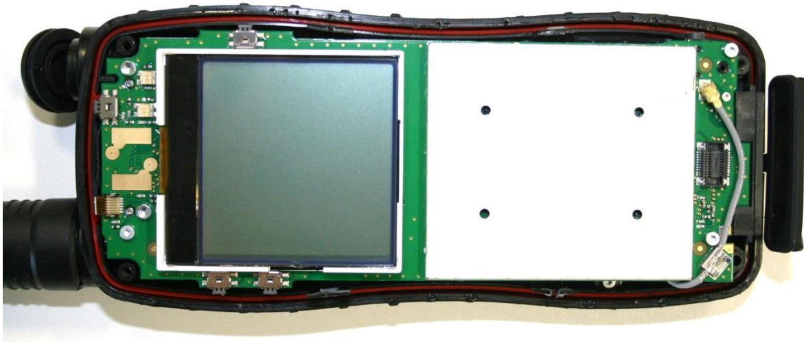
Figure 3 9575N – Front side lid removed showing top side of the Application Board PCB (P0947-001i/V1)
