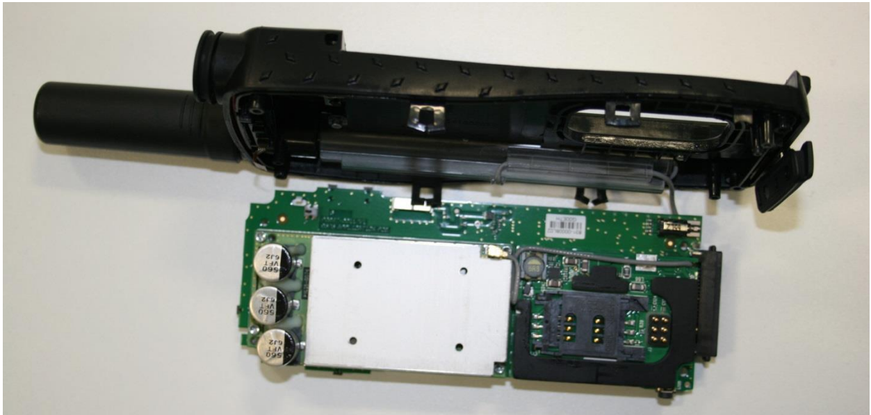
Figure 5 9575N – Bottom side of the Application Board PCB (P0947-001i/V1) with 9523N (P1638-007d) and 9555g Satellite Phone SIM Board fitted
