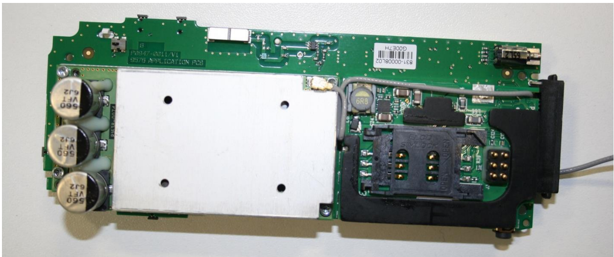
Figure 6 9575N – Bottom side of the Application Board PCB (P0947-001i/V1) with 9523N (P1638-007d) and 9555g Satellite Phone SIM Board fitted
