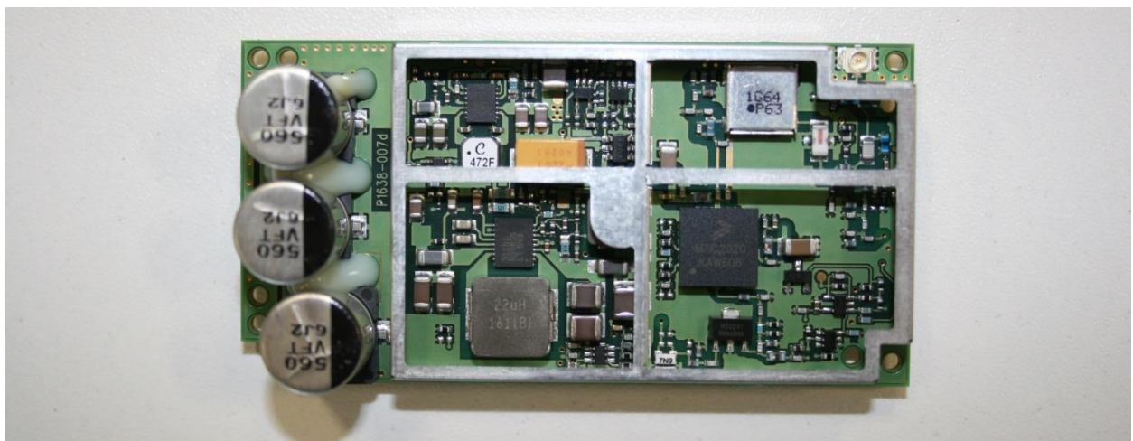
Figure 10 9575N – Top side of 9523N (P1638-007d) (screening can removed)
