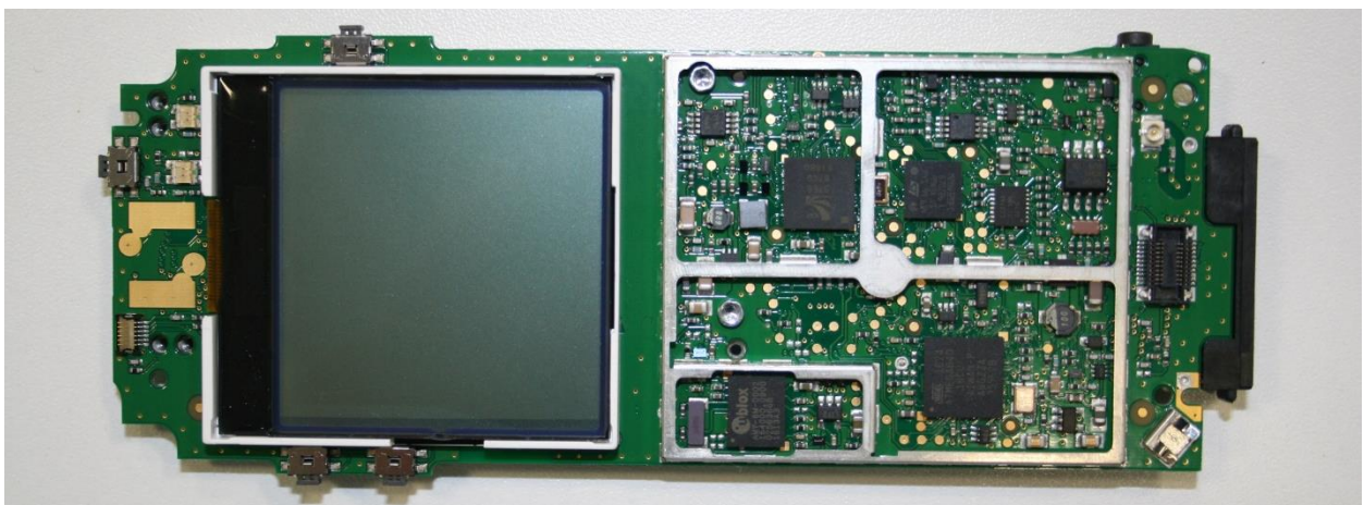
Figure 4 9575N – Top side of the Application Board PCB (P0947-001i/V1) (screening can removed)
