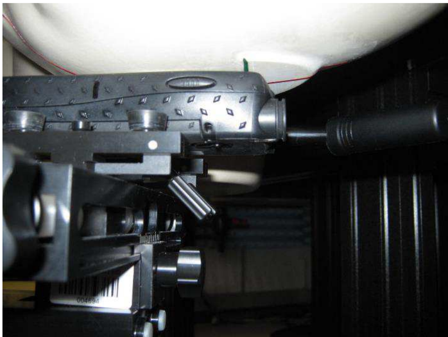
SAR: LH Cheek- Antenna Position 3 (Retracted by 60mm)
