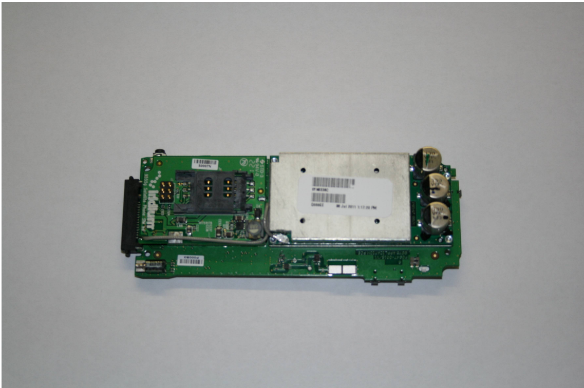
Core Back
