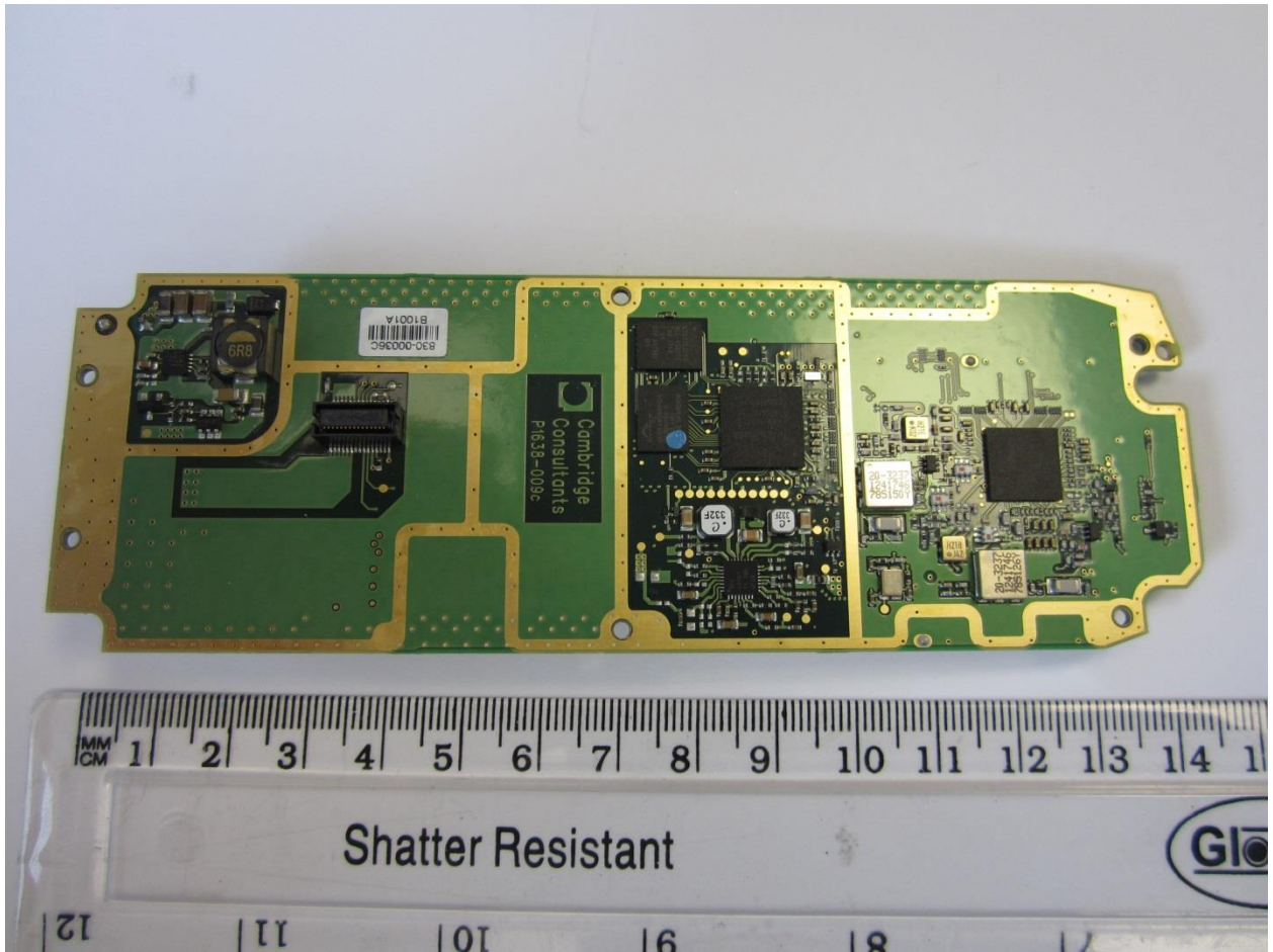
Front of Transceiver Board
