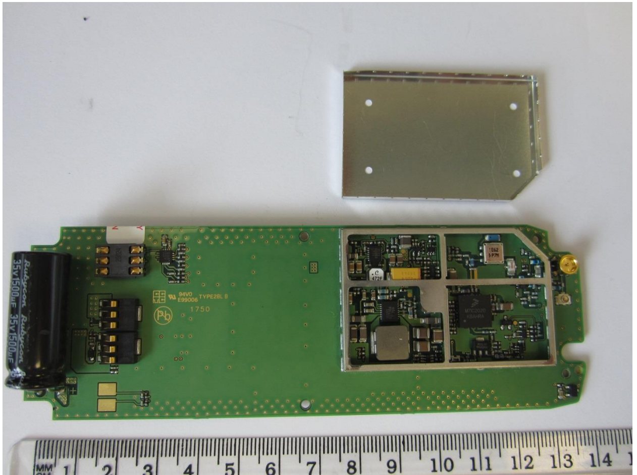
Rear of Transceiver Board with Screening Can Removed
