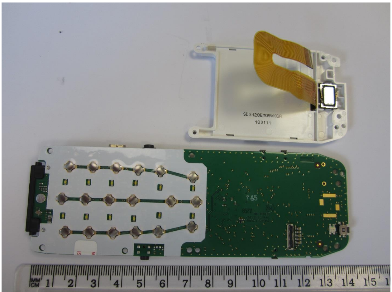
Front View of Application Board with LCD Removed
