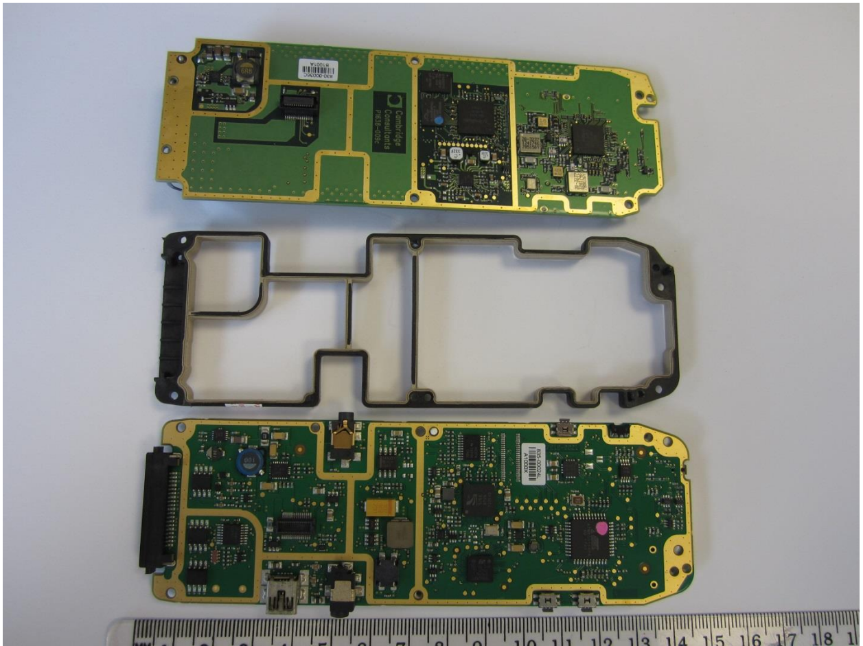
Electronics Assembly separated
