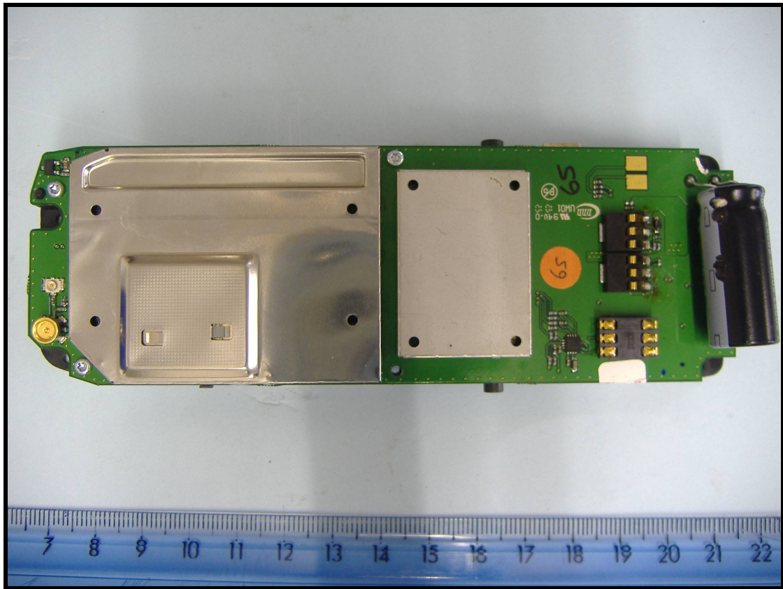
RF PCB
