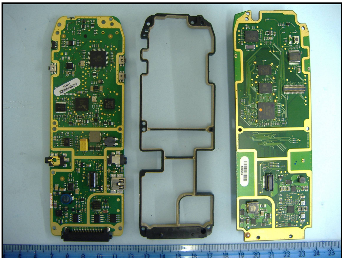
PCBs Overview
