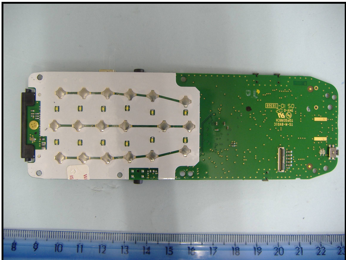
Control PCB Keypad/Display Side – Display Removed
