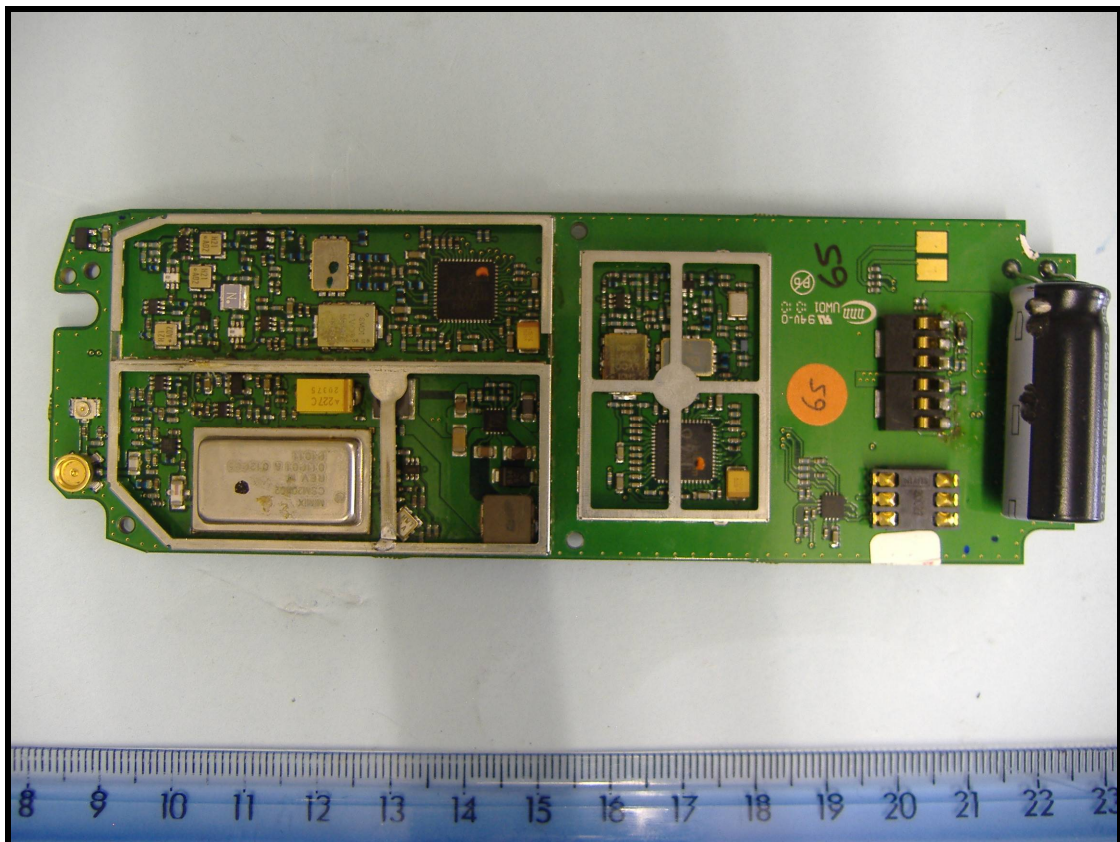
RF PCB Cans Removed
