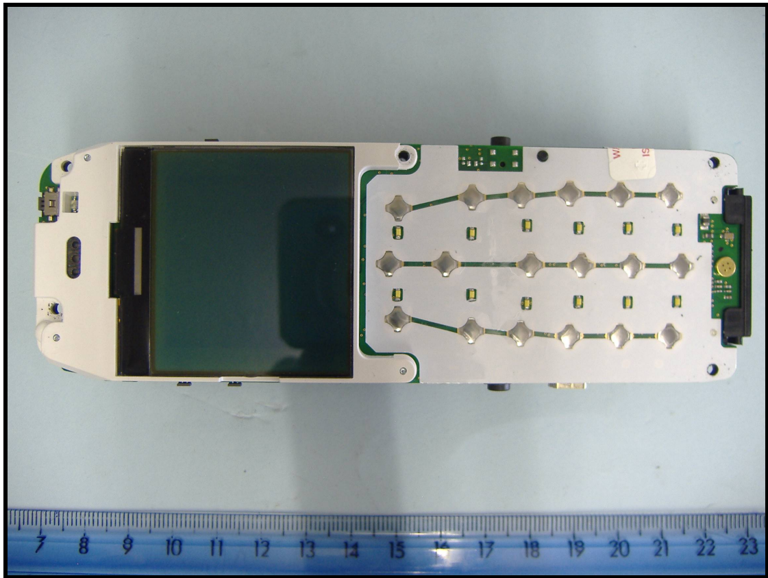
Control PCB Keypad/Display Side
