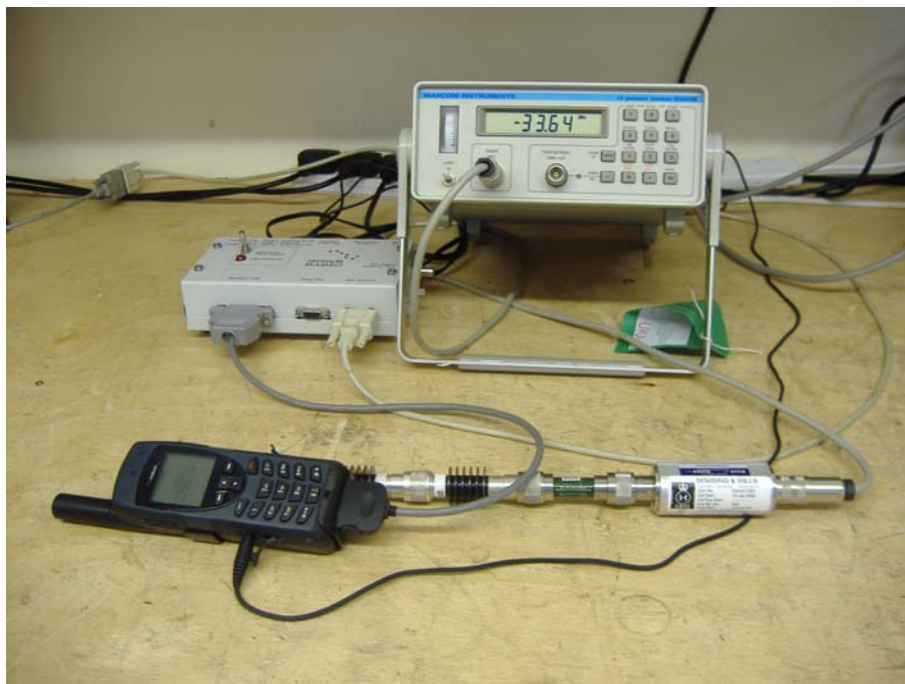
Conducted Output Power Test Setup
