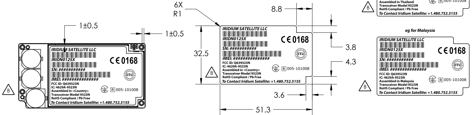
LABEL PLACEMENT
