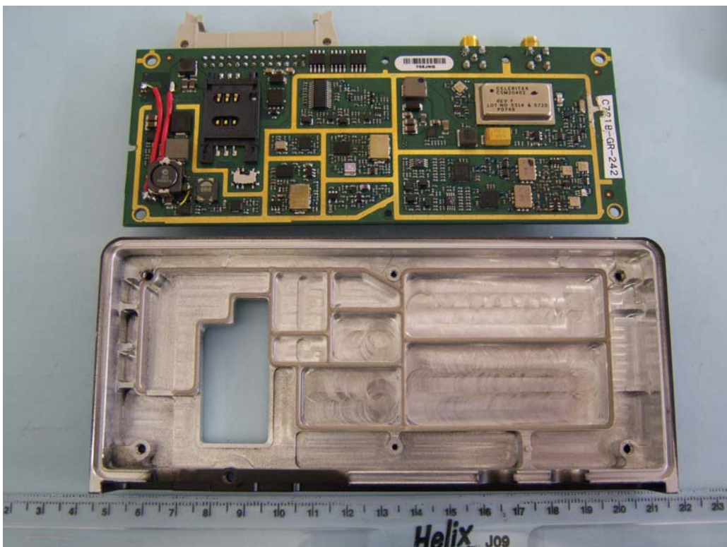
RF Side & Case
