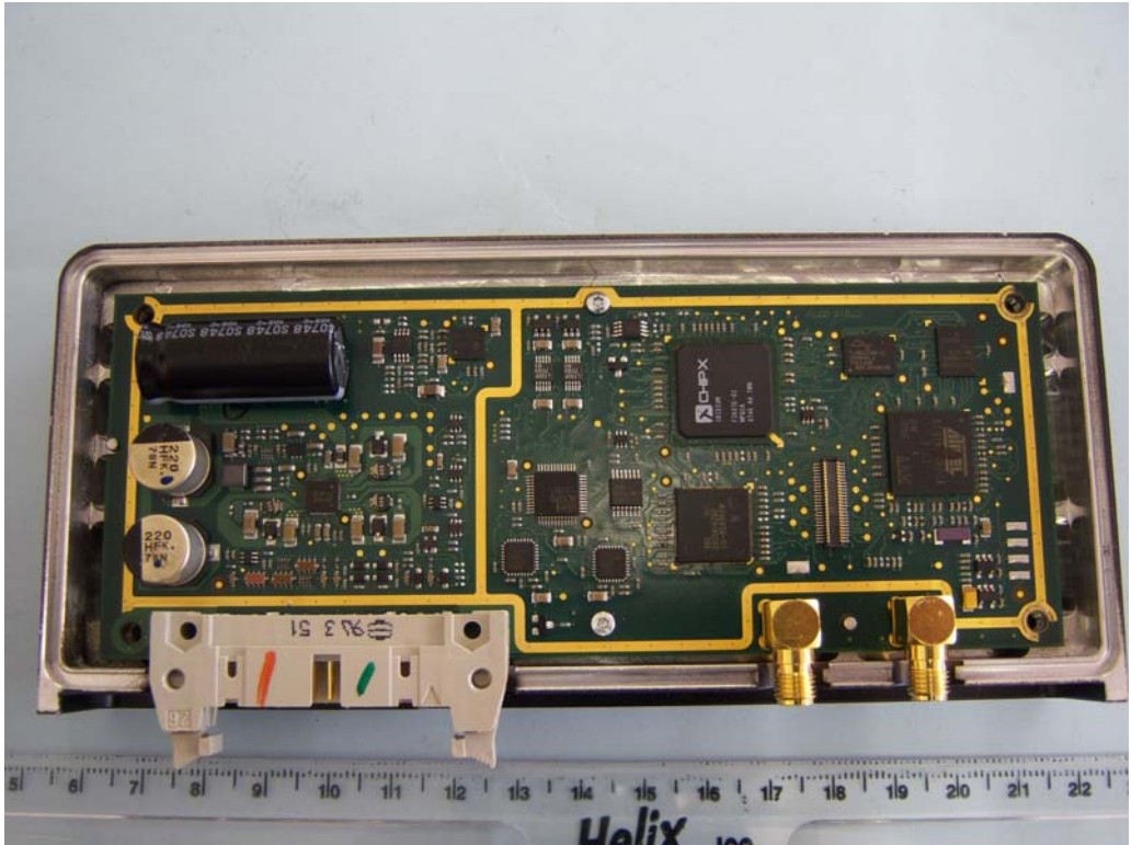
PCB Mounted In Case
