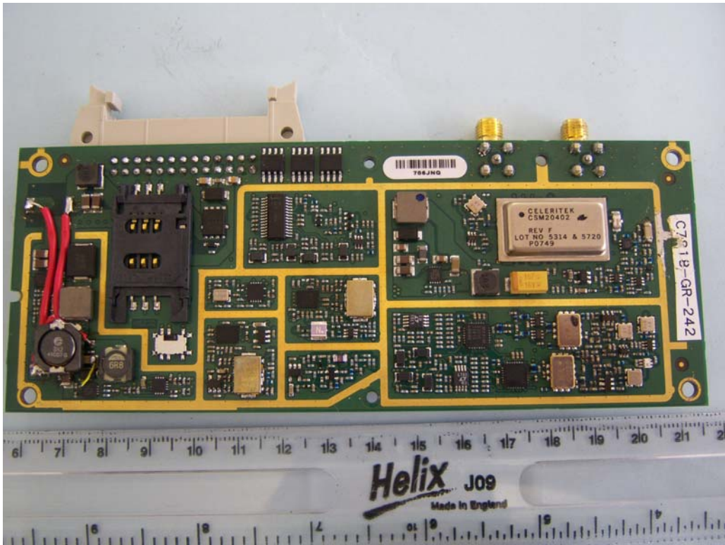
PCB RF Side
