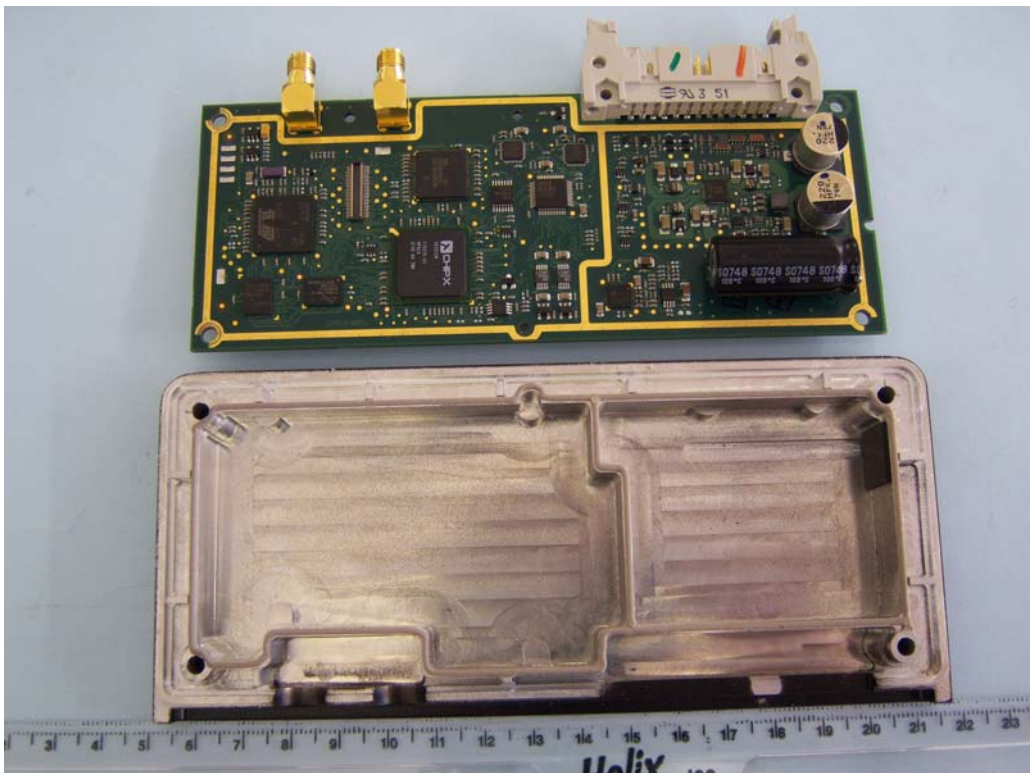
PCB, Processor Side & Case
