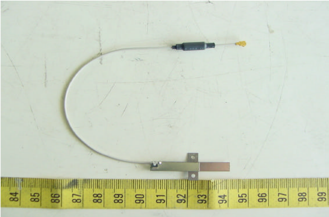
Antenna 2
