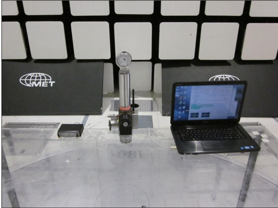
Photograph 1. Radiated Emission, Test Setup, Front
