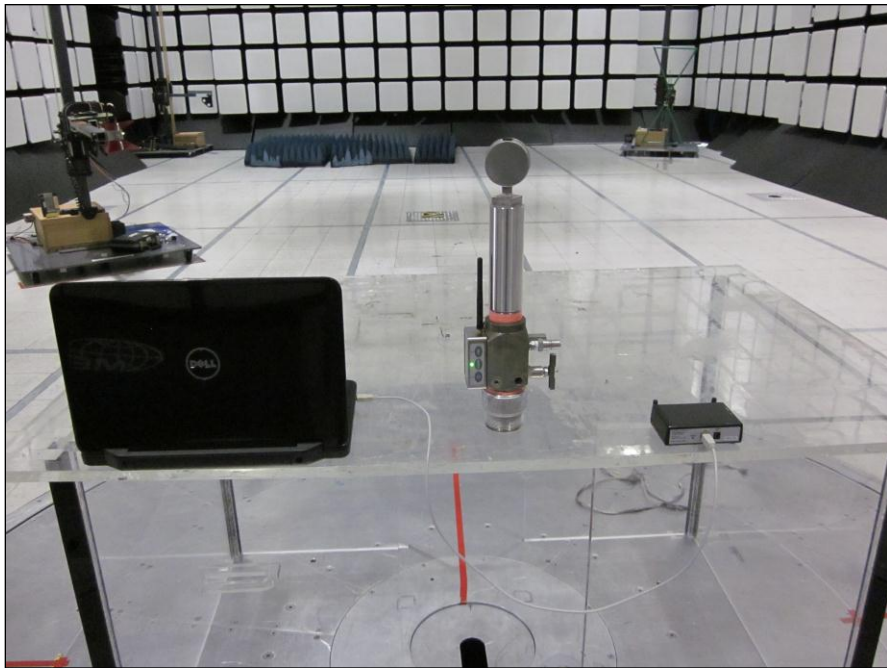
Photograph 2. Radiated Emission, Test Setup, Rear
