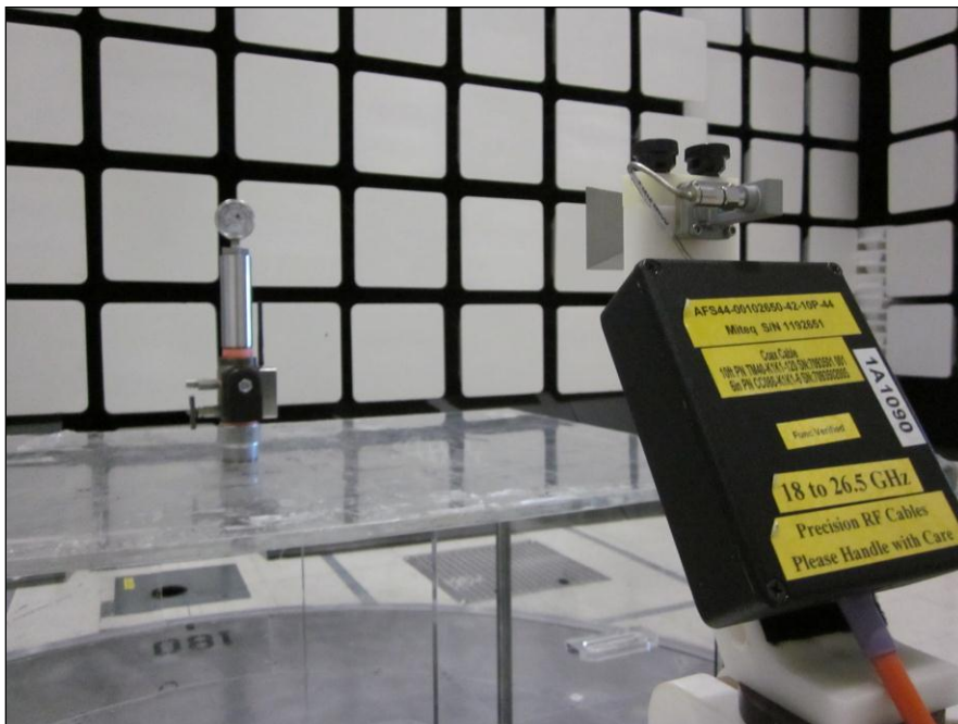
Photograph 6. Radiated Spurious Emissions, Test Setup, 18 GHz – 26.5 GHz
