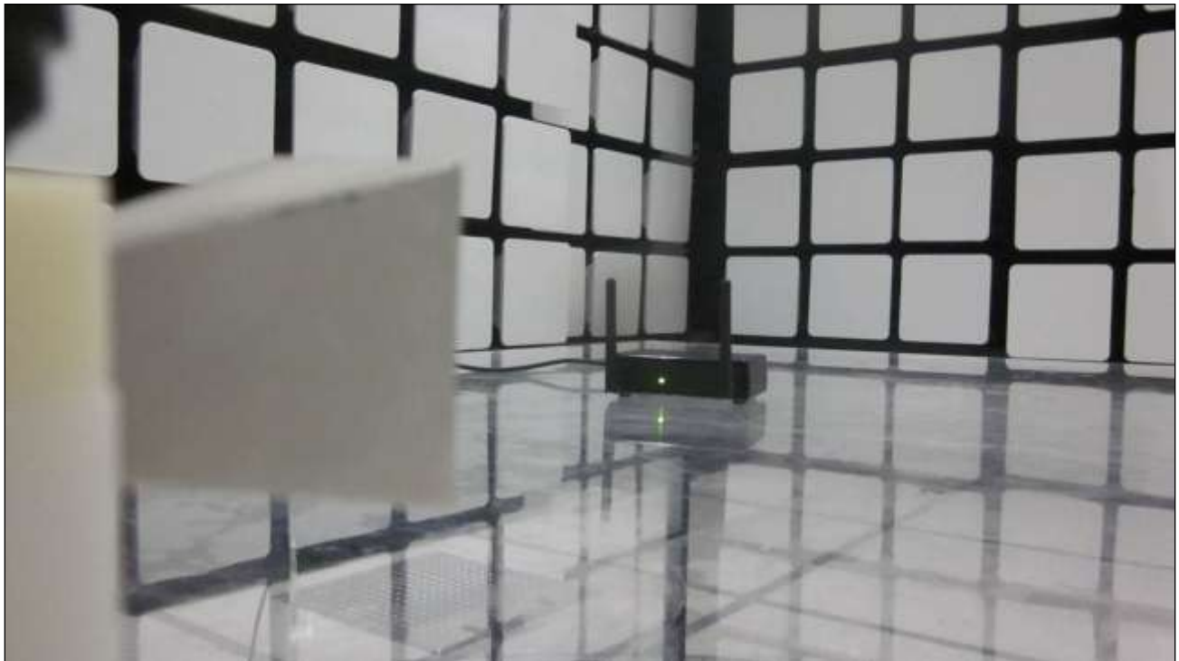
Photograph 4. Radiated Spurious Emissions, Test Setup, 18 GHz – 26 GHz
