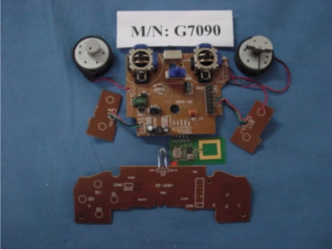
Figure 15 Main Board, Component Side
