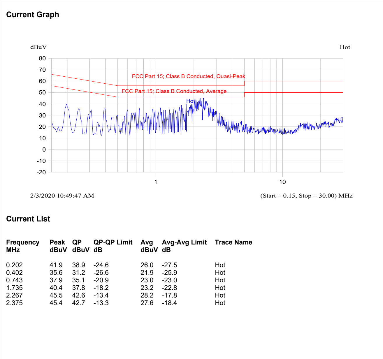
Plot 5.7.5.1. Power Line Conducted Emission, Tx Mode Line Voltage: AC 120 V; Line Tested: Line
