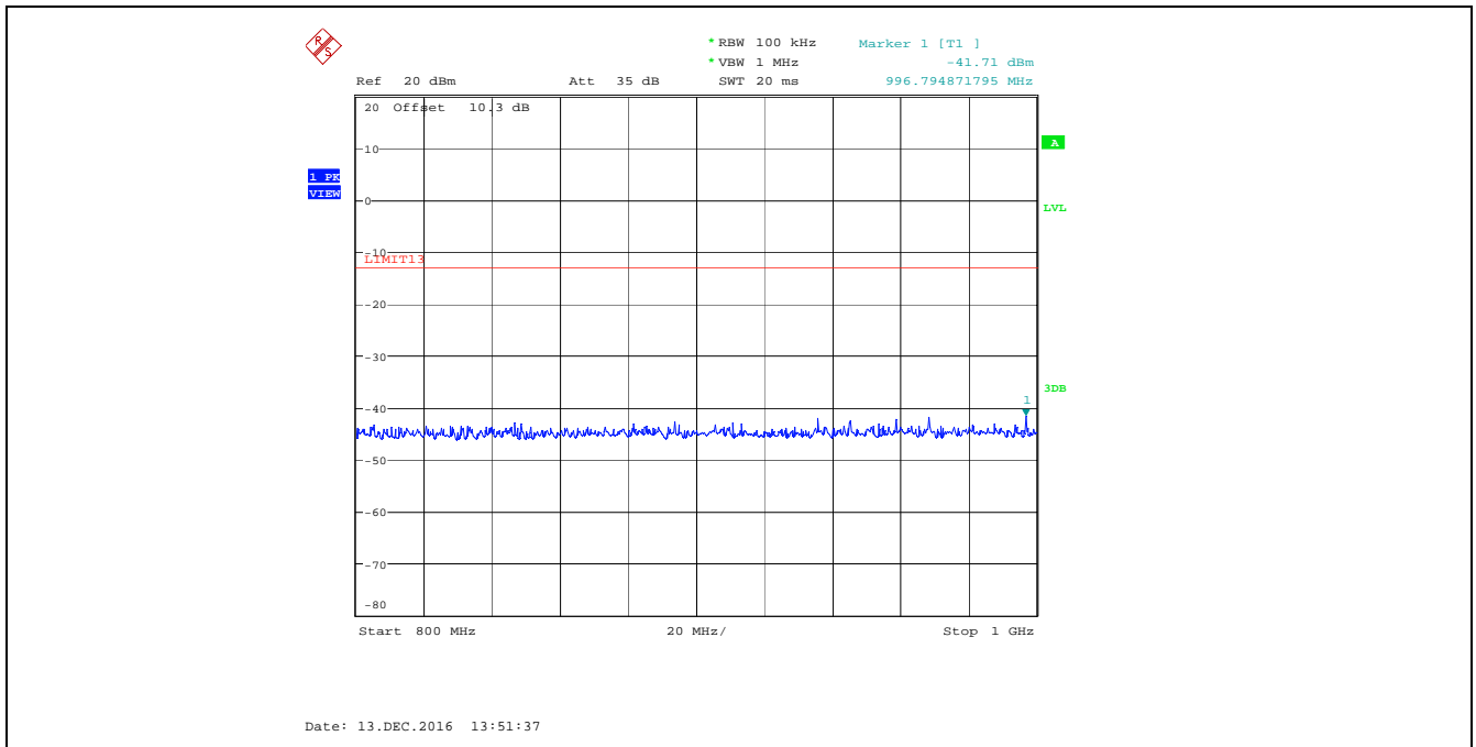
Plot 5.5.4.14. Spurious Emissions at Antenna Terminal, 550.000 MHz, High Power, Audio Input 15 kHz 1 Vrms 800 MHz - 1 GHz
