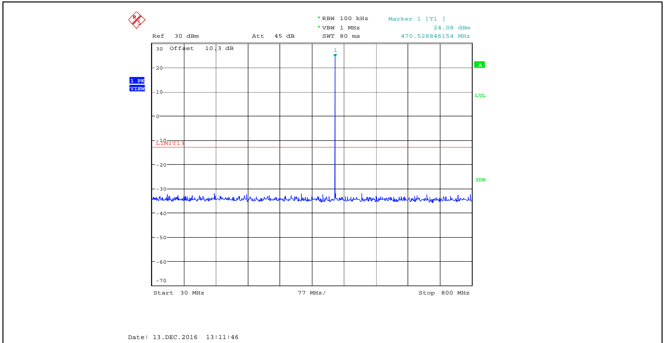
Plot 5.5.4.1. Spurious Emissions at Antenna Terminal, 470.250 MHz, High Power, Audio Input 15 kHz 1 Vrms 30 MHz - 800 MHz
