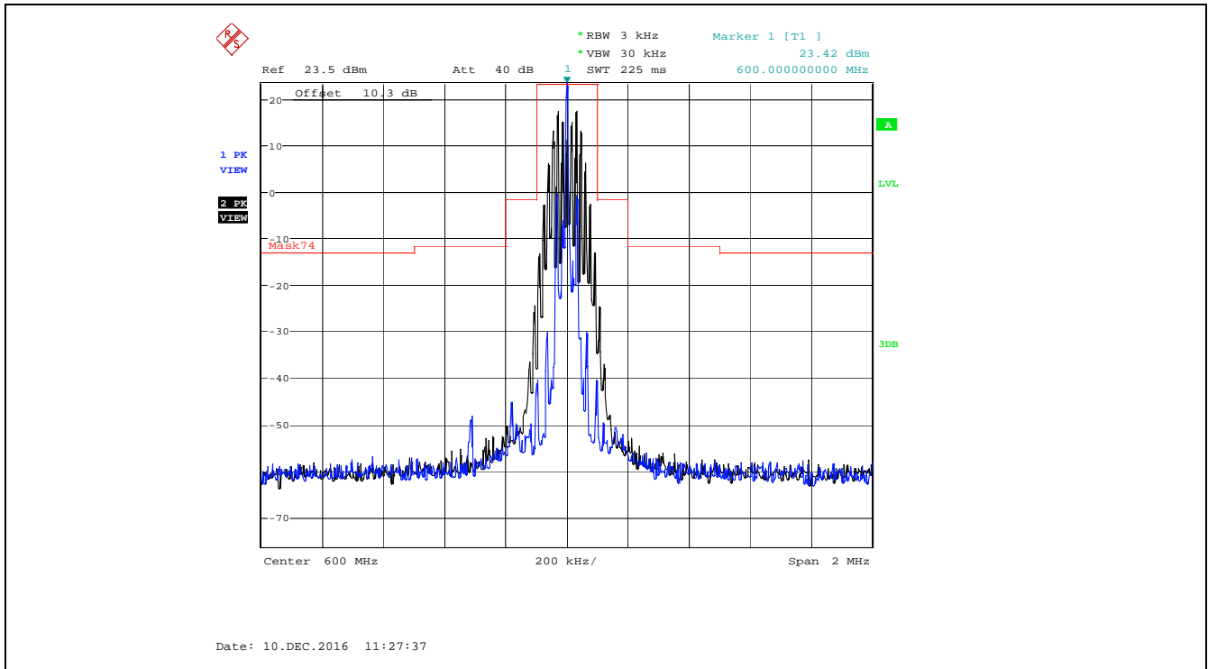
Plot 5.4.4.2.5. Emission Mask of §74.861(e)(6), 600.0 MHz, High Power, Audio input 15 kHz 1 Vrms
