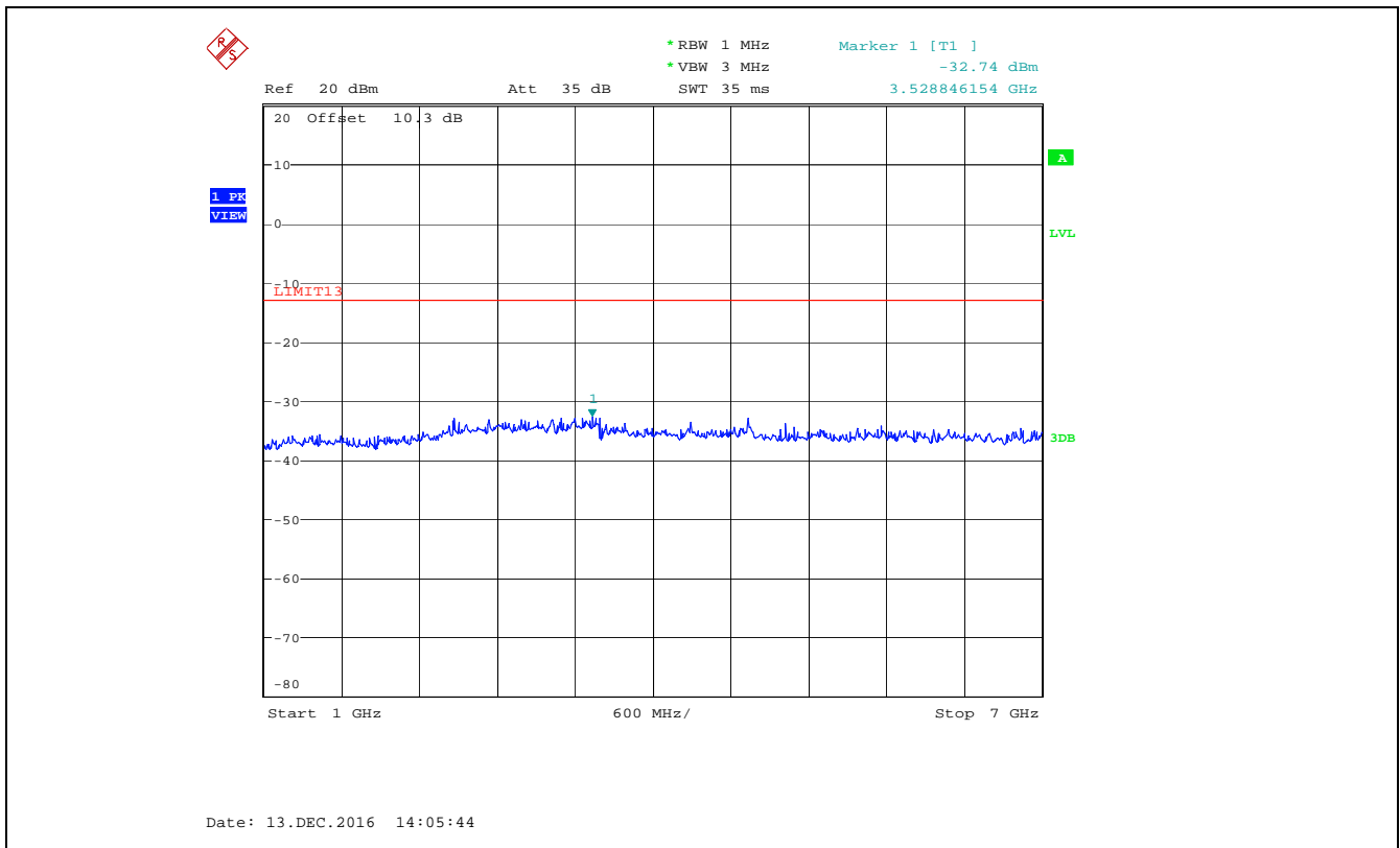
Plot 5.5.4.6. Spurious Emissions at Antenna Terminal, 525.0 MHz, Low Power, Audio Input 15 kHz 1 Vrms 1 GHz - 7 GHz
