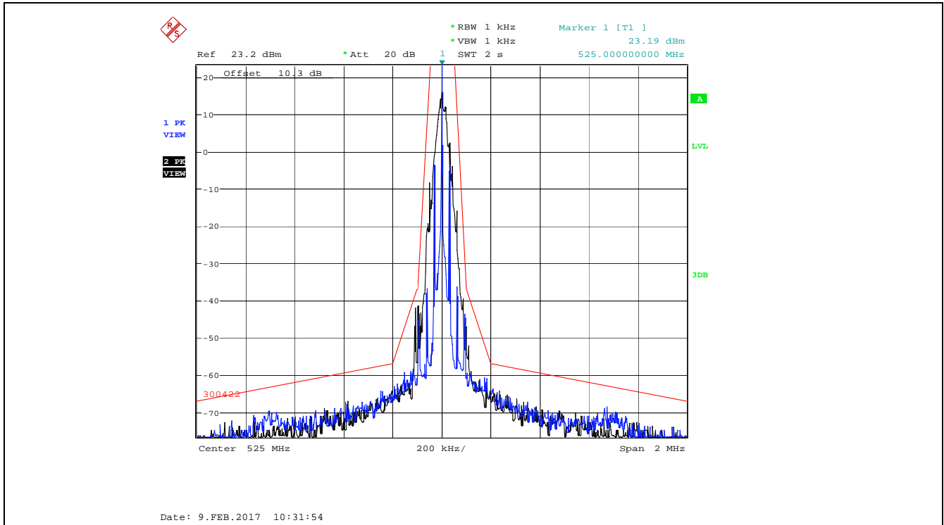
Plot 5.4.4.3.1. Emission Mask of §74.861(e)(7), 525.0 MHz, High Power Audio input maximum 1 Vrms, Noise source input level 1V band limit to 15 kHz
