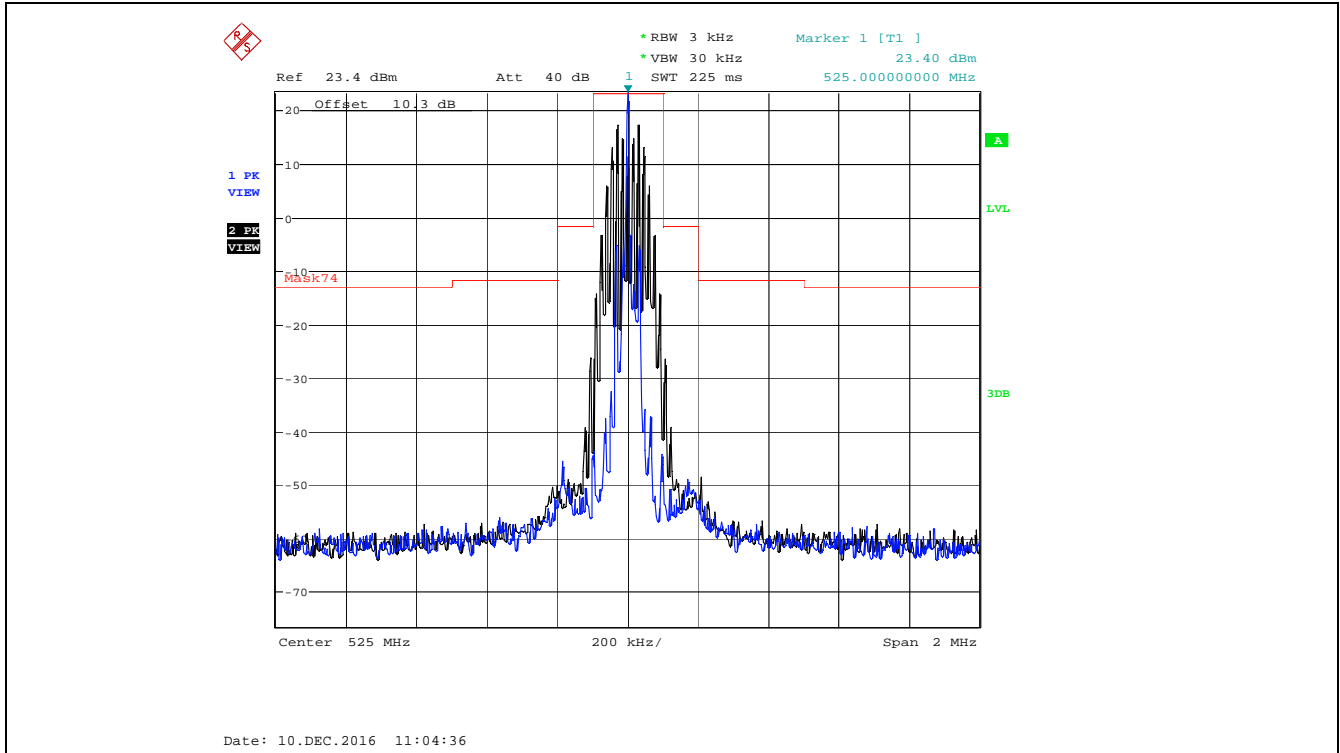
Plot 5.4.4.2.1. Emission Mask of §74.861(e)(6), 525.0 MHz, High Power, Audio input 15 kHz 1 Vrms
