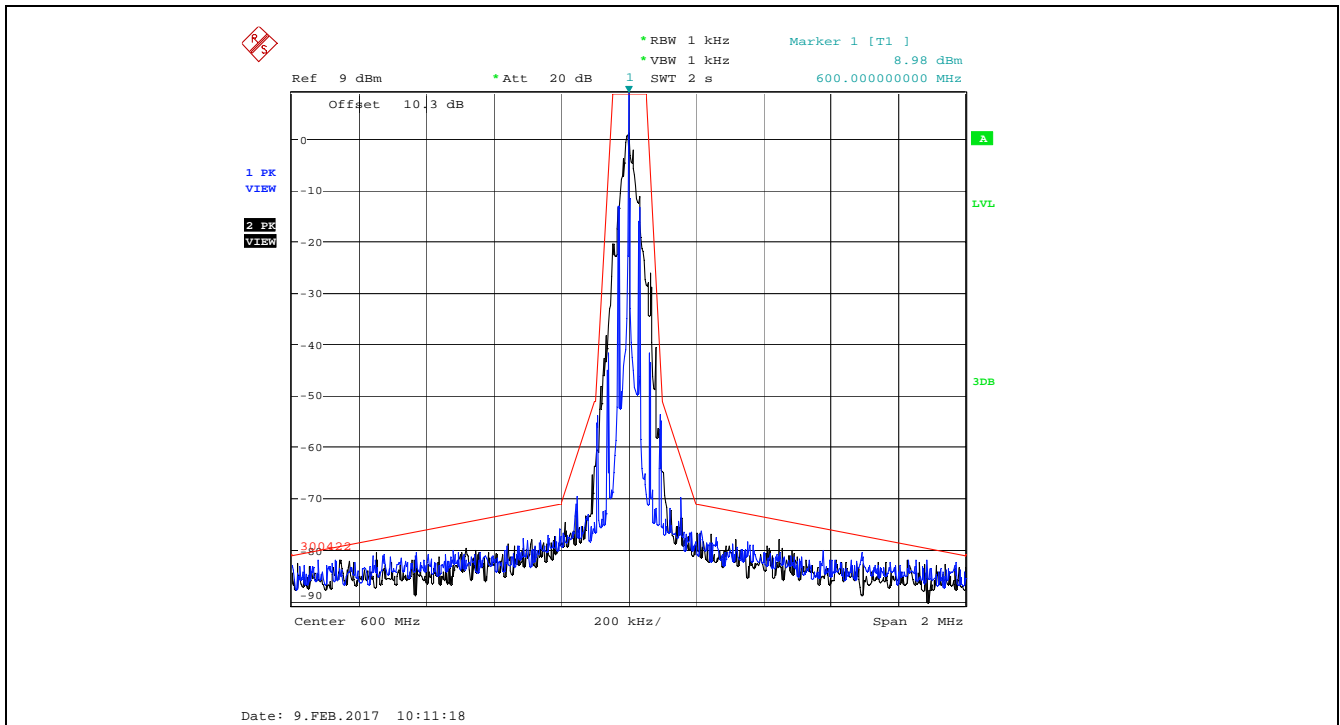
Plot 5.4.4.3.6. Emission Mask of §74.861(e)(7), 600.0 MHz, Low Power Audio input maximum 1 Vrms, Noise source input level 1V band limit to 15 kHz
