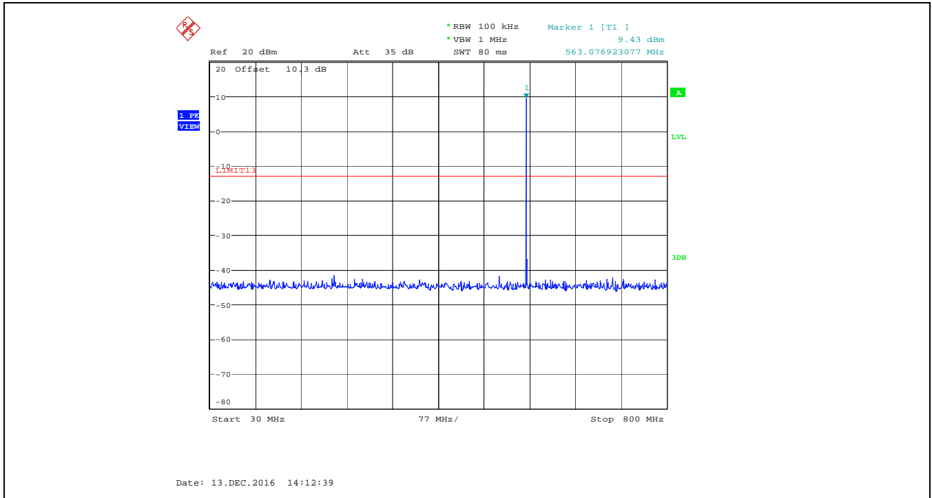
Plot 5.5.4.10. Spurious Emissions at Antenna Terminal, 563.0 MHz, Low Power, Audio Input 15 kHz 1 Vrms 30 MHz - 800 MHz
