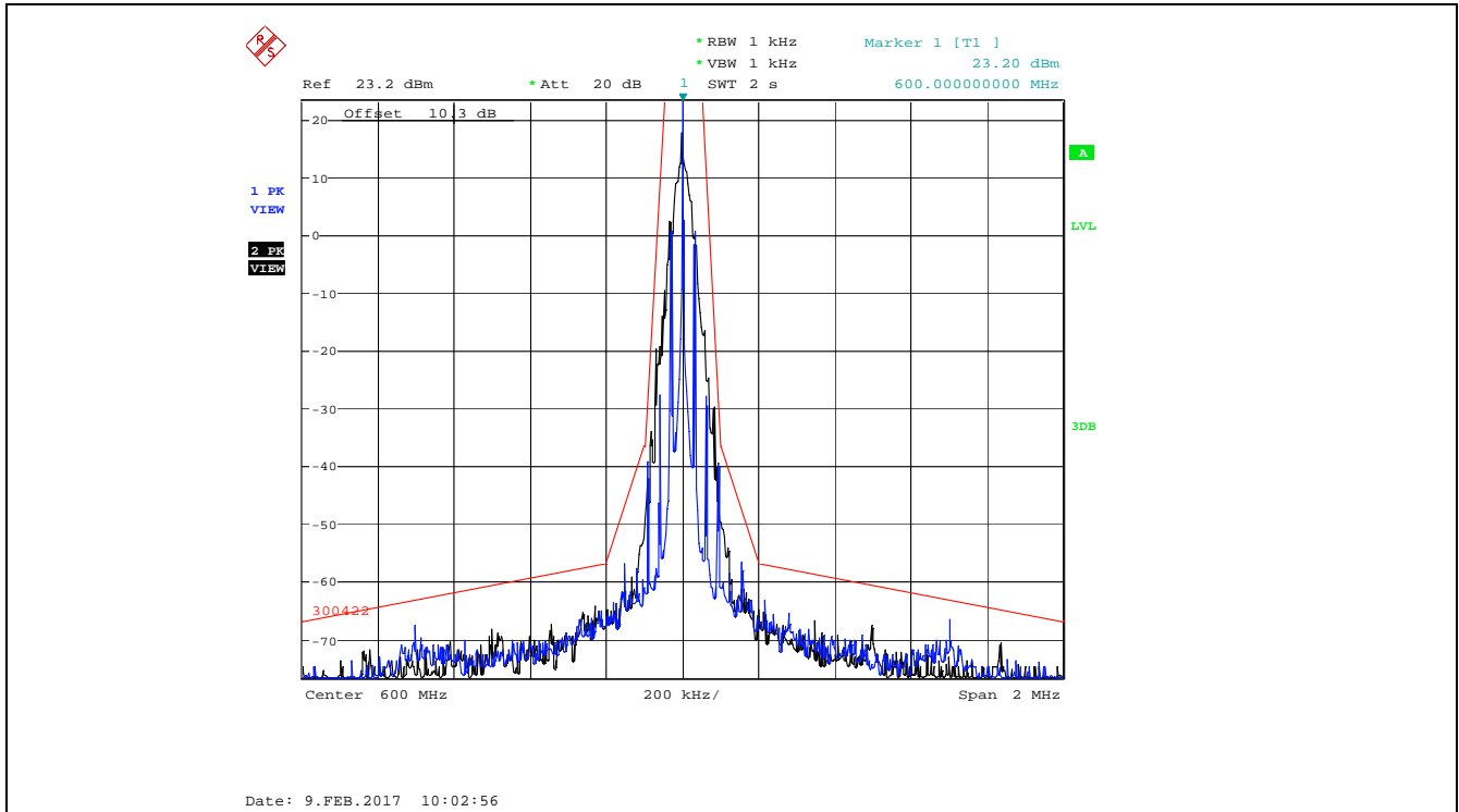
Plot 5.4.4.3.5. Emission Mask of §74.861(e)(7), 600.0 MHz, High Power Audio input maximum 1 Vrms, Noise source input level 1V band limit to 15 kHz
