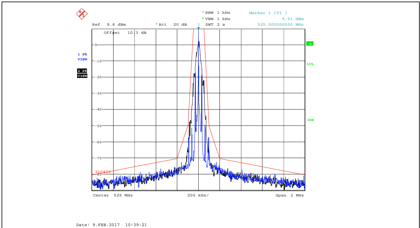
Plot 5.4.4.3.2. Emission Mask of §74.861(e)(7), 525.0 MHz, Low Power Audio input maximum 1 Vrms, Noise source input level 1V band limit to 15 kHz
