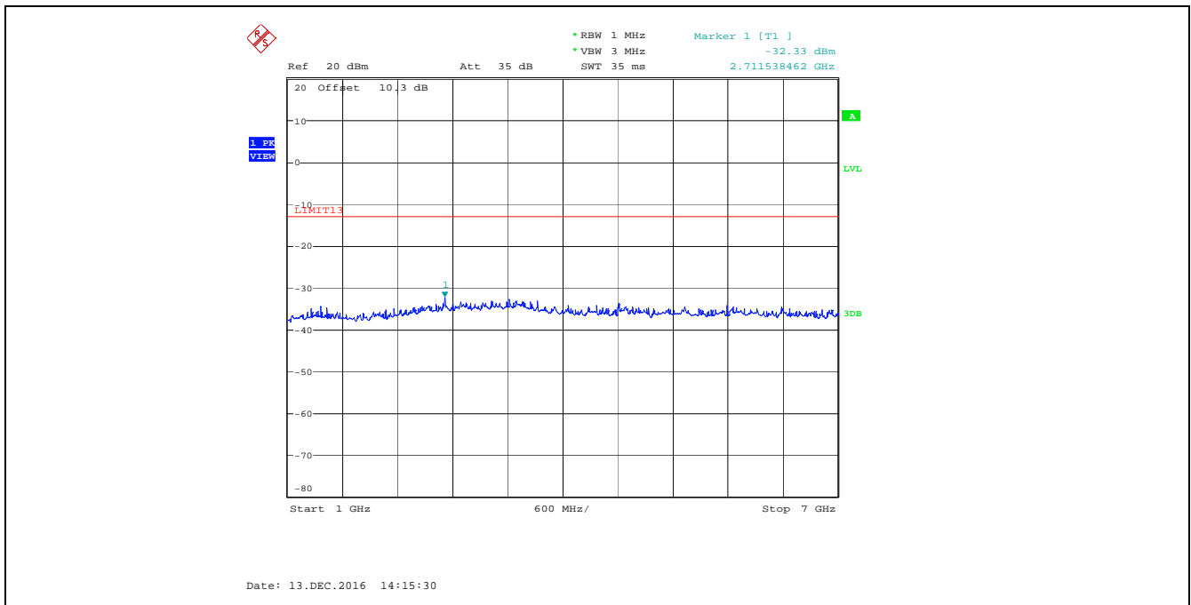
Plot 5.5.4.12. Spurious Emissions at Antenna Terminal, 563.0 MHz, Low Power, Audio Input 15 kHz 1 Vrms 1 GHz - 7 GHz
