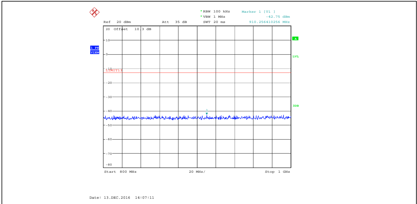
Plot 5.5.4.5. Spurious Emissions at Antenna Terminal, 525.0 MHz, Low Power, Audio Input 15 kHz 1 Vrms 800 MHz - 1 GHz
