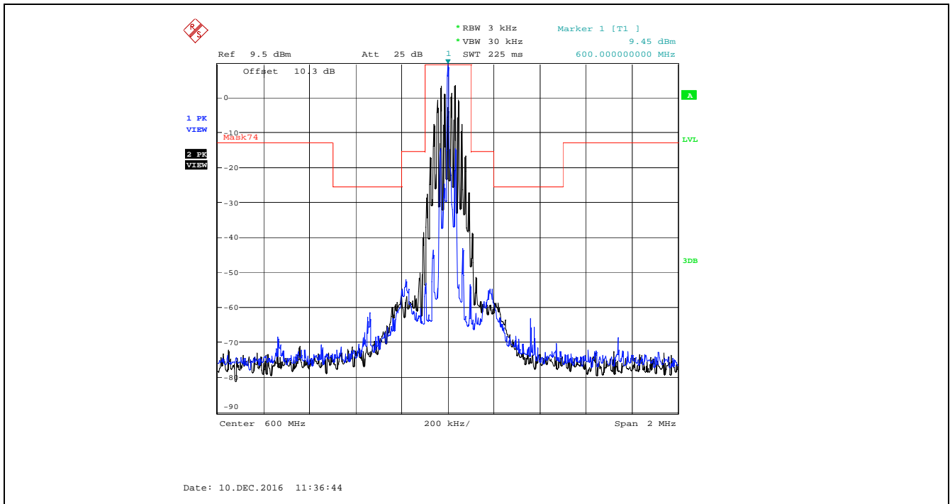
Plot 5.4.4.2.6. Emission Mask of §74.861(e)(6), 600.0 MHz, Low Power, Audio input 15 kHz 1 Vrms
