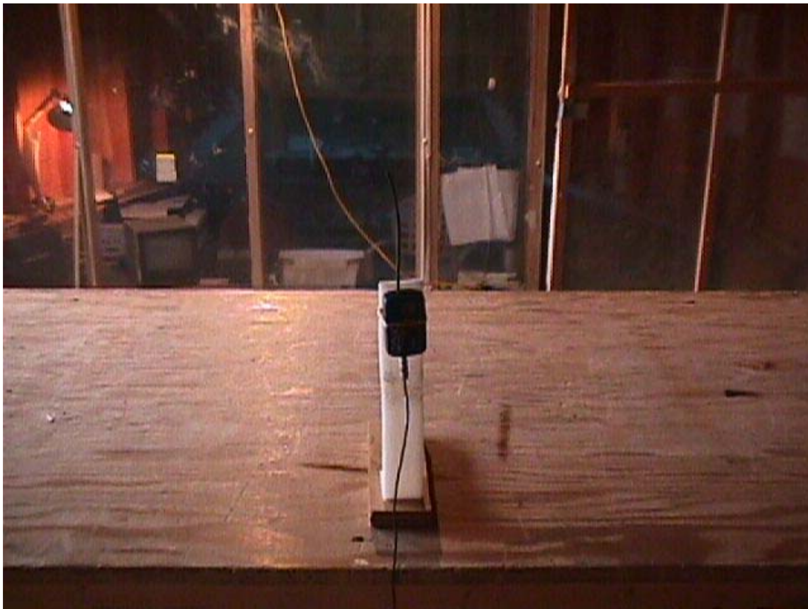
Radiated Emissions at 3 Meters – Orthogonal Position #3
