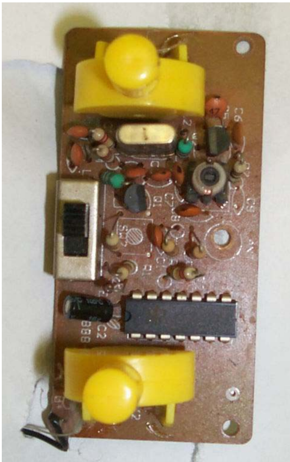
Component Side
