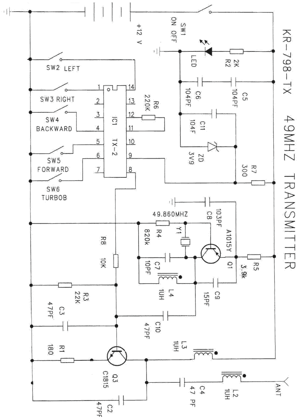
Figure 4.1 System Schematics
