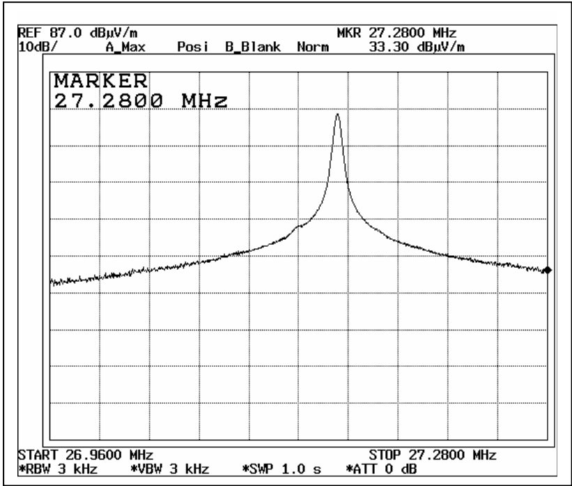
Bandwidth Plot
