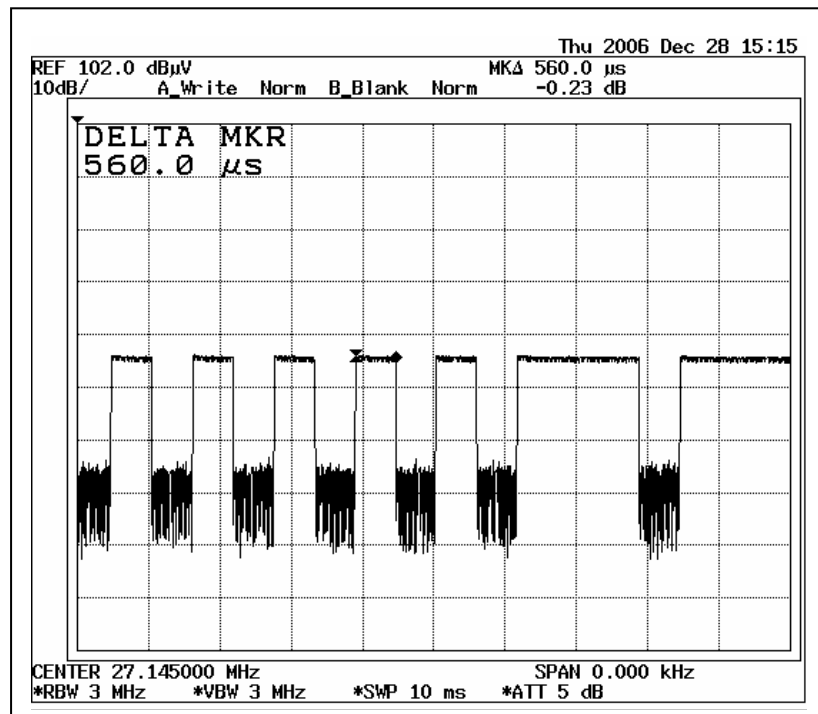
Duty Cycle 3
