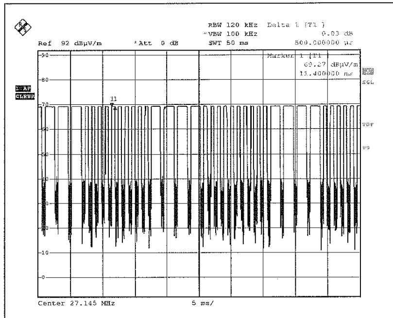
Duty Cycle 3
