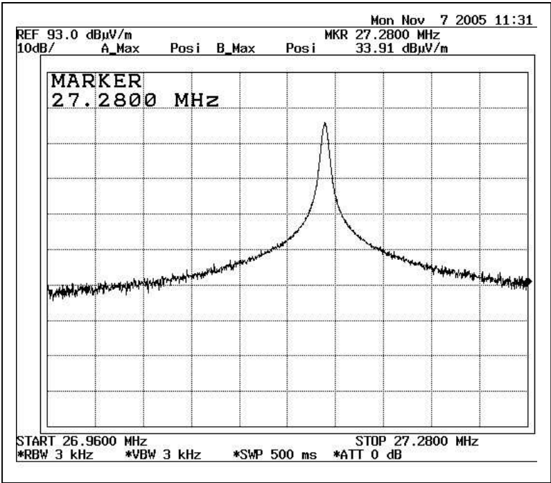
Bandwidth Plot
