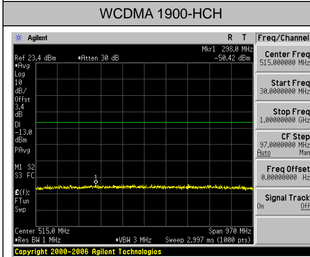
WCDMA 1900-HCH
