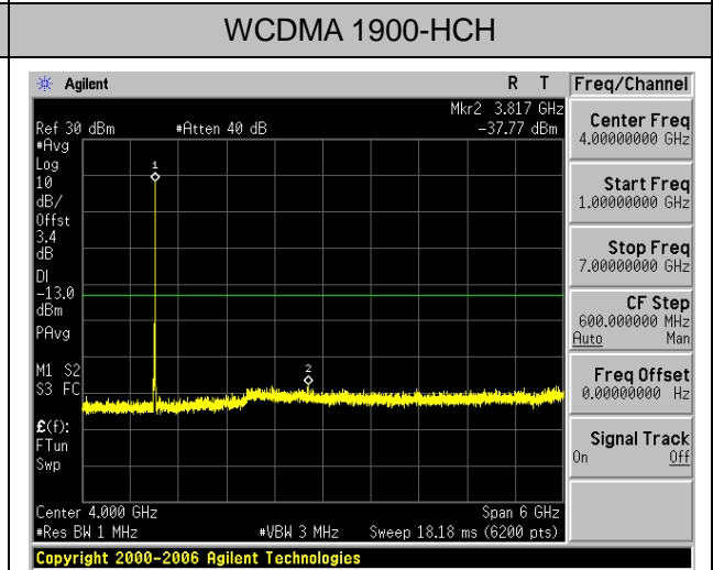
WCDMA 1900-HCH
