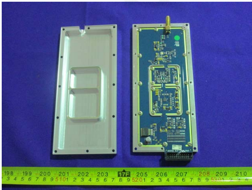
EUT – Receiver Box Uncover View
