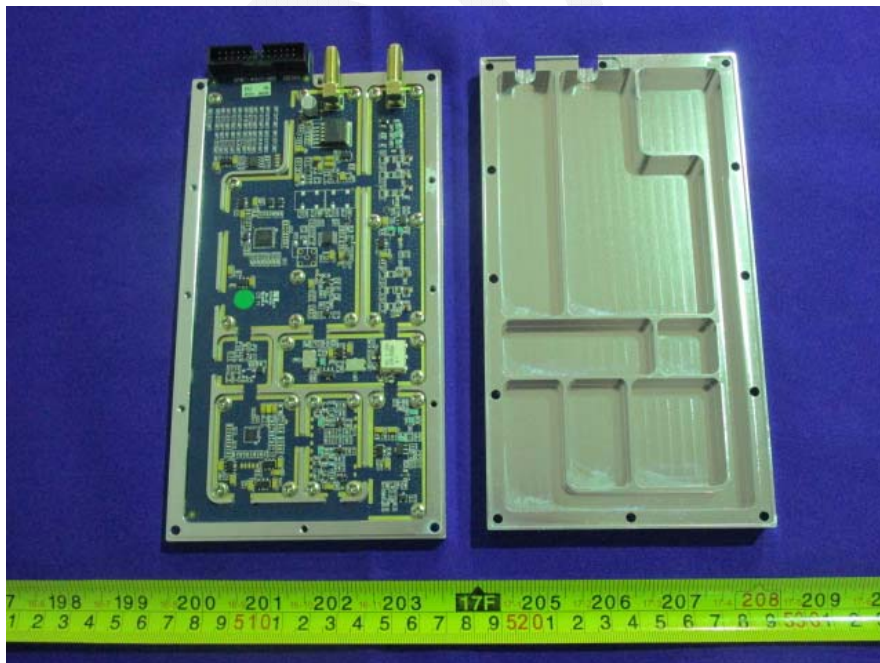
EUT – Transmitter Box Uncover View
