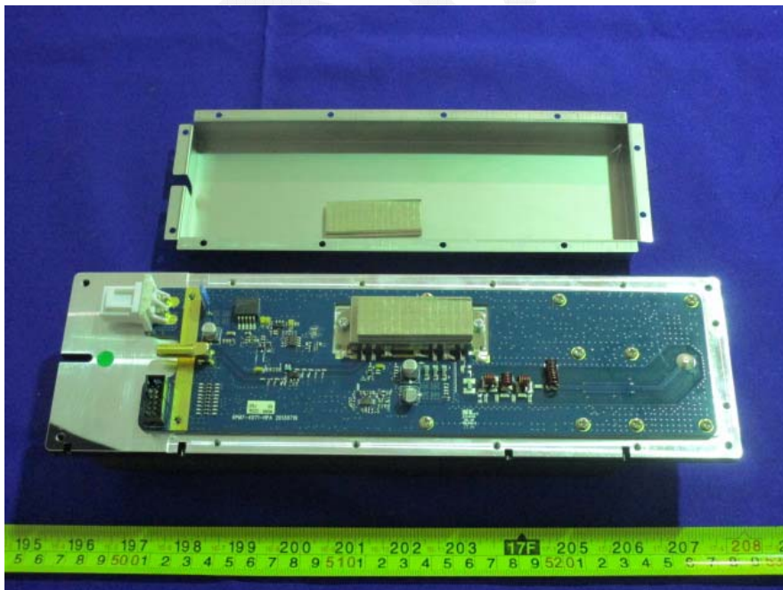
EUT – RF Box Uncover View
