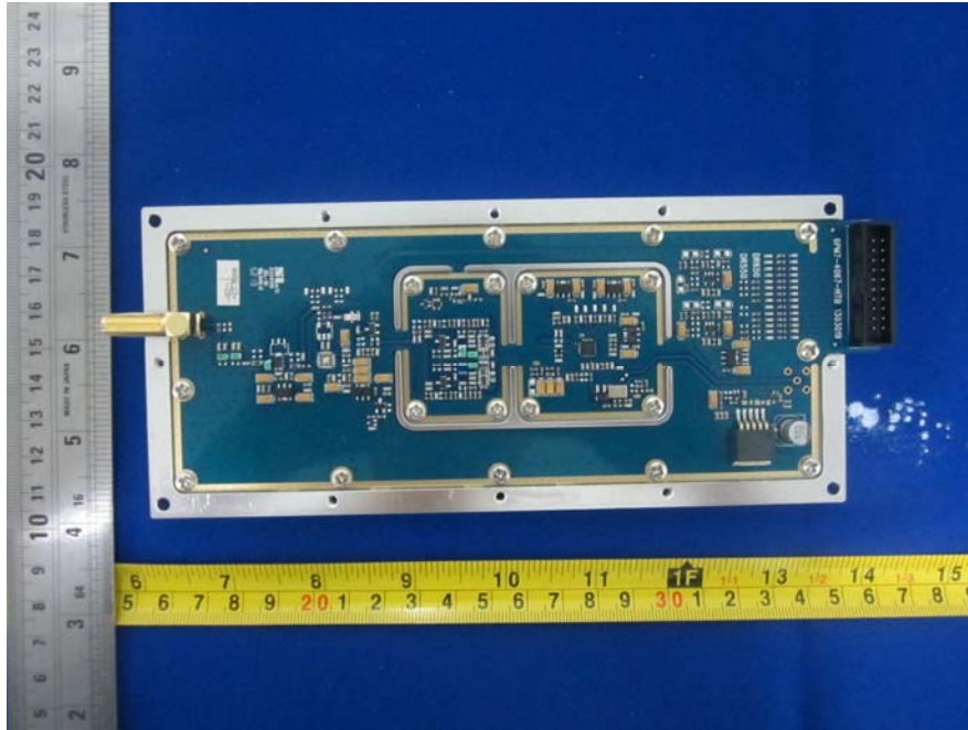
EUT – Transmit Board Top View
