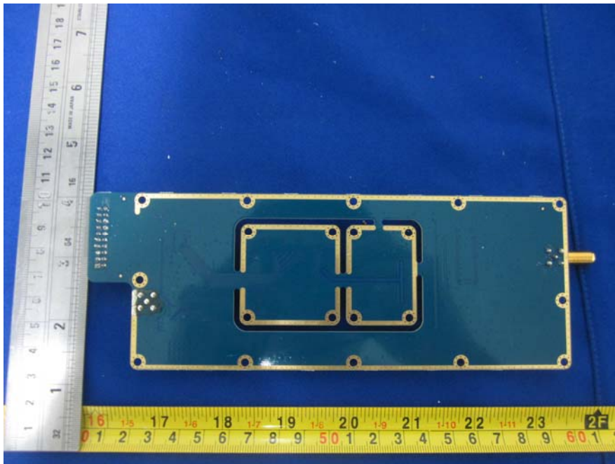
EUT – Transmit Board Bottom View
