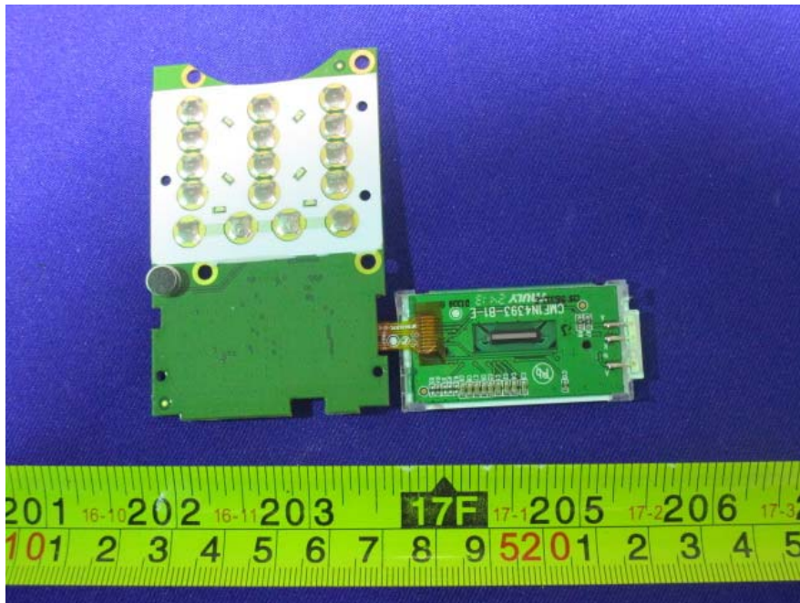
EUT – Sub Board Top LCD Uncover View
