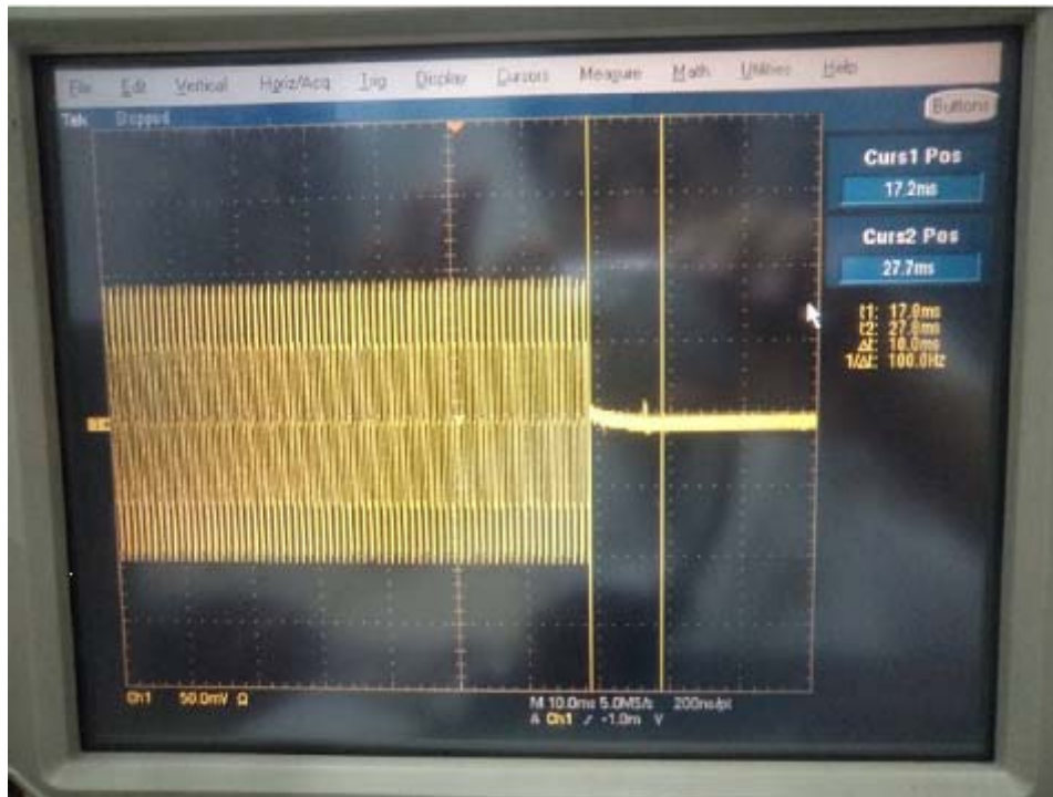
Transmitter Frequency Behaviour @ 12.5 KHz Channel Separation--On to Off
