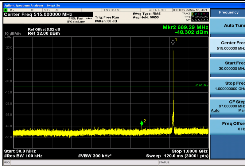
Band26-3MHz-16QAM-26805-1RB#0-30~1000MHz
