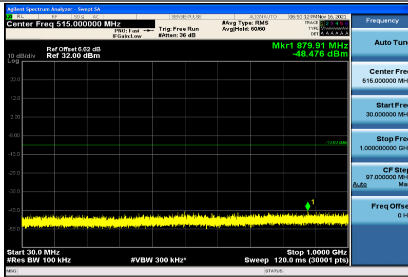
Band25-5MHz-QPSK-26065-1RB#0-30~1000MHz
