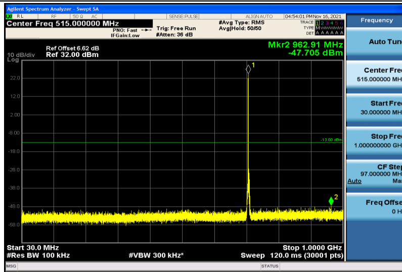
Band12-3MHz-16QAM-23165-1RB#0-30~1000MHz
