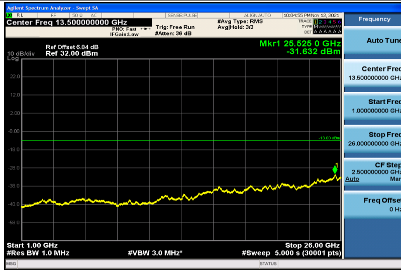
Band5-5MHz-16QAM-20525-1RB#0-1000~26000MHz
