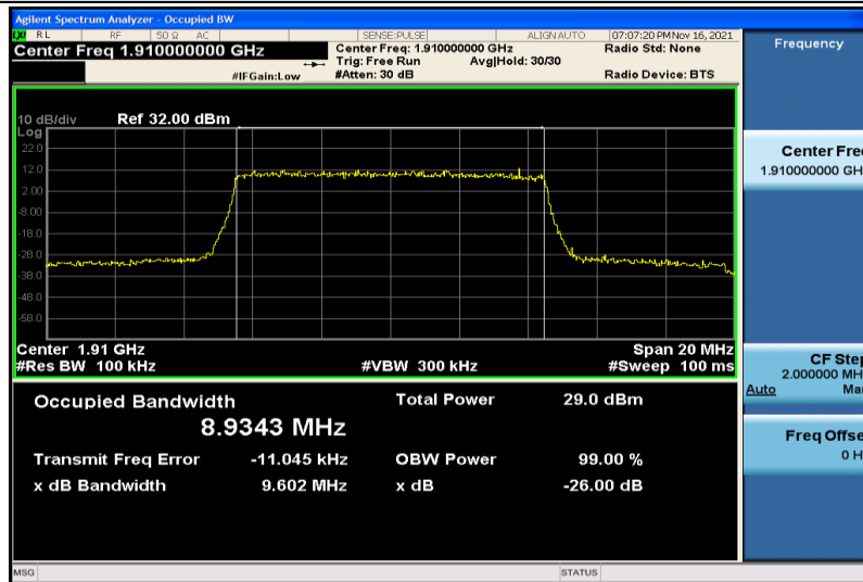
Band25-10MHz-16QAM-26640-50RB#0-8.9343
