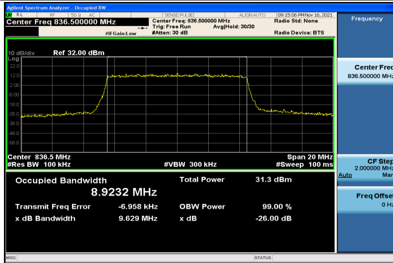
Band26-10MHz-QPSK-26915-50RB#0-8.9232
