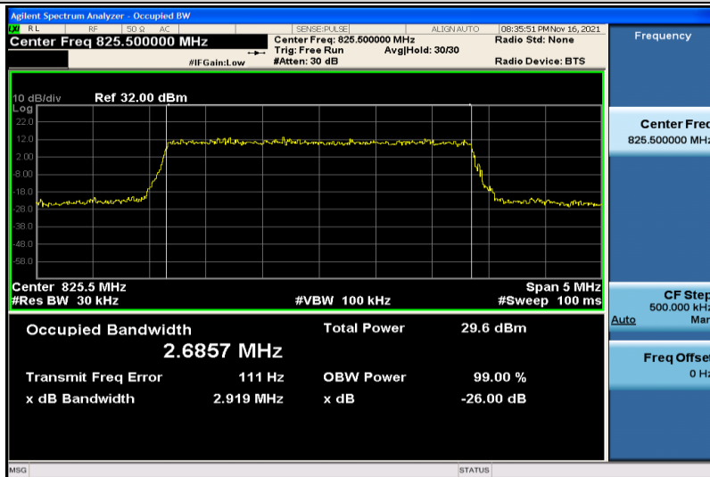
Band26-3MHz-16QAM-26805-15RB#0-2.6857
