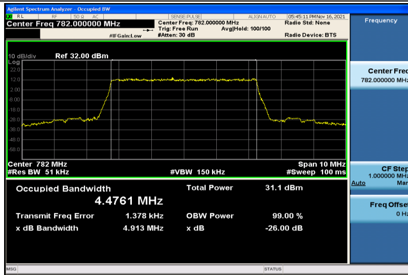
Band13-5MHz-QPSK-23230-25RB#0-4.4761
