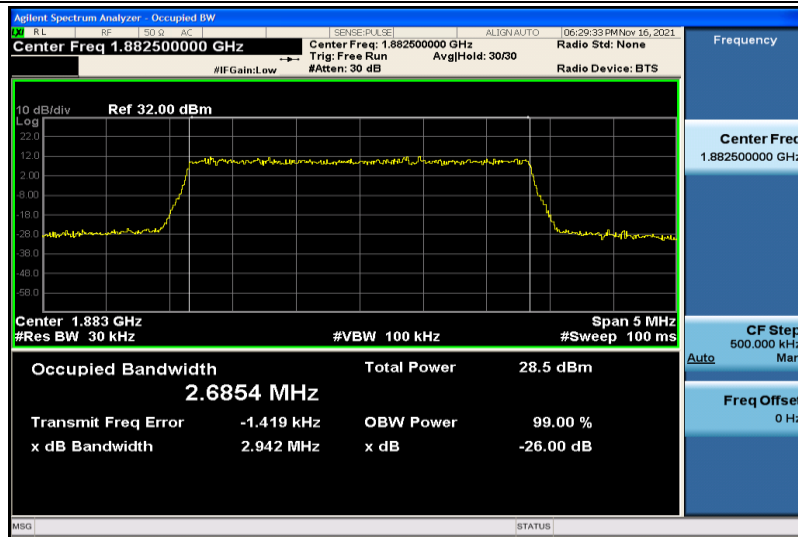
Band25-3MHz-16QAM-26365-15RB#0-2.6854
