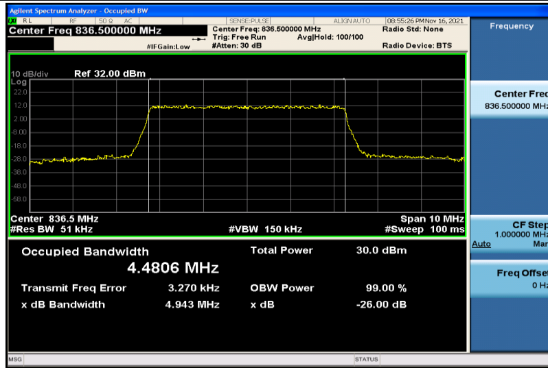
Band26-5MHz-16QAM-26915-25RB#0-4.4806
