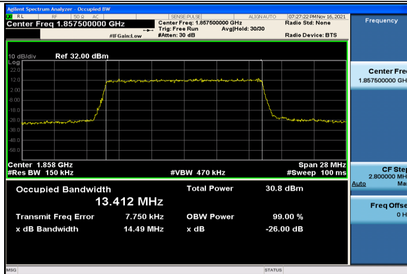
Band25-15MHz-QPSK-26115-75RB#0-13.412
