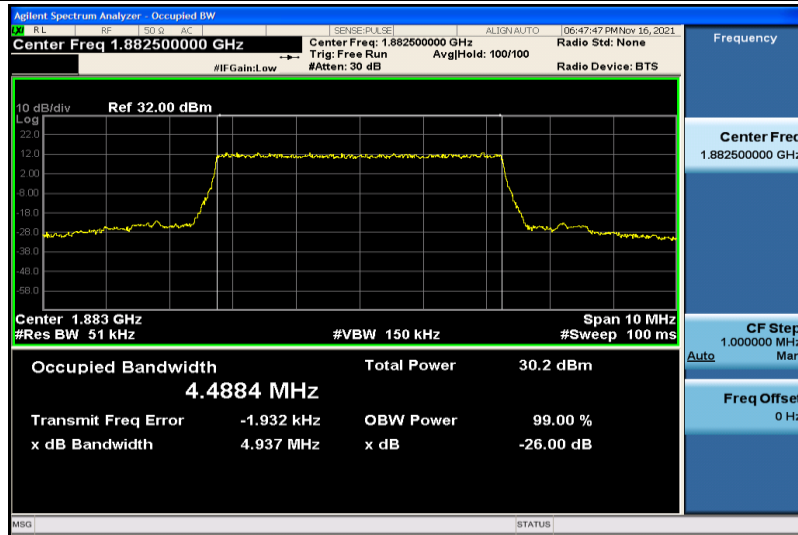
Band25-5MHz-QPSK-26365-25RB#0-4.4884
