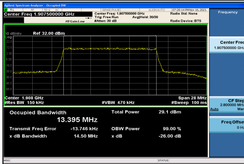
Band25-15MHz-16QAM-26615-75RB#0-13.395
