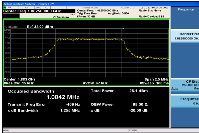
Band25-1.4MHz-16QAM-26365-6RB#0-1.0842
