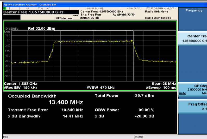
Band25-15MHz-16QAM-26115-75RB#0-13.400
