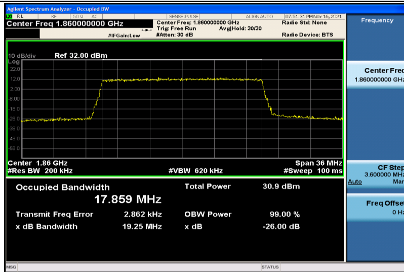
Band25-20MHz-QPSK-26140-100RB#0-17.859
