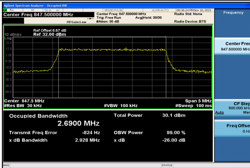
Band26-3MHz-QPSK-27025-15RB#0-2.6900
