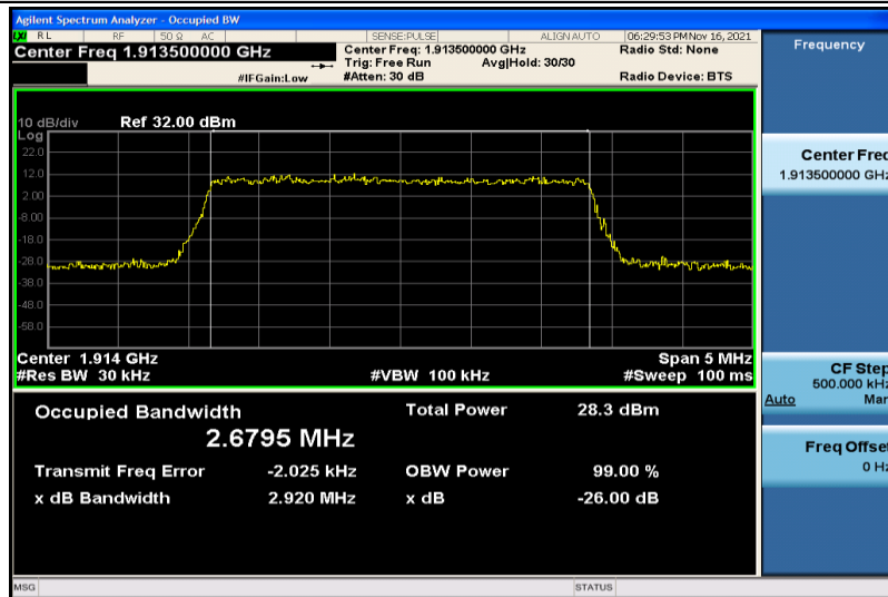
Band25-3MHz-16QAM-26675-15RB#0-2.6795
