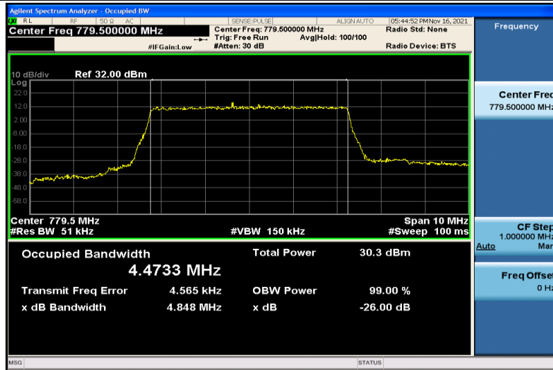
Band13-5MHz-16QAM-23205-25RB#0-4.4733
