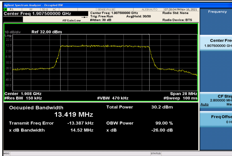
Band25-15MHz-QPSK-26615-75RB#0-13.419
