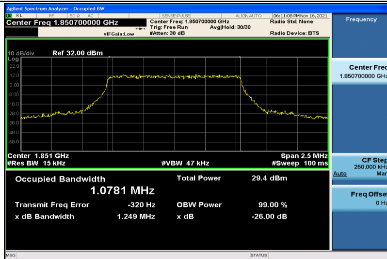
Band25-1.4MHz-QPSK-26047-6RB#0-1.0781
