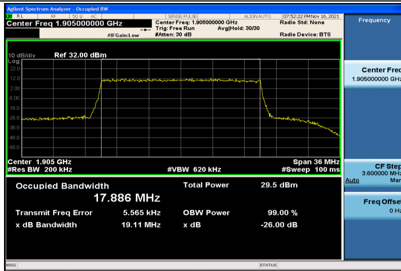
Band25-20MHz-16QAM-26590-100RB#0-17.886
