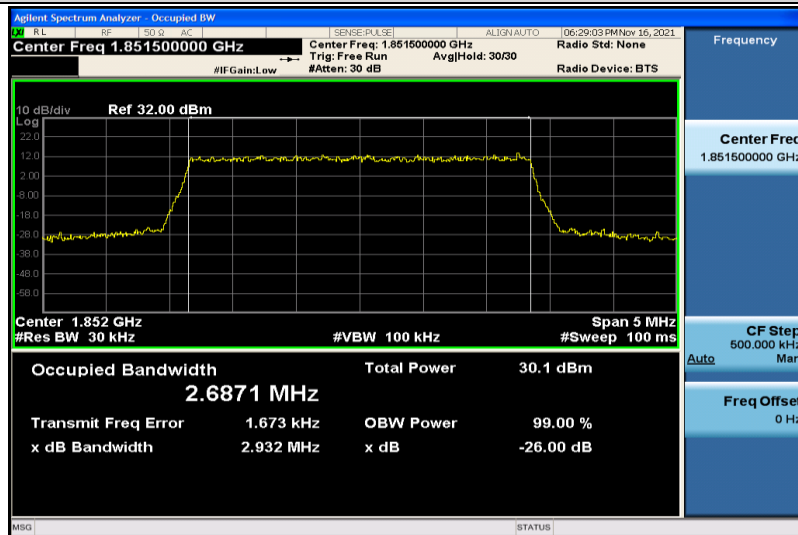
Band25-3MHz-QPSK-26055-15RB#0-2.6871
