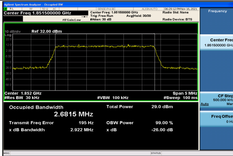
Band25-3MHz-16QAM-26055-15RB#0-2.6815
