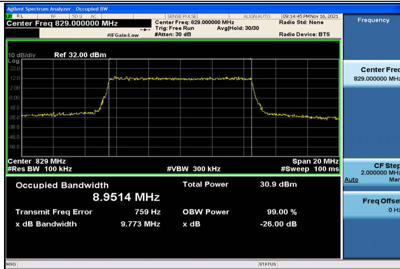
Band26-10MHz-QPSK-26840-50RB#0-8.9514
