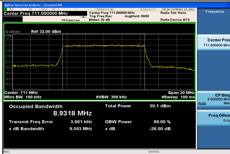
Band12-10MHz-16QAM-23130-50RB#0-8.9318
