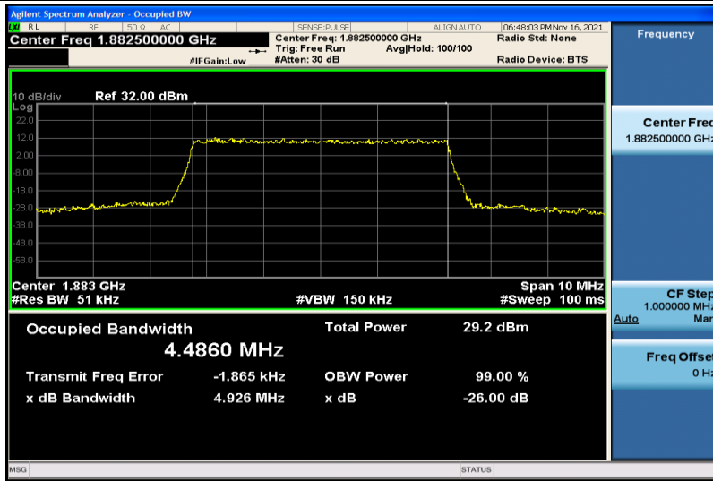
Band25-5MHz-16QAM-26365-25RB#0-4.4860
