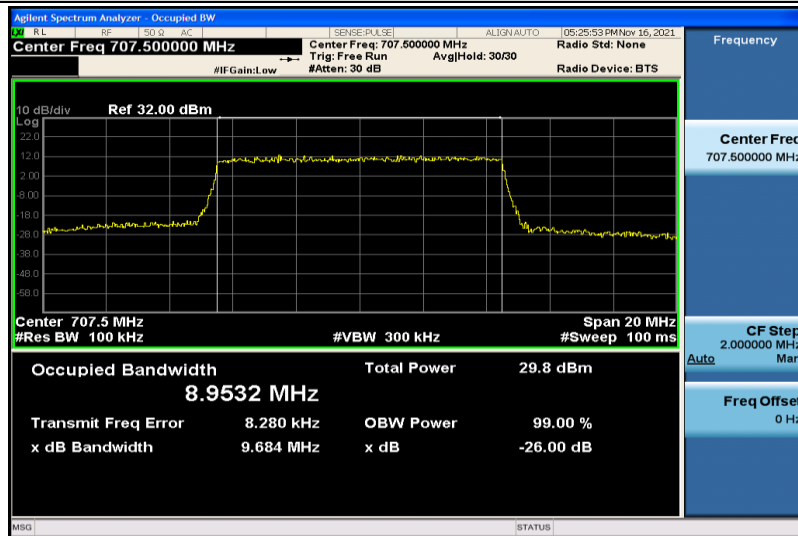
Band12-10MHz-16QAM-23095-50RB#0-8.9532
