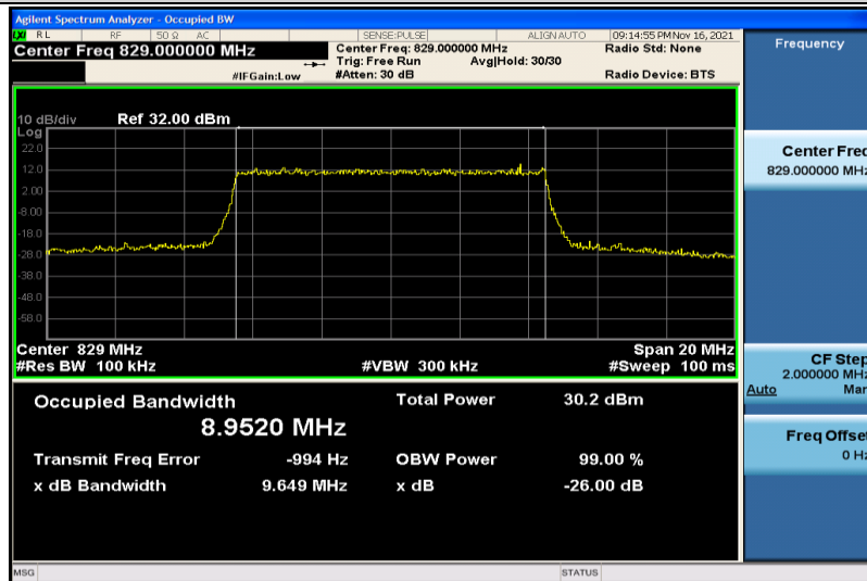
Band26-10MHz-16QAM-26840-50RB#0-8.9520
