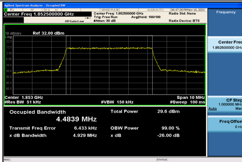
Band25-5MHz-16QAM-26065-25RB#0-4.4839
