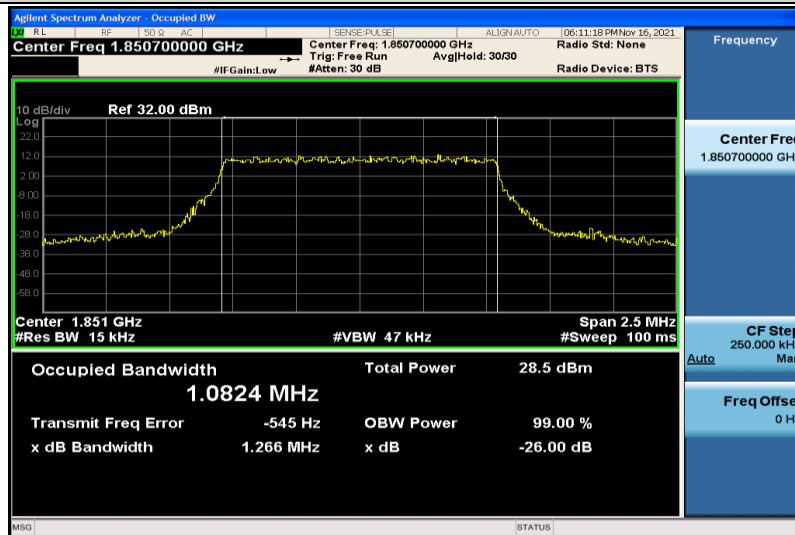
Band25-1.4MHz-16QAM-26047-6RB#0-1.0824
