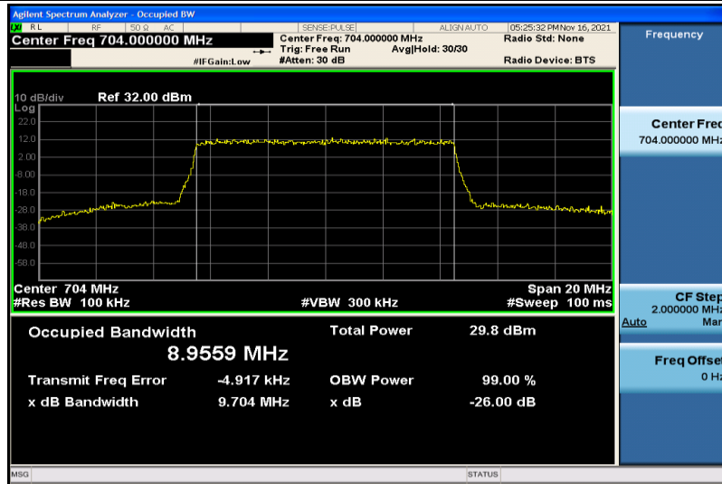
Band12-10MHz-16QAM-23060-50RB#0-8.9559
