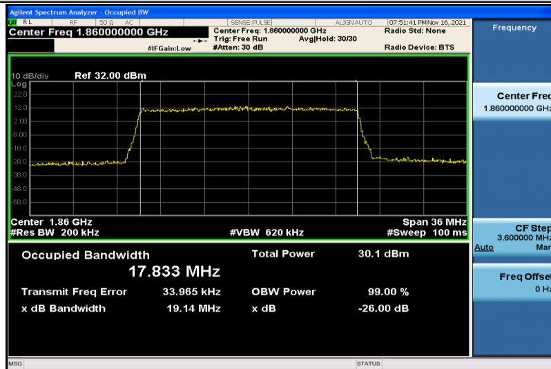
Band25-20MHz-16QAM-26140-100RB#0-17.833
