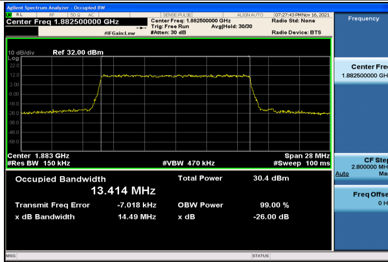
Band25-15MHz-QPSK-26365-75RB#0-13.414
