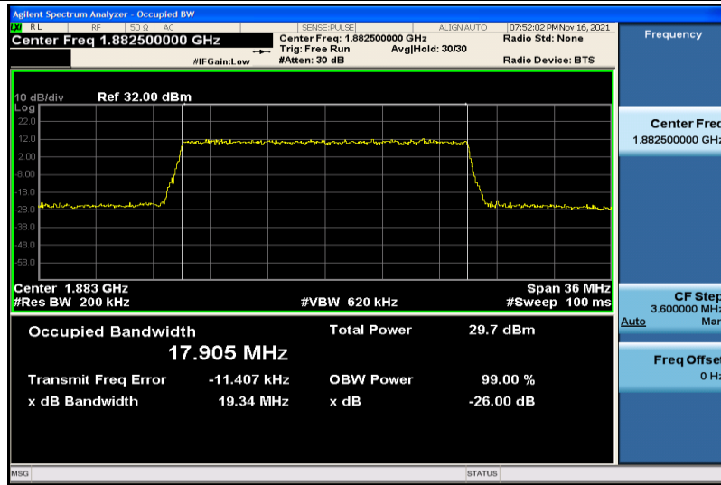
Band25-20MHz-16QAM-26365-100RB#0-17.905
