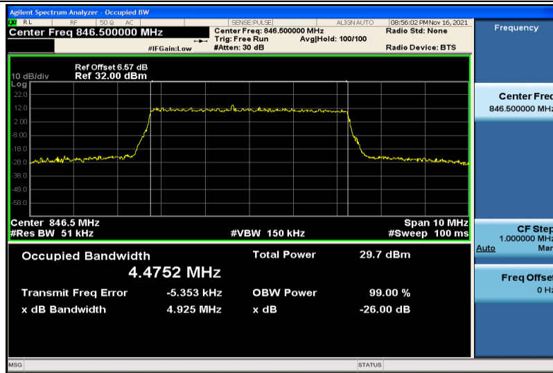
Band26-5MHz-16QAM-27015-25RB#0-4.4752
