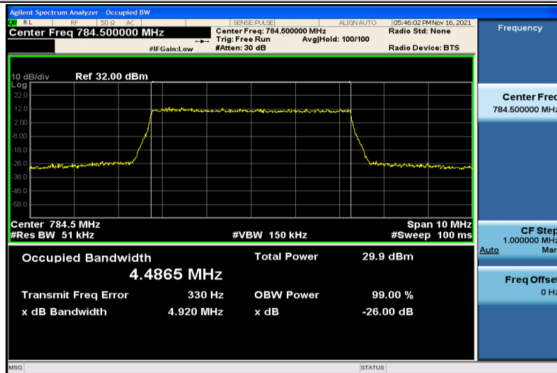
Band13-5MHz-16QAM-23255-25RB#0-4.4865
