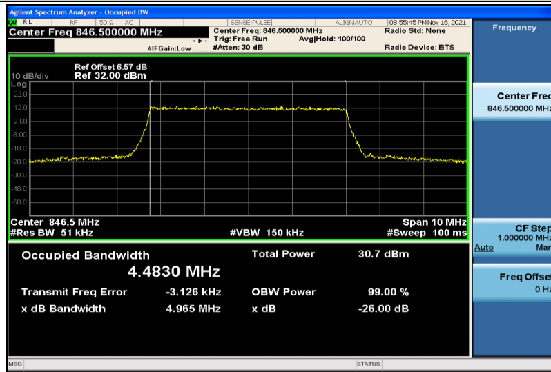
Band26-5MHz-QPSK-27015-25RB#0-4.4830
