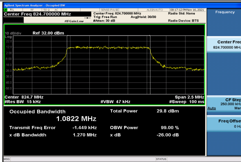
Band26-1.4MHz-QPSK-26797-6RB#0-1.0822
