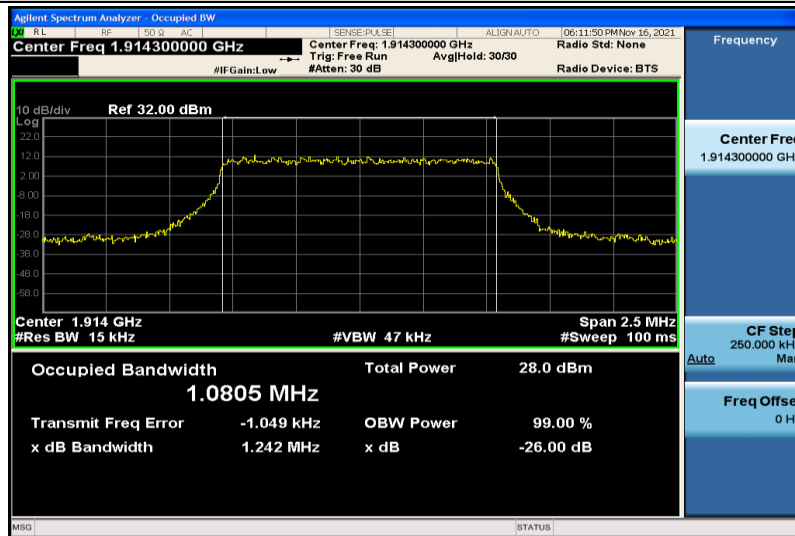
Band25-1.4MHz-QPSK-26683-6RB#0-1.0805
