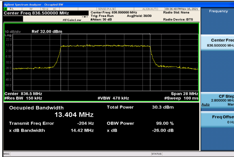
Band26-15MHz-16QAM-26915-75RB#0-13.404
