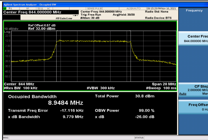
Band26-10MHz-QPSK-26990-50RB#0-8.9484
