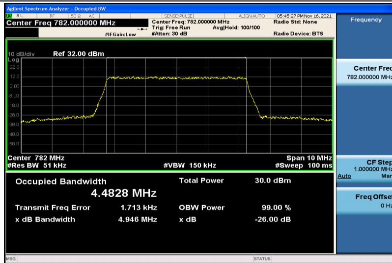
Band13-5MHz-16QAM-23230-25RB#0-4.4828
