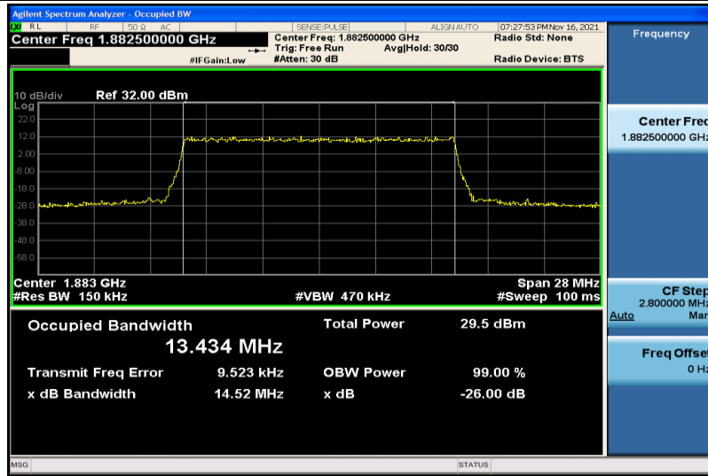
Band25-15MHz-16QAM-26365-75RB#0-13.434
