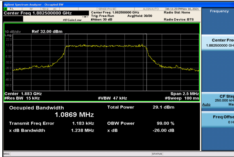
Band25-1.4MHz-QPSK-26365-6RB#0-1.0869
