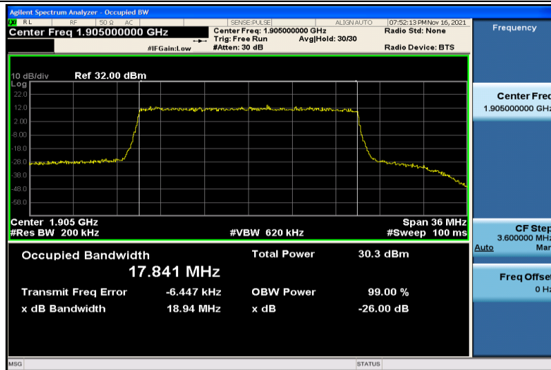
Band25-20MHz-QPSK-26590-100RB#0-17.841
