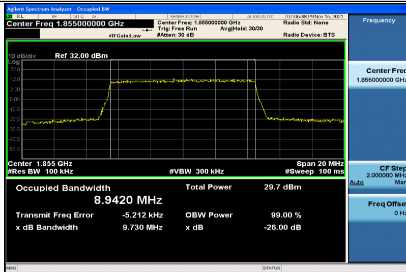
Band25-10MHz-16QAM-26090-50RB#0-8.9420
