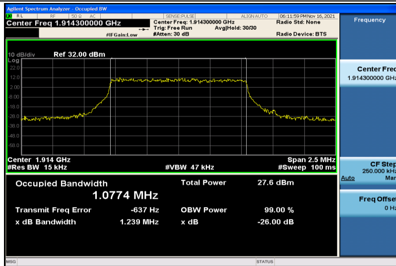
Band25-1.4MHz-16QAM-26683-6RB#0-1.0774
