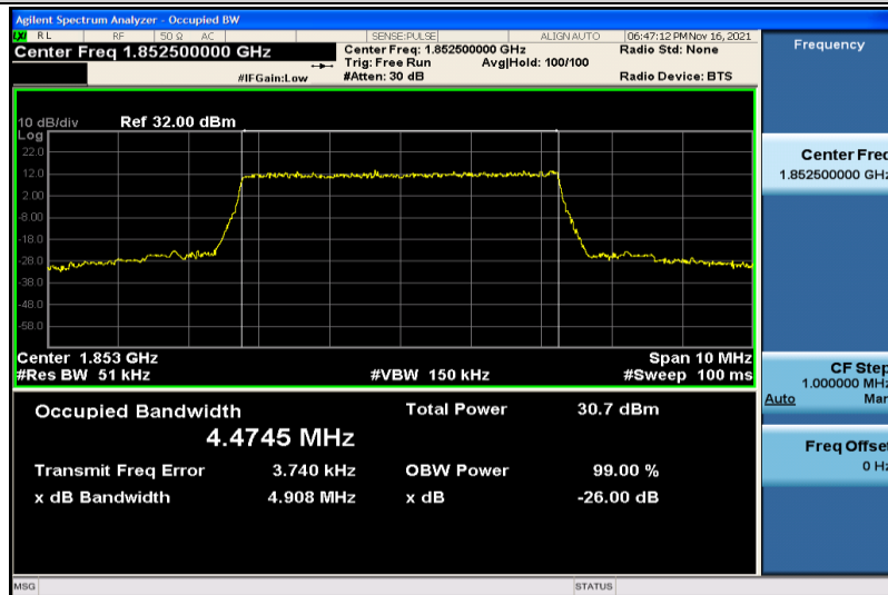
Band25-5MHz-QPSK-26065-25RB#0-4.4745
