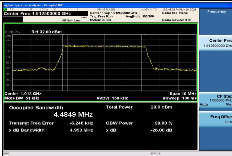
Band25-5MHz-QPSK-26665-25RB#0-4.4849
