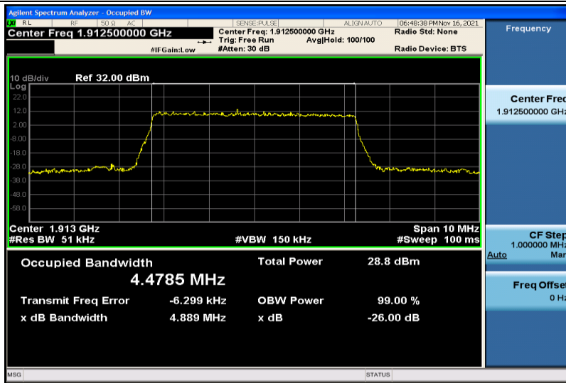
Band25-5MHz-16QAM-26665-25RB#0-4.4785
