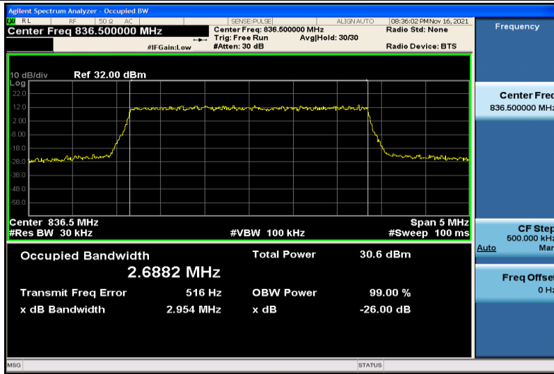
Band26-3MHz-QPSK-26915-15RB#0-2.6882
