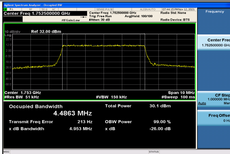
Band4-5MHz-QPSK-20375-25RB#0-4.4863
