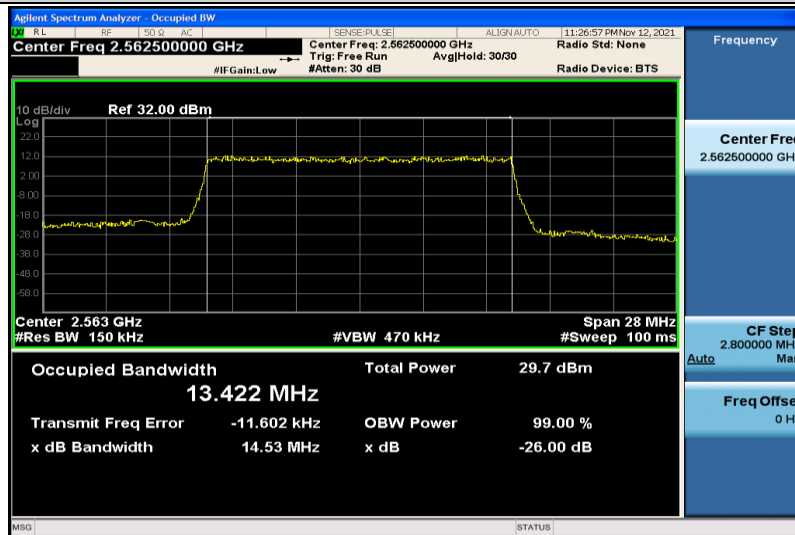
Band7-15MHz-16QAM-21375-75RB#0-13.422
