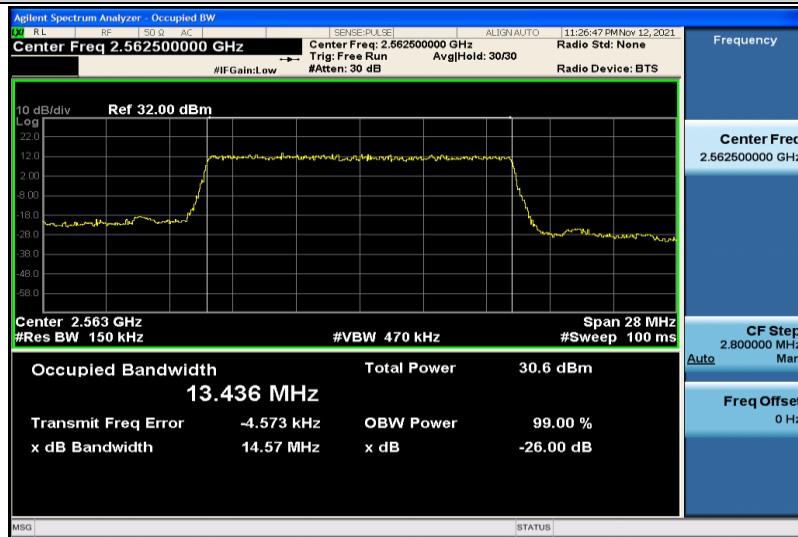
Band7-15MHz-QPSK-21375-75RB#0-13.436
