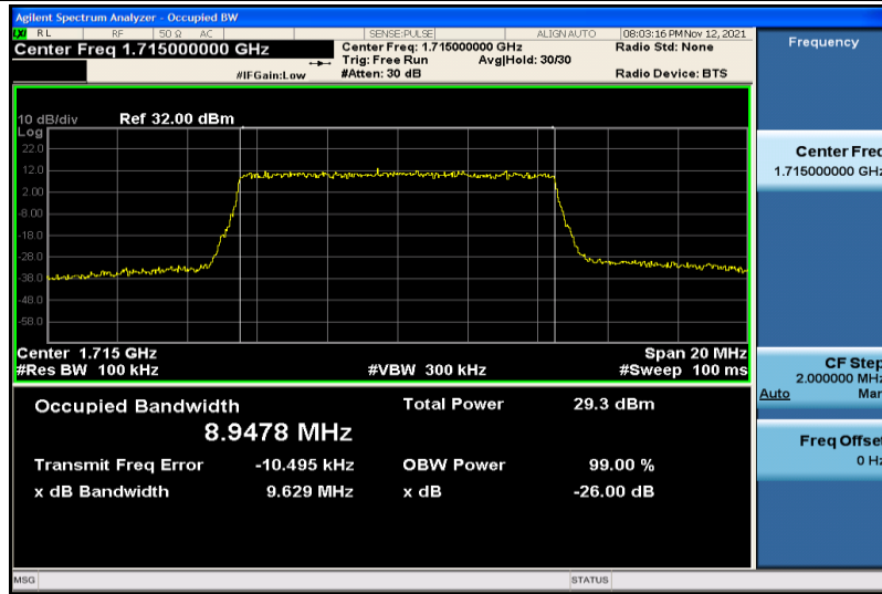
Band4-10MHz-16QAM-20000-50RB#0-8.9478
