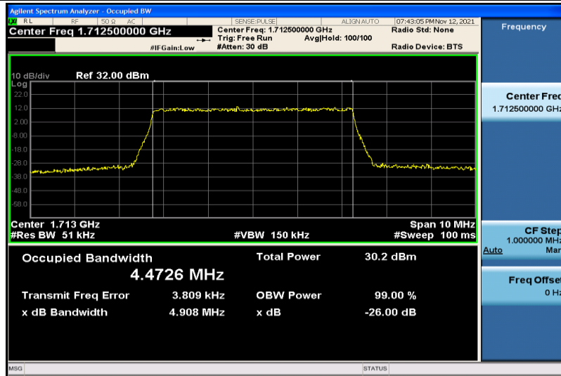
Band4-5MHz-QPSK-19975-25RB#0-4.4726
