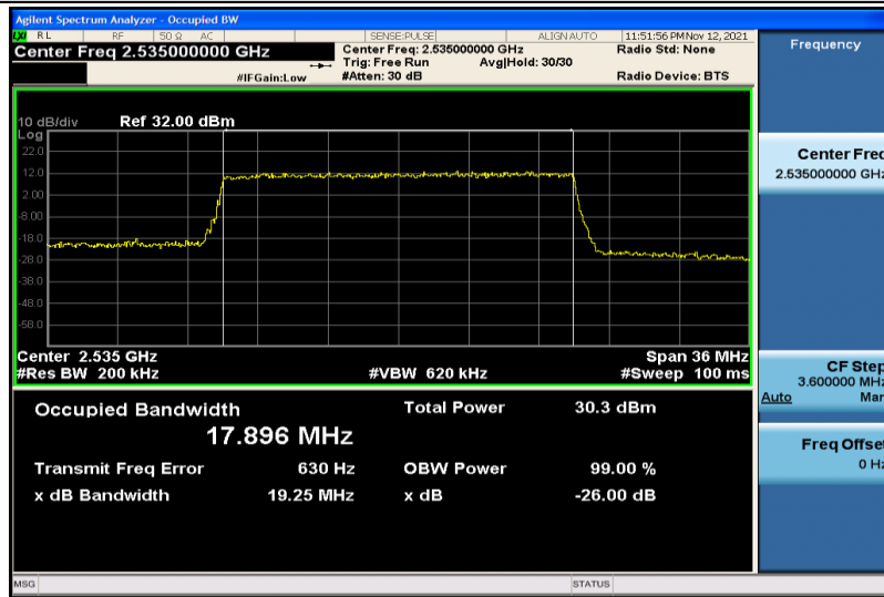
Band7-20MHz-16QAM-21100-100RB#0-17.896
