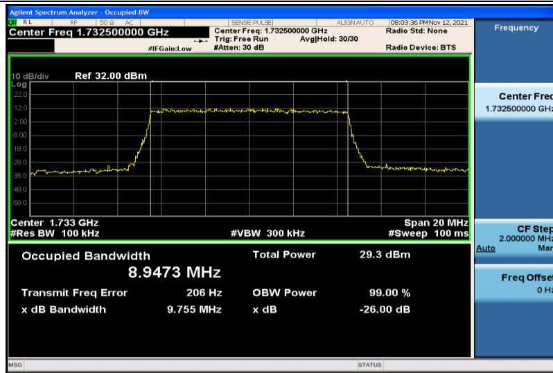
Band4-10MHz-16QAM-20175-50RB#0-8.9473
