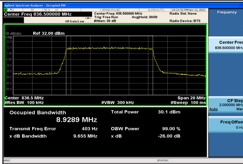
Band5-10MHz-16QAM-20525-50RB#0-8.9289
