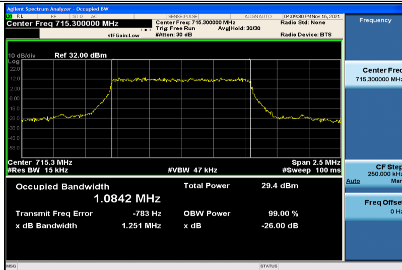
Band12-1.4MHz-QPSK-23173-6RB#0-1.0842
