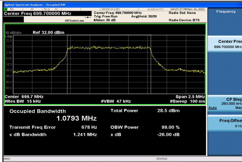
Band12-1.4MHz-16QAM-23017-6RB#0-1.0793
