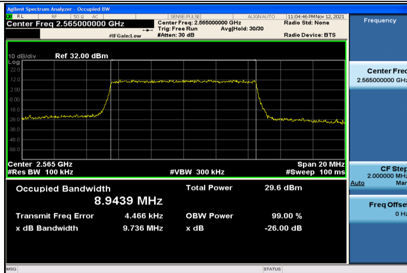
Band7-10MHz-16QAM-21400-50RB#0-8.9439
