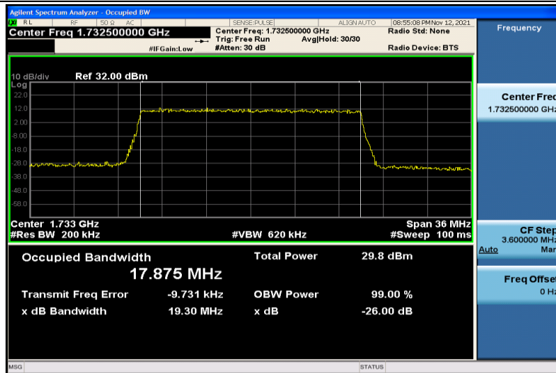
Band4-20MHz-16QAM-20175-100RB#0-17.875
