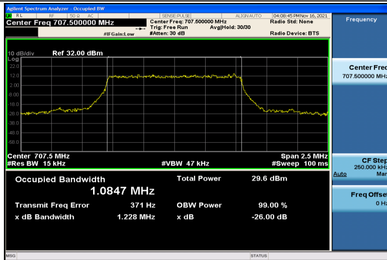
Band12-1.4MHz-QPSK-23095-6RB#0-1.0847
