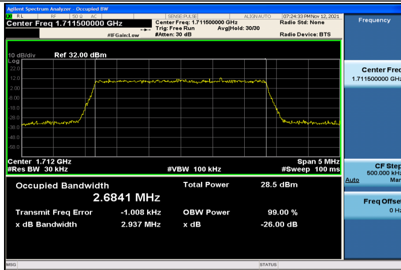
Band4-3MHz-16QAM-19965-15RB#0-2.6841
