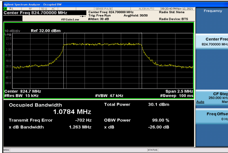
Band5-1.4MHz-QPSK-20407-6RB#0-1.0784
