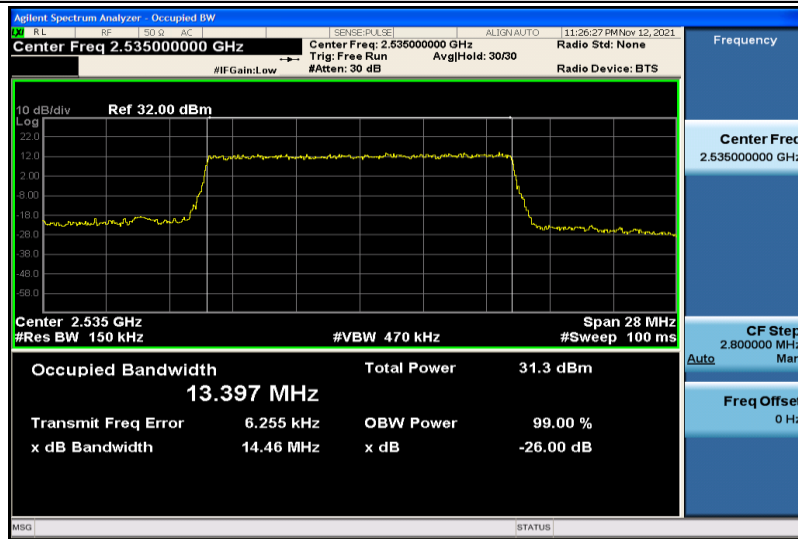
Band7-15MHz-QPSK-21100-75RB#0-13.397
