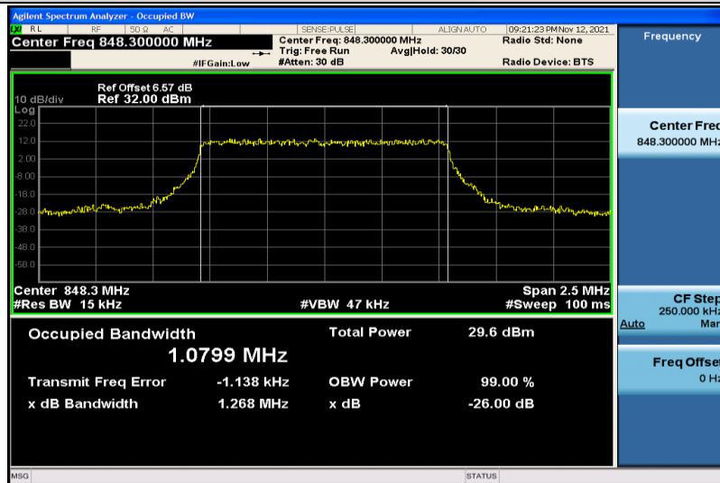
Band5-1.4MHz-QPSK-20643-6RB#0-1.0799
