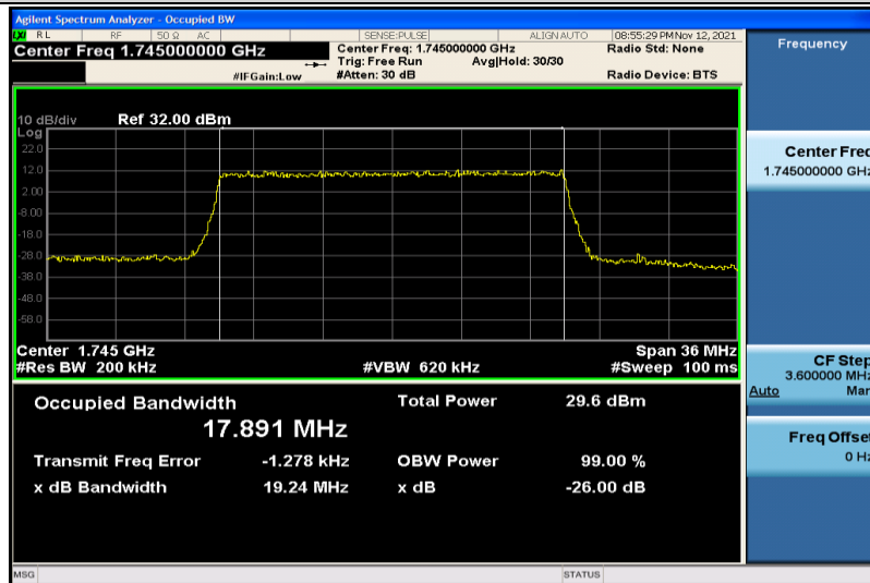
Band4-20MHz-16QAM-20300-100RB#0-17.891
