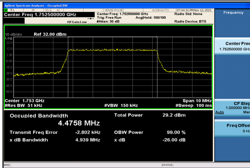
Band4-5MHz-16QAM-20375-25RB#0-4.4758
