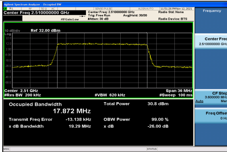
Band7-20MHz-QPSK-20850-100RB#0-17.872
