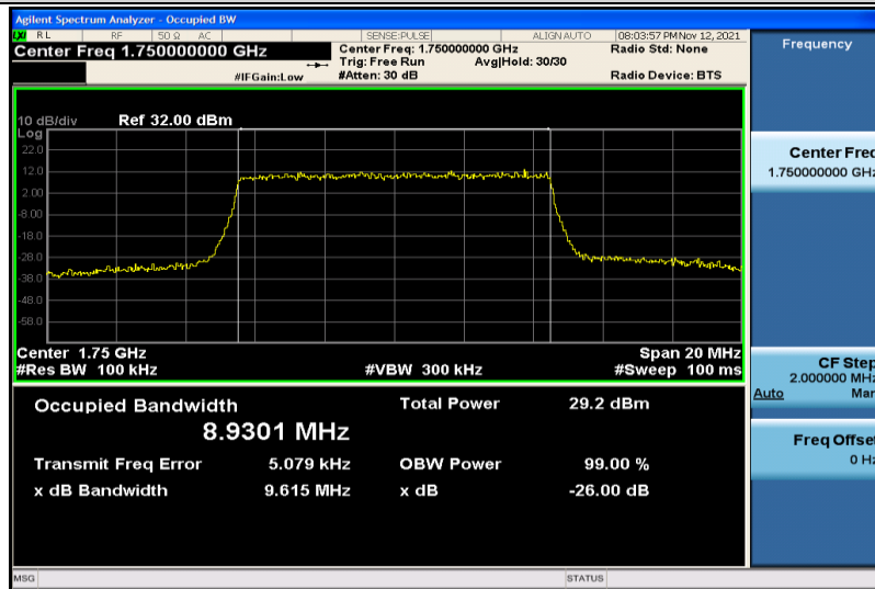
Band4-10MHz-16QAM-20350-50RB#0-8.9301
