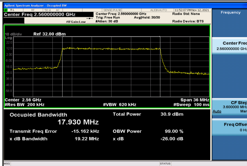
Band7-20MHz-QPSK-21350-100RB#0-17.930
