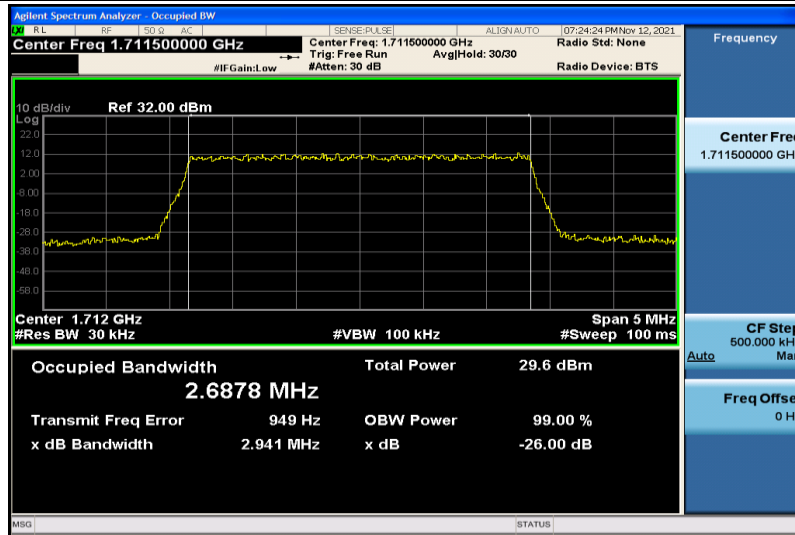
Band4-3MHz-QPSK-19965-15RB#0-2.6878
