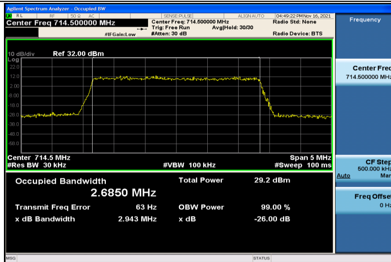
Band12-3MHz-16QAM-23165-15RB#0-2.6850
