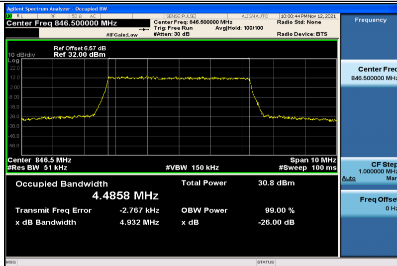
Band5-5MHz-QPSK-20625-25RB#0-4.4858
