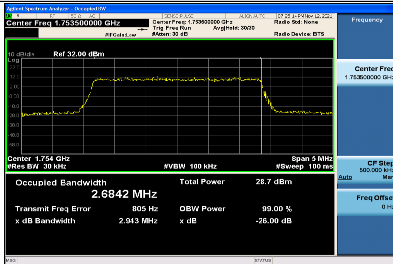
Band4-3MHz-16QAM-20385-15RB#0-2.6842
