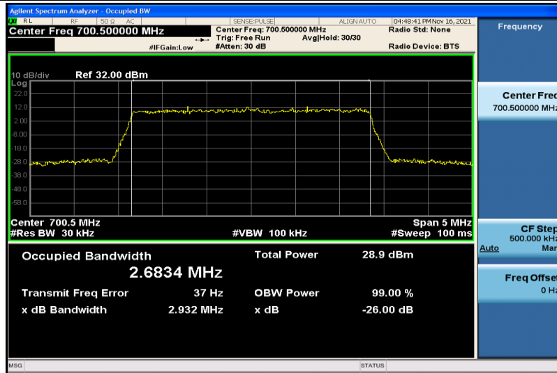
Band12-3MHz-16QAM-23025-15RB#0-2.6834
