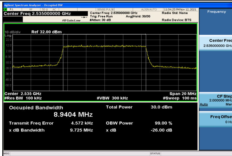
Band7-10MHz-16QAM-21100-50RB#0-8.9404
