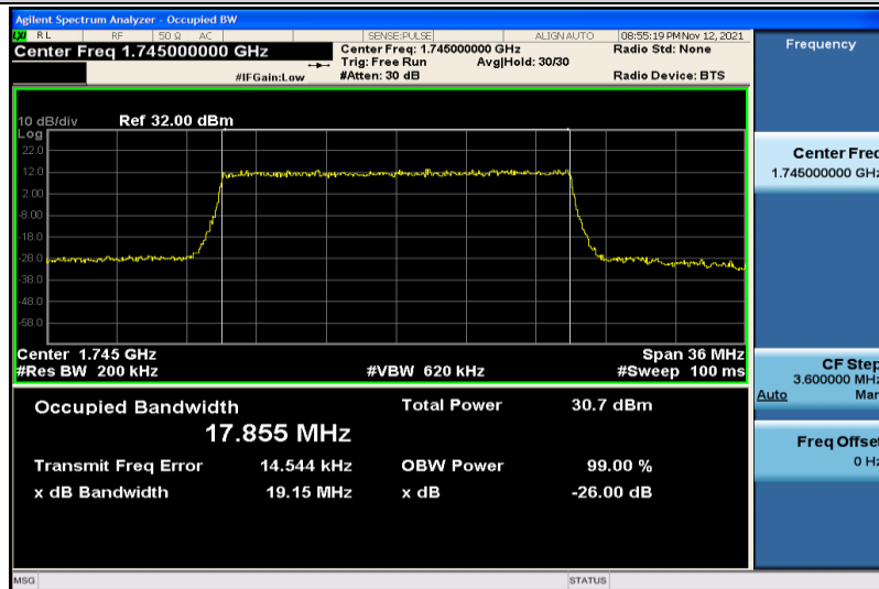
Band4-20MHz-QPSK-20300-100RB#0-17.855
