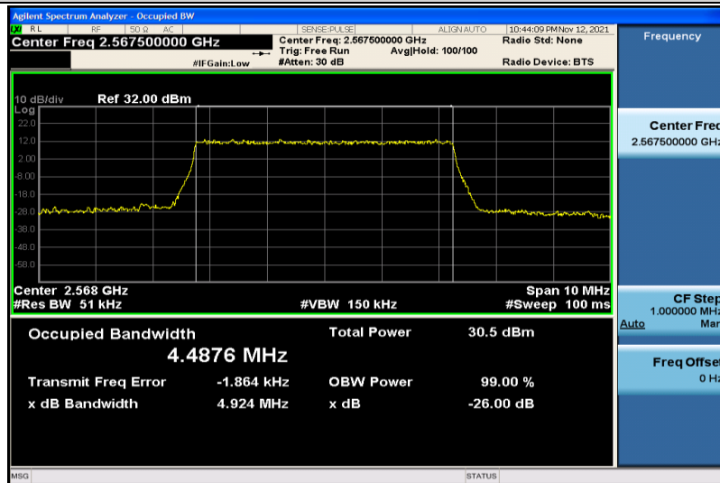
Band7-5MHz-QPSK-21425-25RB#0-4.4876
