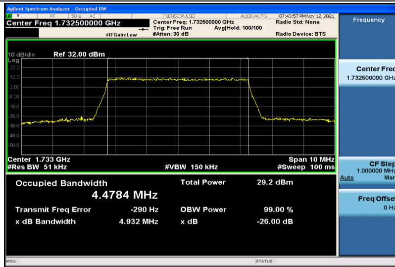
Band4-5MHz-16QAM-20175-25RB#0-4.4784
