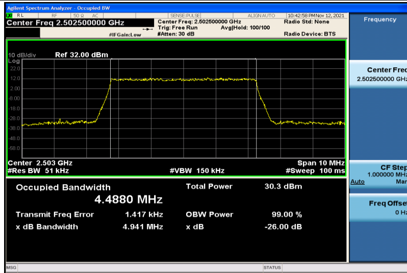
Band7-5MHz-QPSK-20775-25RB#0-4.4880
