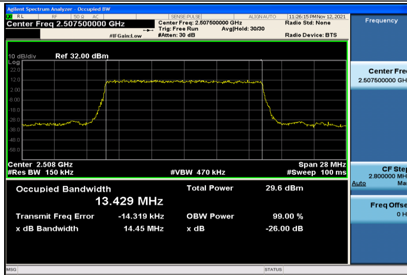
Band7-15MHz-16QAM-20825-75RB#0-13.429
