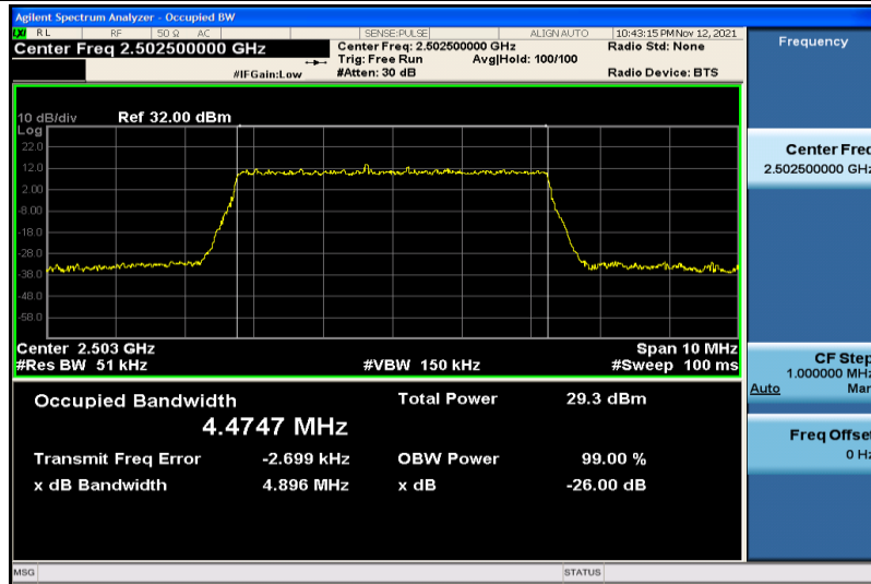
Band7-5MHz-16QAM-20775-25RB#0-4.4747
