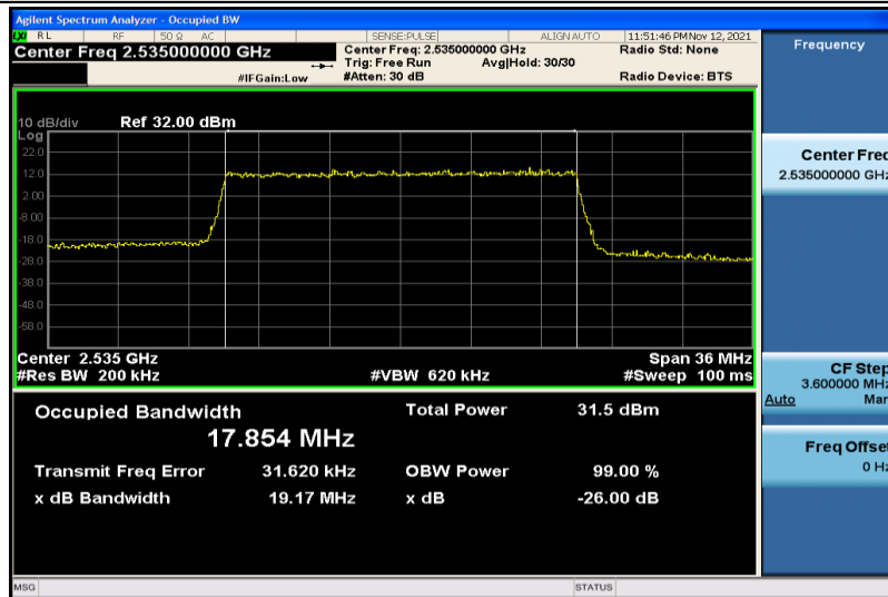
Band7-20MHz-QPSK-21100-100RB#0-17.854
