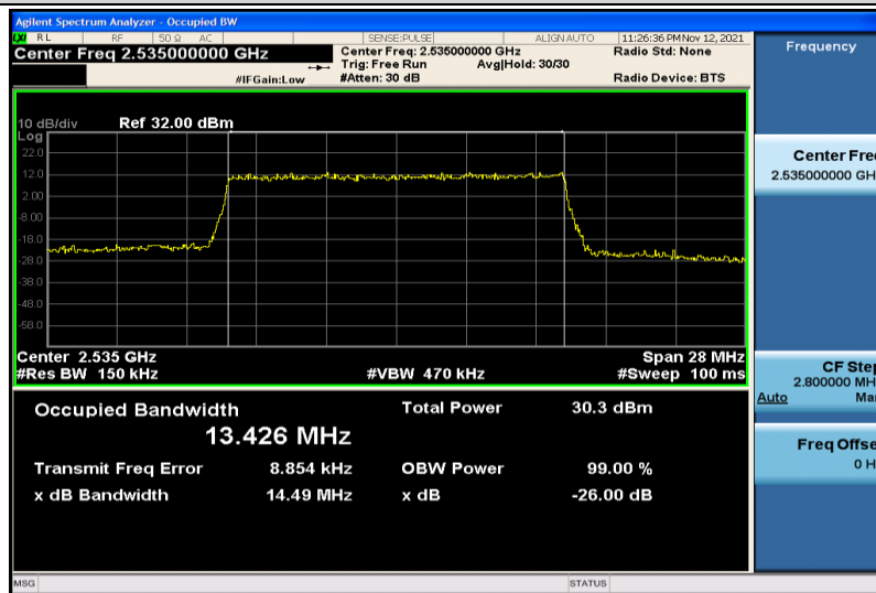
Band7-15MHz-16QAM-21100-75RB#0-13.426
