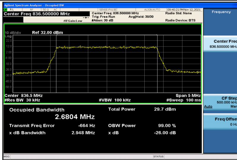
Band5-3MHz-16QAM-20525-15RB#0-2.6804
