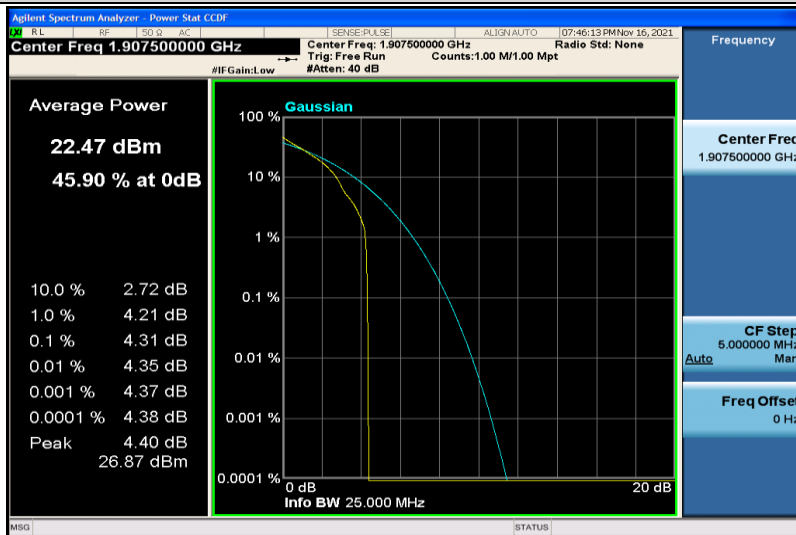
Band25-15MHz-QPSK-26615-1RB#0
