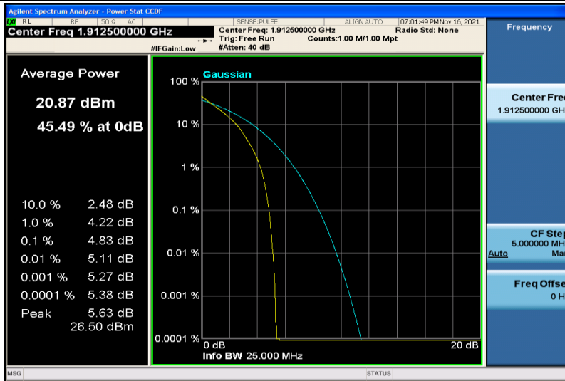
Band25-5MHz-QPSK-26665-25RB#0
