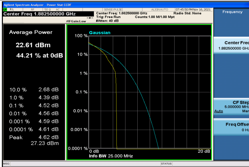
Band25-15MHz-QPSK-26365-1RB#0
