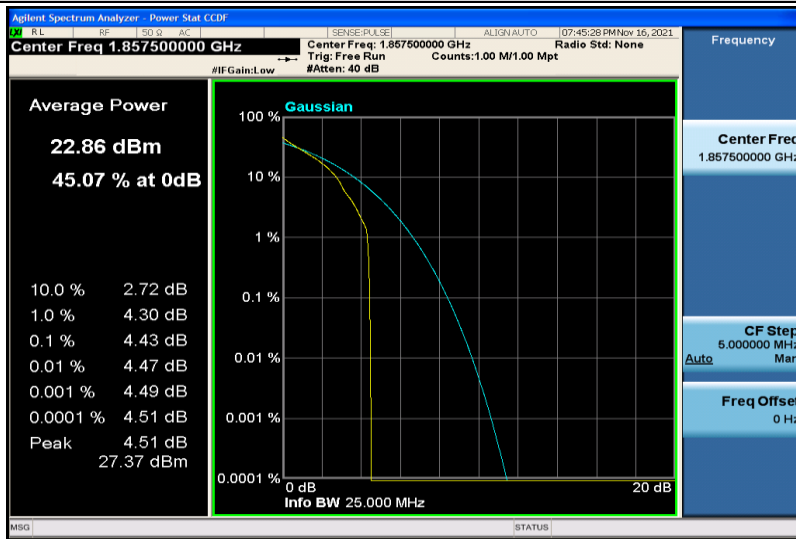
Band25-15MHz-QPSK-26115-1RB#0
