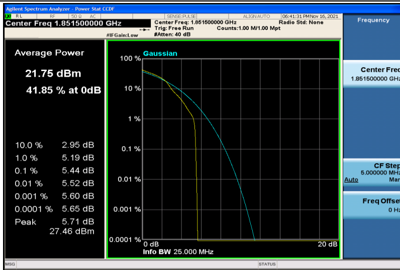
Band25-3MHz-16QAM-26055-1RB#0
