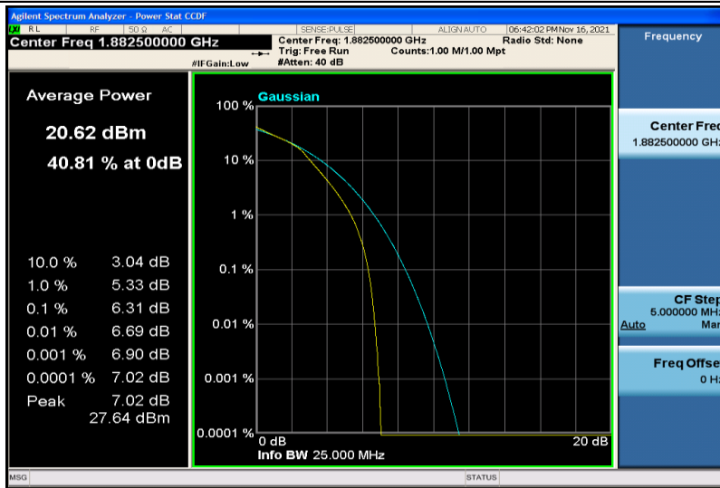
Band25-3MHz-16QAM-26365-15RB#0
