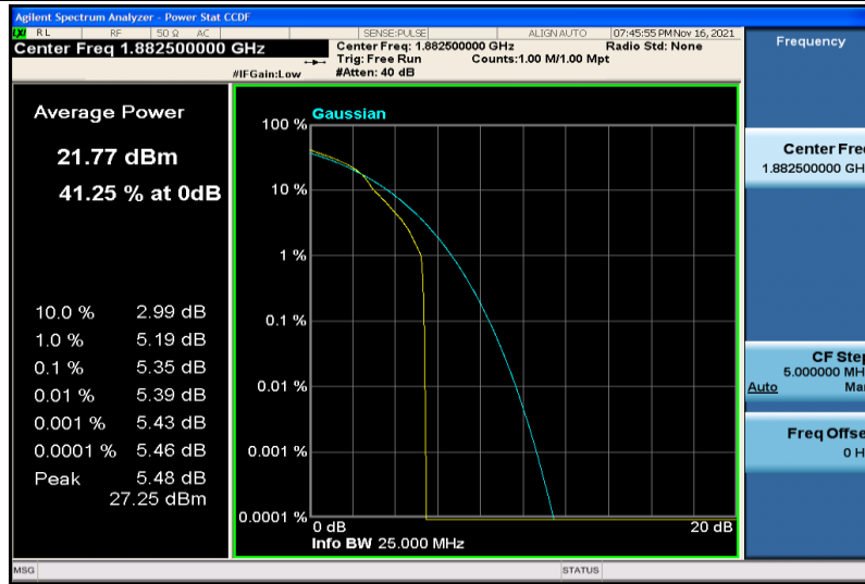
Band25-15MHz-16QAM-26365-1RB#0
