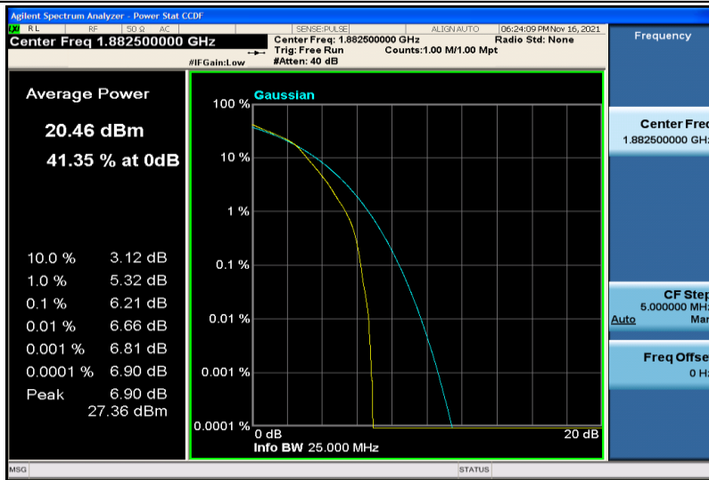
Band25-1.4MHz-16QAM-26365-6RB#0
