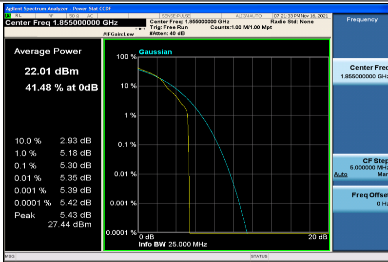
Band25-10MHz-16QAM-26090-1RB#0
