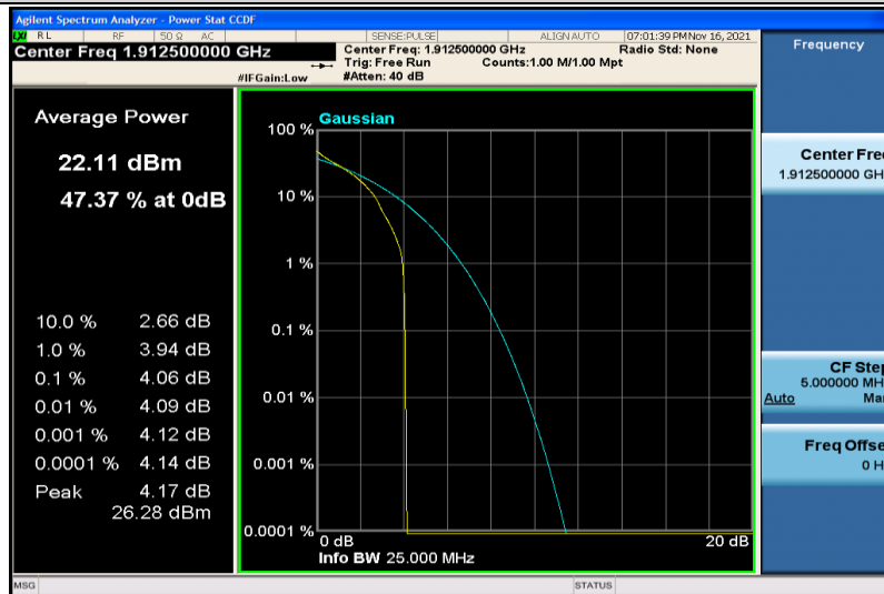
Band25-5MHz-QPSK-26665-1RB#0
