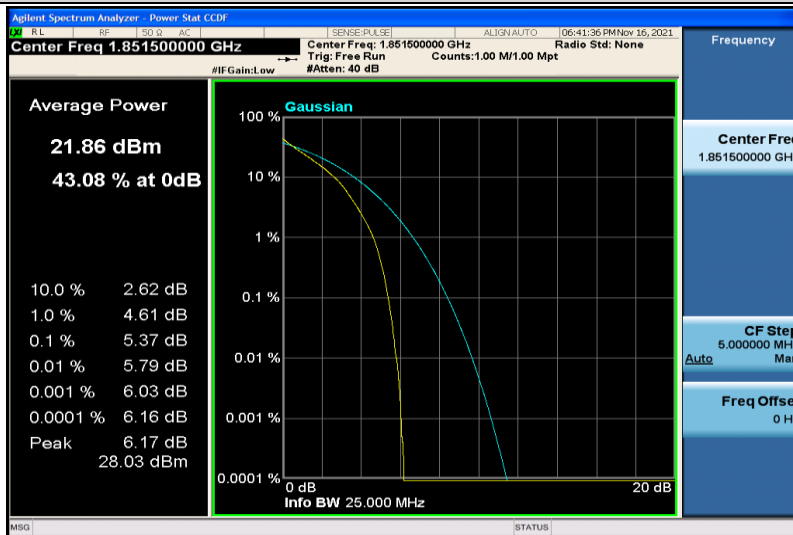
Band25-3MHz-QPSK-26055-15RB#0
