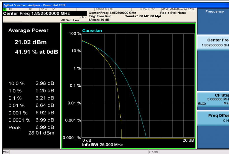
Band25-5MHz-16QAM-26065-25RB#0
