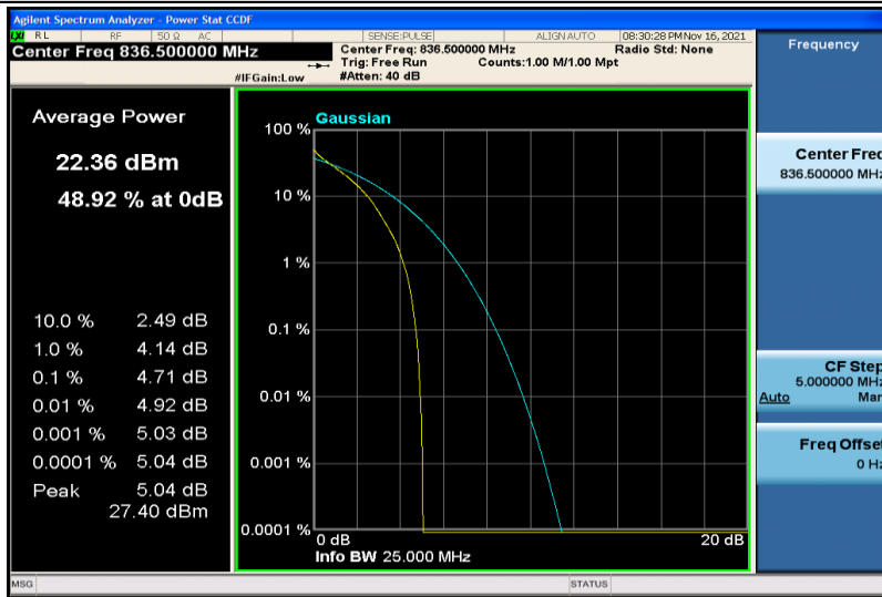
Band26-1.4MHz-QPSK-26915-6RB#0
