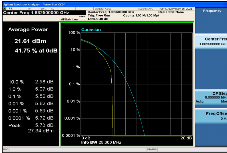
Band25-3MHz-16QAM-26365-1RB#0
