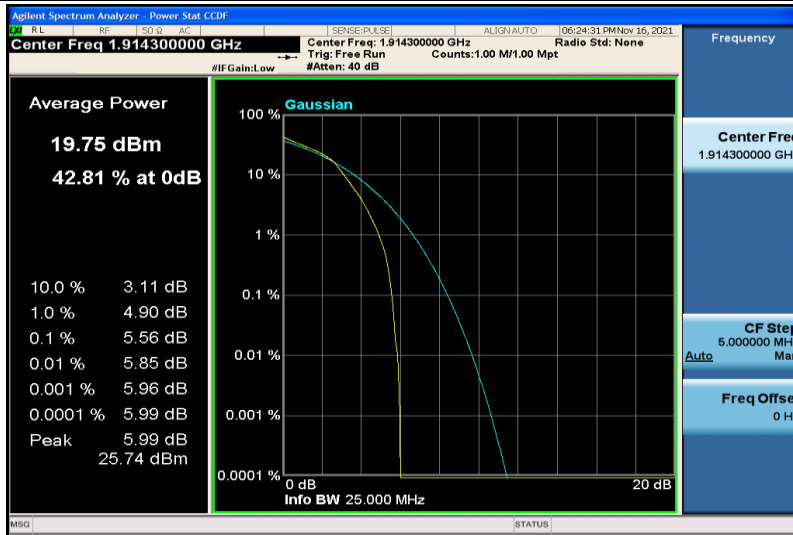
Band25-1.4MHz-16QAM-26683-6RB#0
