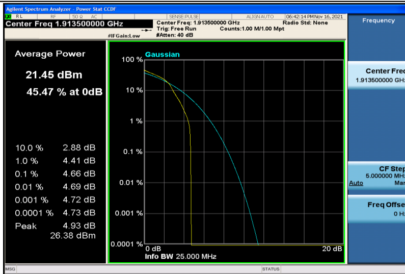
Band25-3MHz-16QAM-26675-1RB#0
