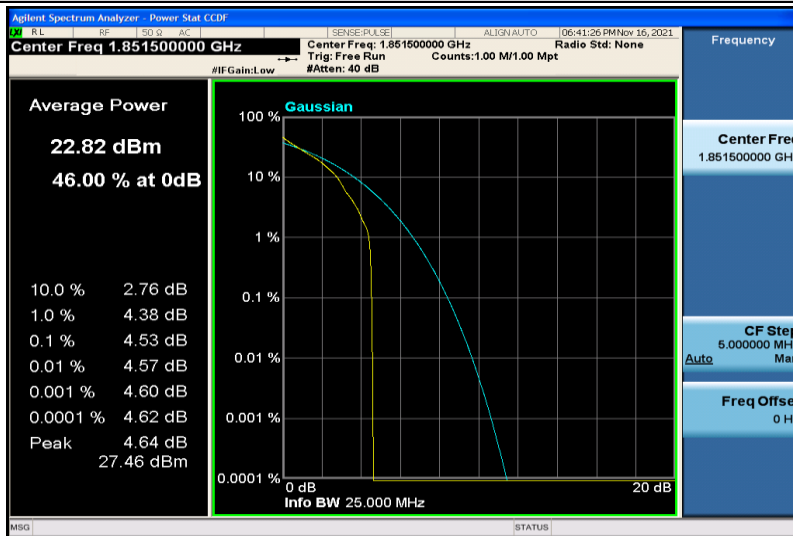
Band25-3MHz-QPSK-26055-1RB#0
