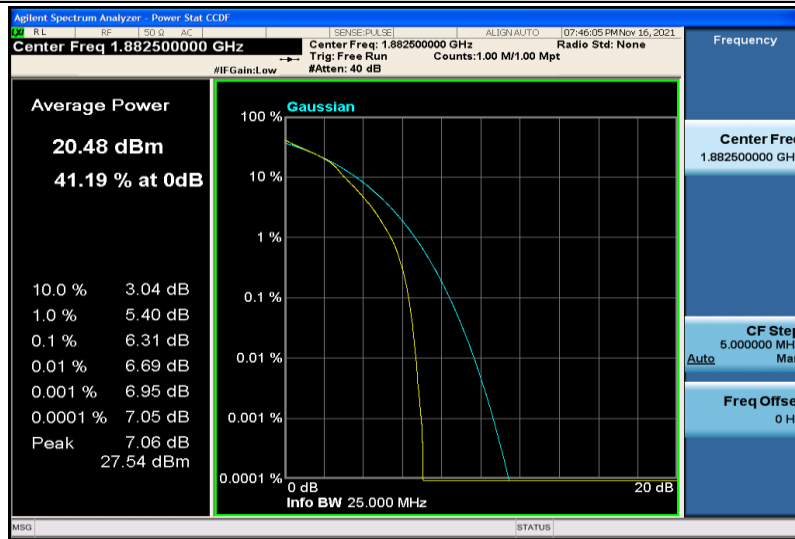
Band25-15MHz-16QAM-26365-75RB#0
