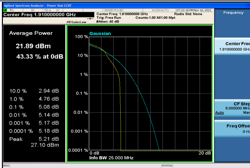
Band25-10MHz-16QAM-26640-1RB#0
