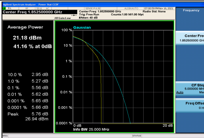
Band25-5MHz-16QAM-26065-1RB#0
