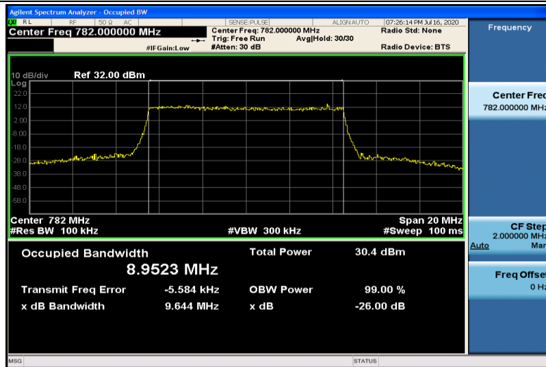
Band13-10MHz-16QAM-23230-50RB#0-8.9523
