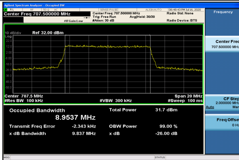
Band12-10MHz-QPSK-23095-50RB#0-8.9537
