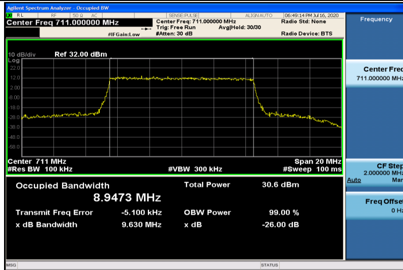
Band12-10MHz-16QAM-23130-50RB#0-8.9473
