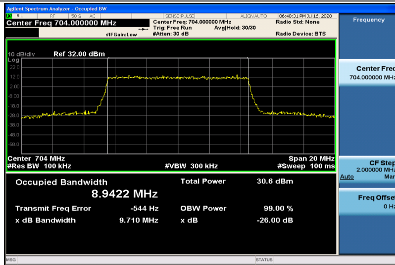
Band12-10MHz-16QAM-23060-50RB#0-8.9422
