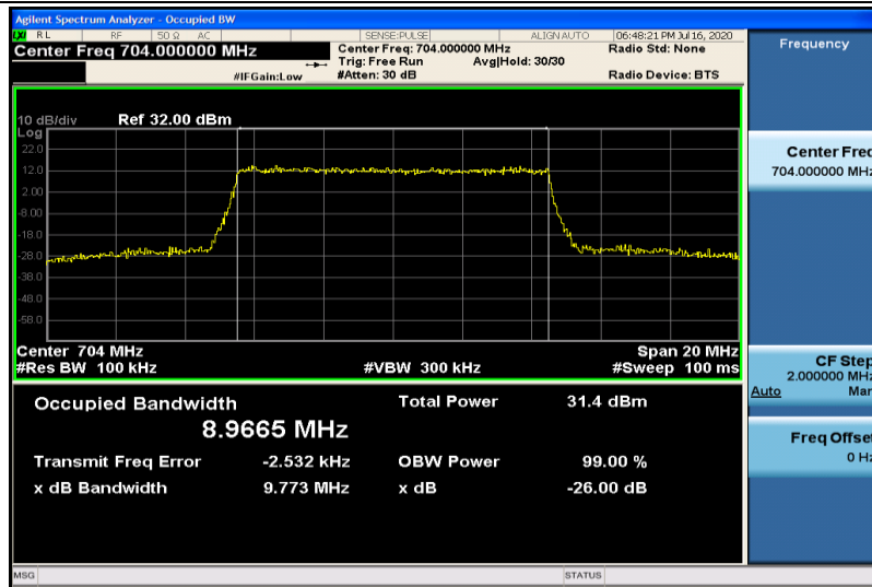
Band12-10MHz-QPSK-23060-50RB#0-8.9665
