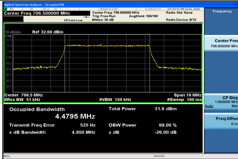
Band17-5MHz-QPSK-23755-25RB#0-4.4795
