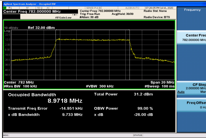
Band13-10MHz-QPSK-23230-50RB#0-8.9718
