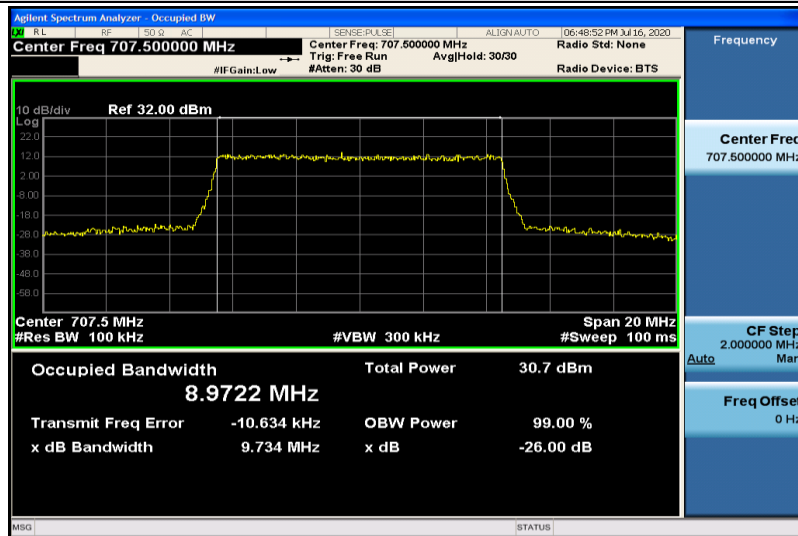
Band12-10MHz-16QAM-23095-50RB#0-8.9722
