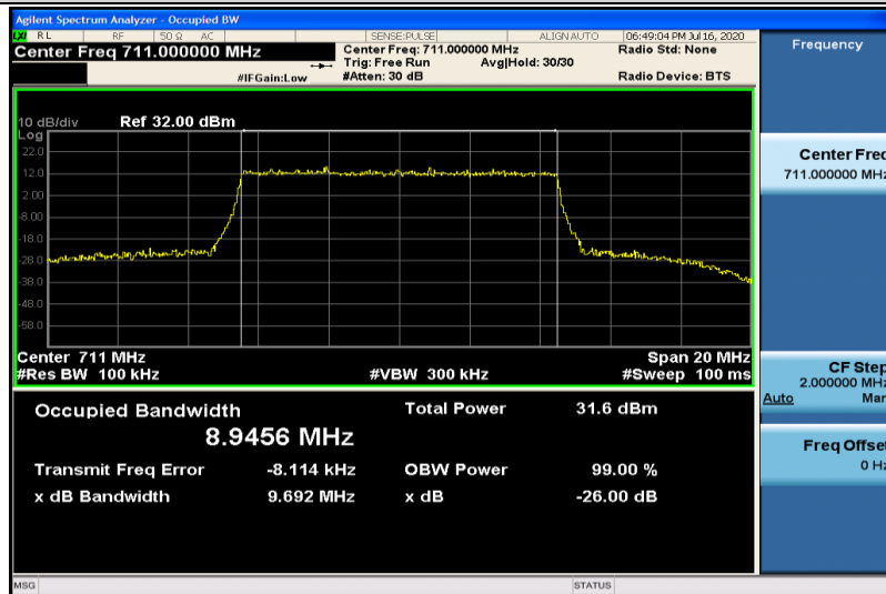
Band12-10MHz-QPSK-23130-50RB#0-8.9456
