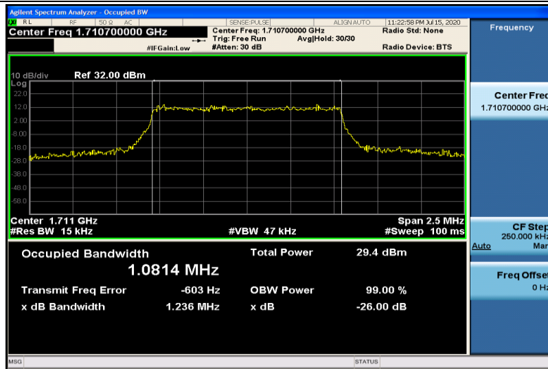
Band4-1.4MHz-16QAM-19957-6RB#0-1.0814
