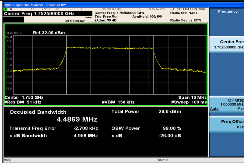
Band4-5MHz-16QAM-20375-25RB#0-4.4869
