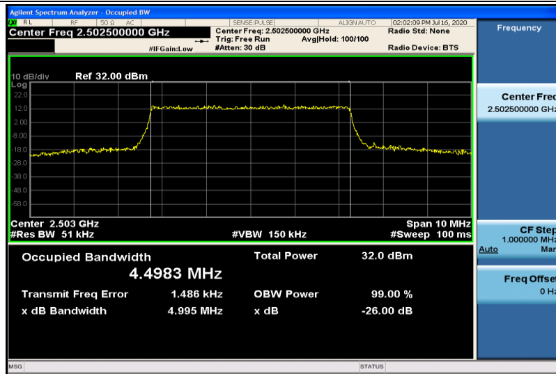
Band7-5MHz-QPSK-20775-25RB#0-4.4983
