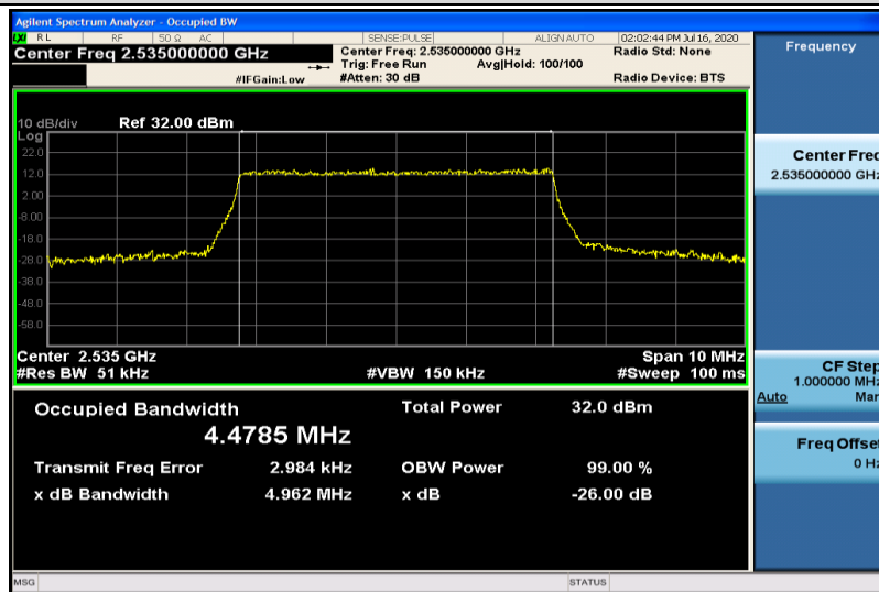
Band7-5MHz-QPSK-21100-25RB#0-4.4785
