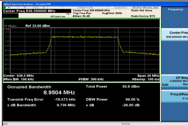
Band5-10MHz-16QAM-20525-50RB#0-8.9504
