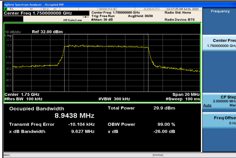
Band4-10MHz-16QAM-20350-50RB#0-8.9438
