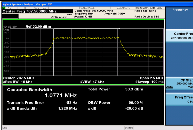
Band12-1.4MHz-QPSK-23095-6RB#0-1.0771
