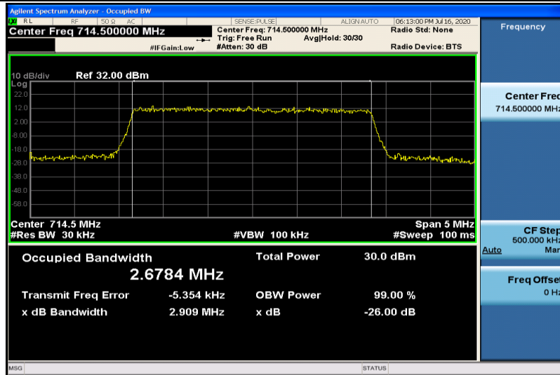
Band12-3MHz-16QAM-23165-15RB#0-2.6784
