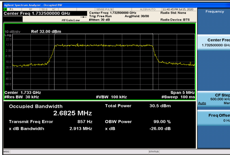
Band4-3MHz-16QAM-20175-15RB#0-2.6825
