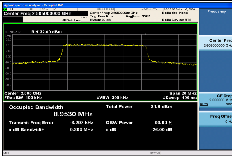
Band7-10MHz-QPSK-20800-50RB#0-8.9530
