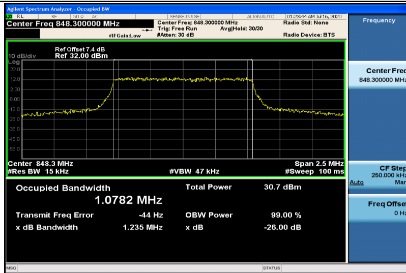
Band5-1.4MHz-QPSK-20643-6RB#0-1.0782
