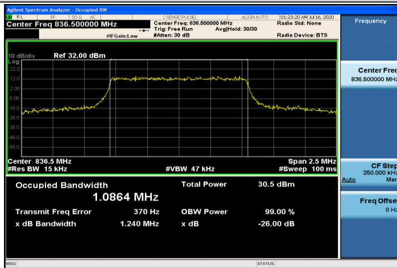
Band5-1.4MHz-QPSK-20525-6RB#0-1.0864
