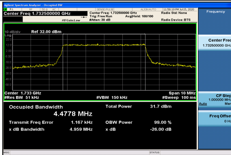
Band4-5MHz-QPSK-17325-25RB#0-4.4778
