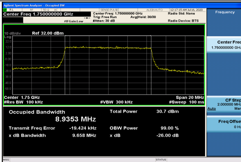
Band4-10MHz-QPSK-20350-50RB#0-8.9353
