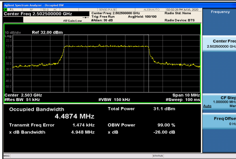
Band7-5MHz-16QAM-20775-25RB#0-4.4874
