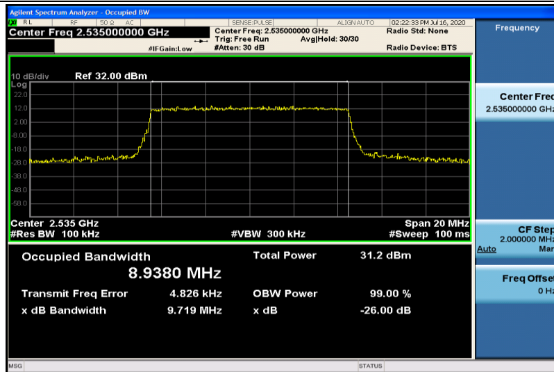
Band7-10MHz-16QAM-21100-50RB#0-8.9380
