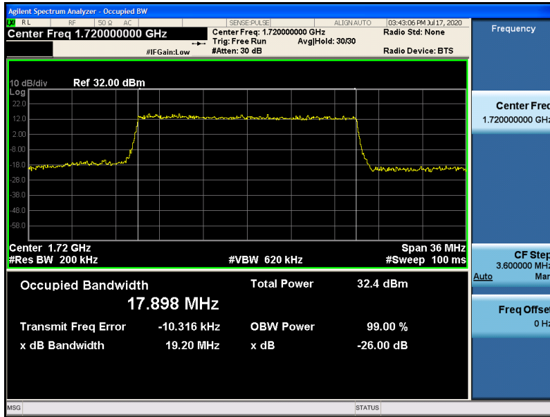
Band4-20MHz-QPSK-20050-100RB#0-17.898
