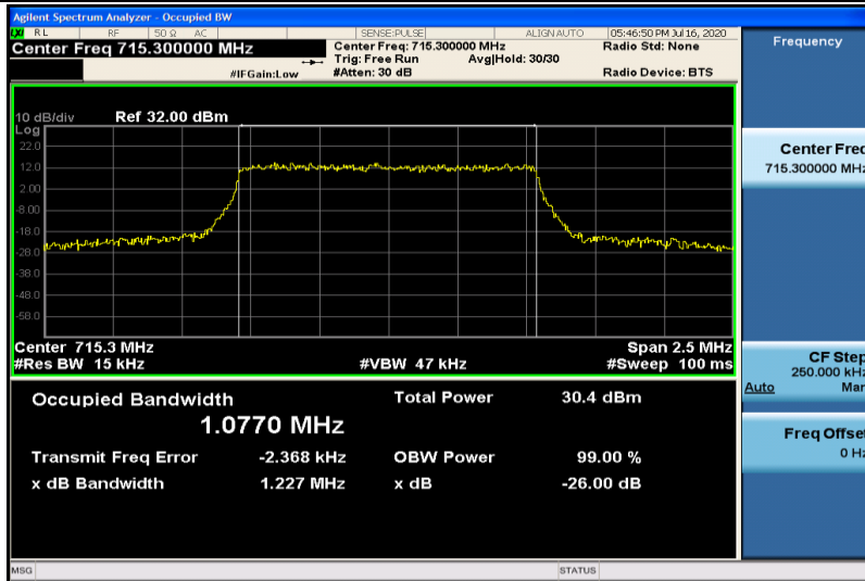
Band12-1.4MHz-QPSK-23173-6RB#0-1.0770
