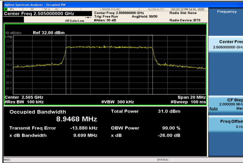
Band7-10MHz-16QAM-20800-50RB#0-8.9468
