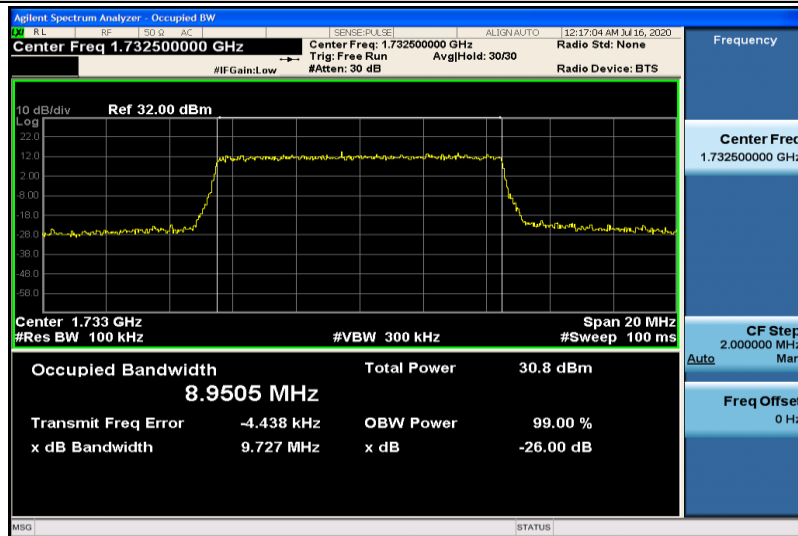
Band4-10MHz-16QAM-20175-50RB#0-8.9505
