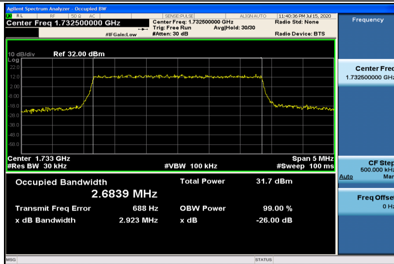
Band4-3MHz-QPSK-20175-15RB#0-2.6839
