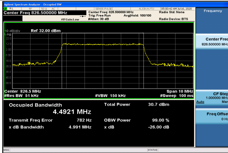
Band5-5MHz-16QAM-20425-25RB#0-4.4921
