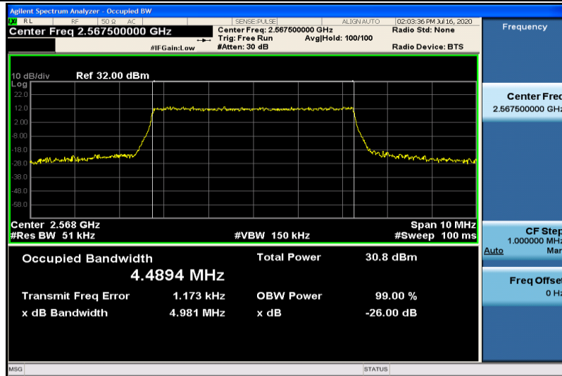
Band7-5MHz-16QAM-21425-25RB#0-4.4894
