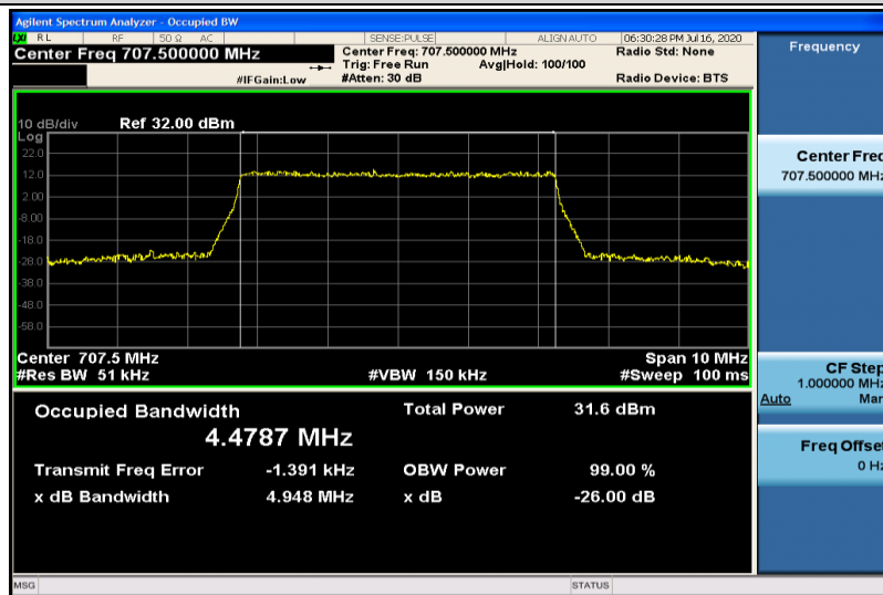
Band12-5MHz-QPSK-23095-25RB#0-4.4787
