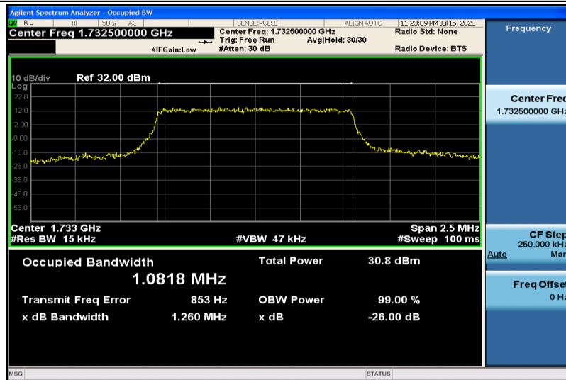
Band4-1.4MHz-QPSK-20175-6RB#0-1.0818
