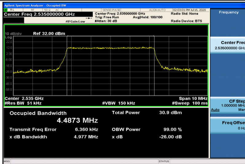
Band7-5MHz-16QAM-21100-25RB#0-4.4873
