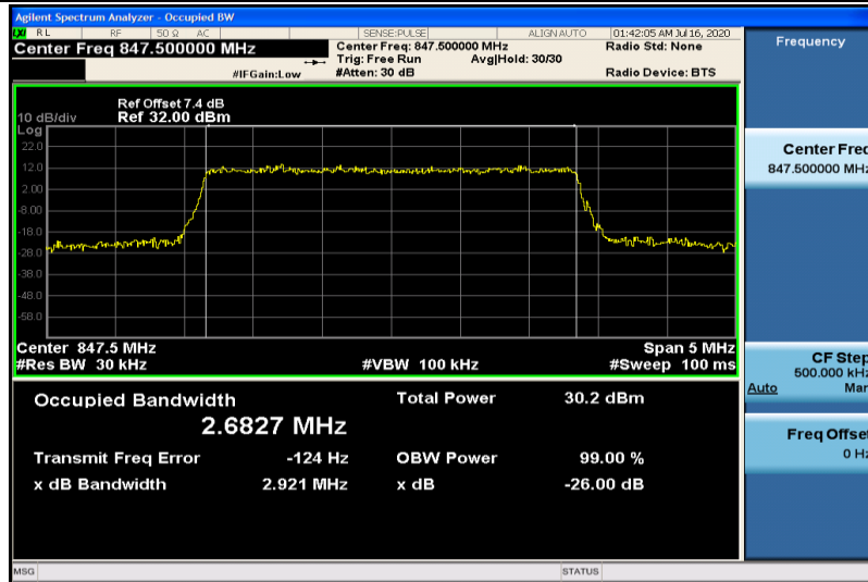
Band5-3MHz-16QAM-20635-15RB#0-2.6827
