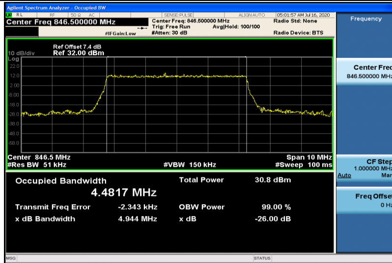
Band5-5MHz-16QAM-20625-25RB#0-4.4817
