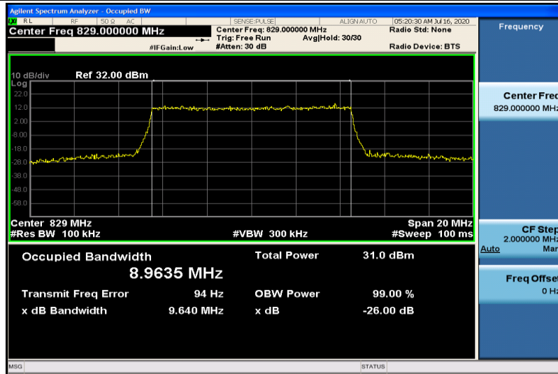
Band5-10MHz-16QAM-20450-50RB#0-8.9635
