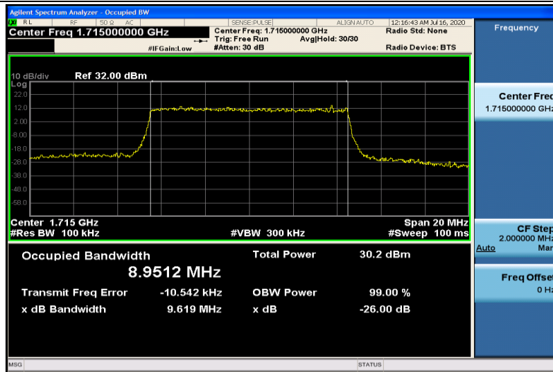
Band4-10MHz-16QAM-20000-50RB#0-8.9512
