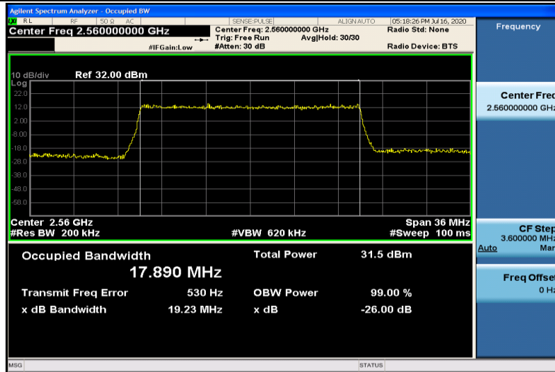
Band7-20MHz-QPSK-21350-100RB#0-17.890
