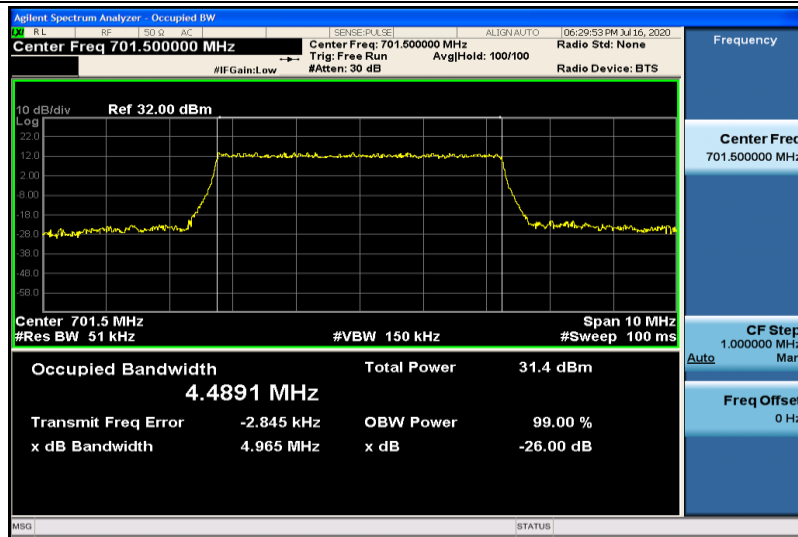
Band12-5MHz-QPSK-23035-25RB#0-4.4891
