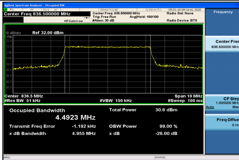
Band5-5MHz-16QAM-20525-25RB#0-4.4923
