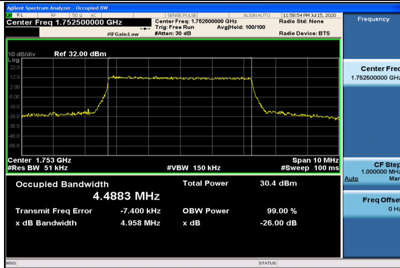
Band4-5MHz-QPSK-20175-25RB#0-4.4883
