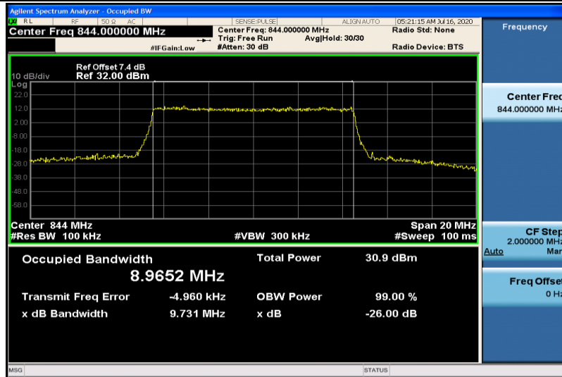
Band5-10MHz-16QAM-20600-50RB#0-8.9652
