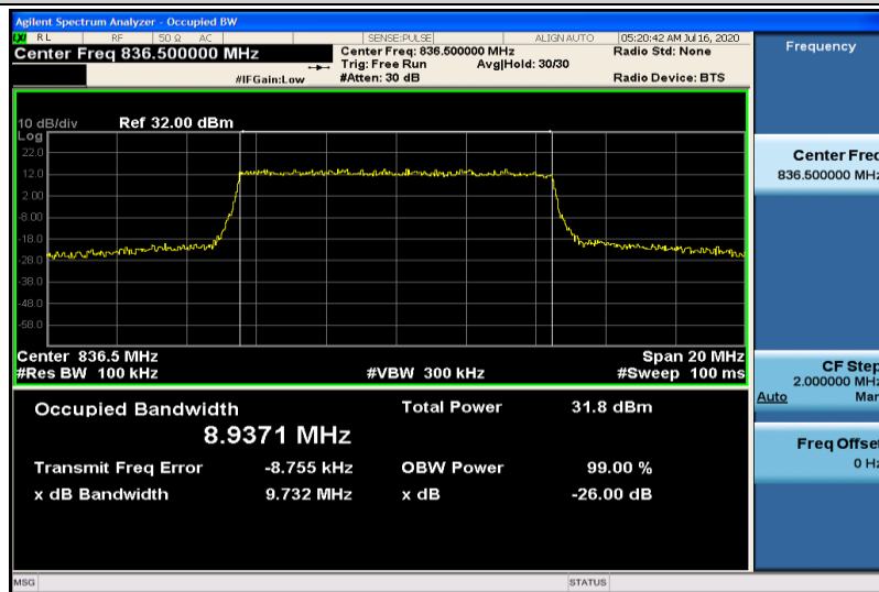
Band5-10MHz-QPSK-20525-50RB#0-8.9371
