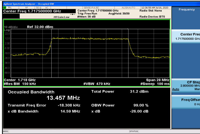
Band4-15MHz-QPSK-20025-75RB#0-13.457
