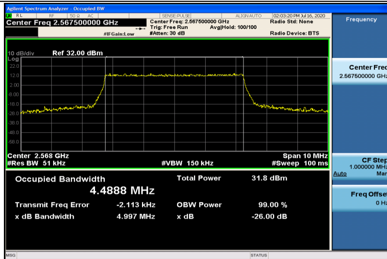
Band7-5MHz-QPSK-21425-25RB#0-4.4888
