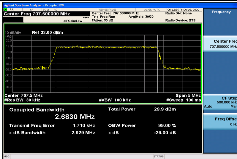
Band12-3MHz-16QAM-23095-15RB#0-2.6830
