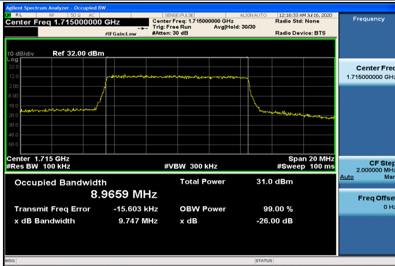
Band4-10MHz-QPSK-20000-50RB#0-8.9659
