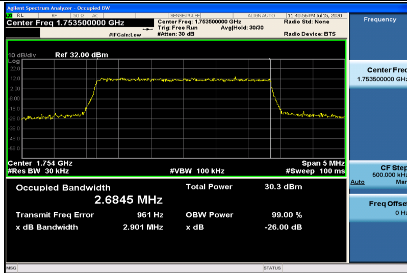
Band4-3MHz-QPSK-20385-15RB#0-2.6845
