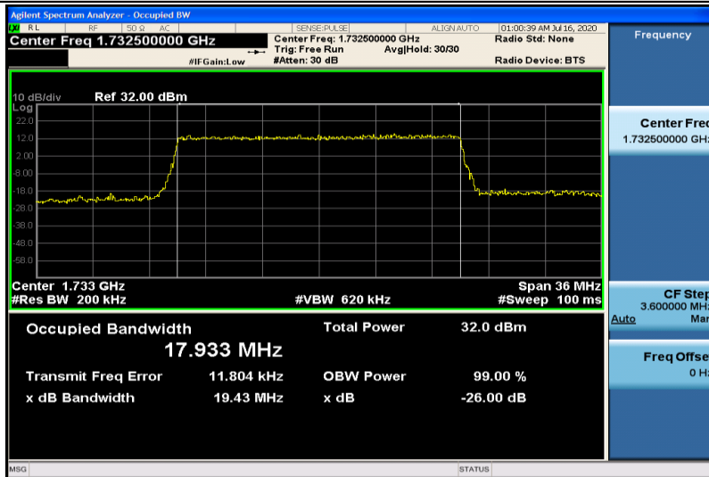
Band4-20MHz-QPSK-20175-100RB#0-17.933
