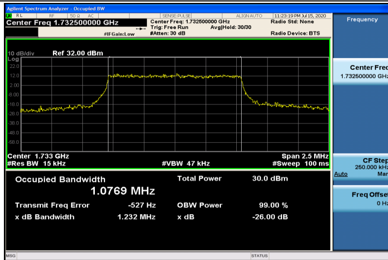
Band4-1.4MHz-16QAM-20175-6RB#0-1.0769
