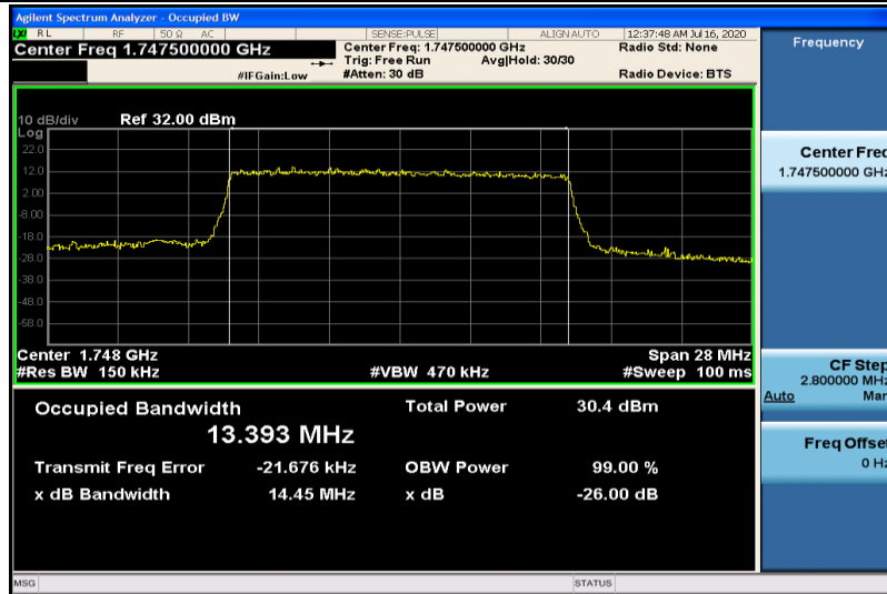
Band4-15MHz-16QAM-20325-75RB#0-13.393
