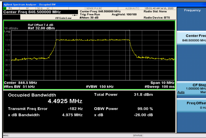
Band5-5MHz-QPSK-20625-25RB#0-4.4925
