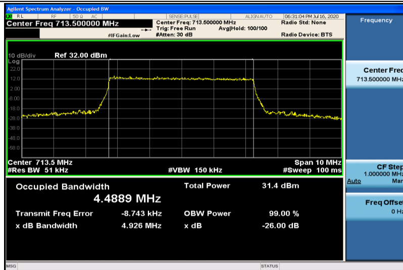
Band12-5MHz-QPSK-23155-25RB#0-4.4889
