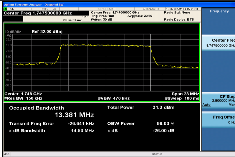
Band4-15MHz-QPSK-20325-75RB#0-13.381
