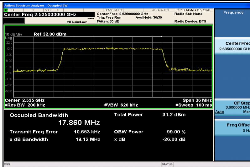
Band7-20MHz-16QAM-21100-100RB#0-17.860
