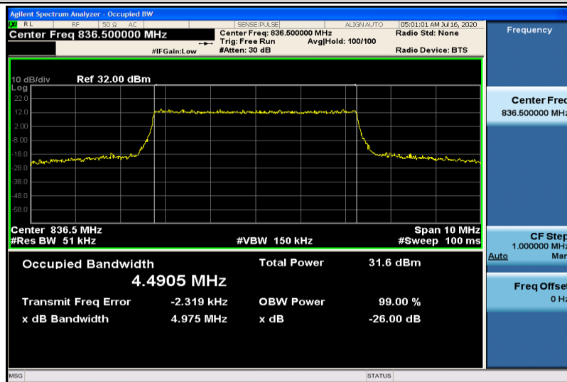
Band5-5MHz-QPSK-20525-25RB#0-4.4905
