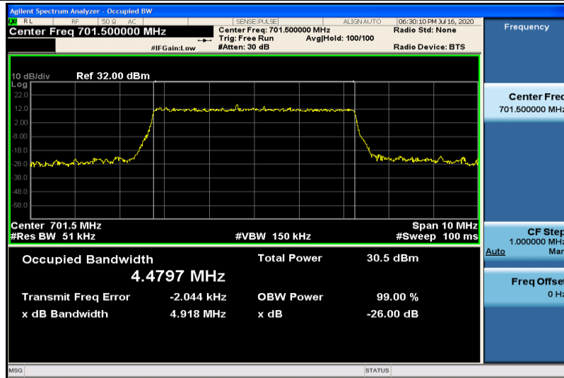
Band12-5MHz-16QAM-23035-25RB#0-4.4797
