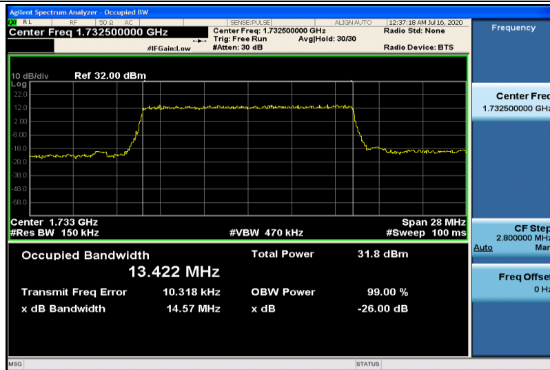
Band4-15MHz-QPSK-20175-75RB#0-13.422
