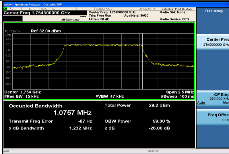
Band4-1.4MHz-QPSK-20393-6RB#0-1.0757
