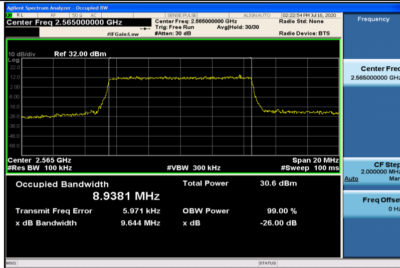
Band7-10MHz-16QAM-21400-50RB#0-8.9381
