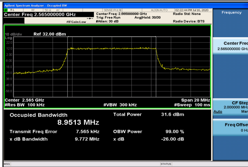
Band7-10MHz-QPSK-21400-50RB#0-8.9513
