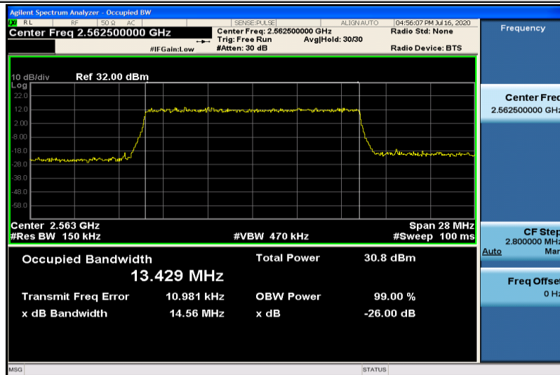
Band7-15MHz-16QAM-21375-75RB#0-13.429
