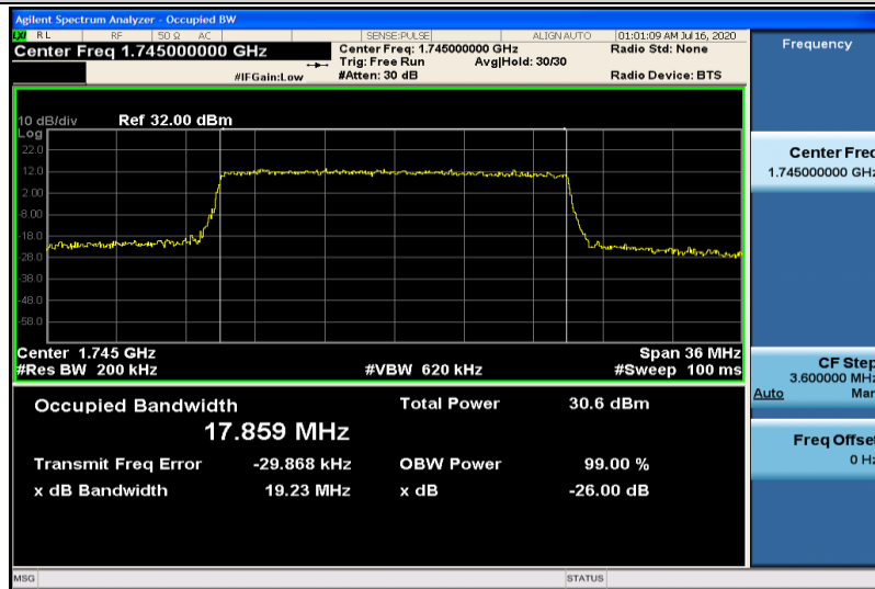
Band4-20MHz-16QAM-20300-100RB#0-17.859
