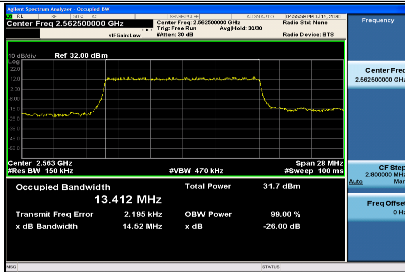
Band7-15MHz-QPSK-21375-75RB#0-13.412
