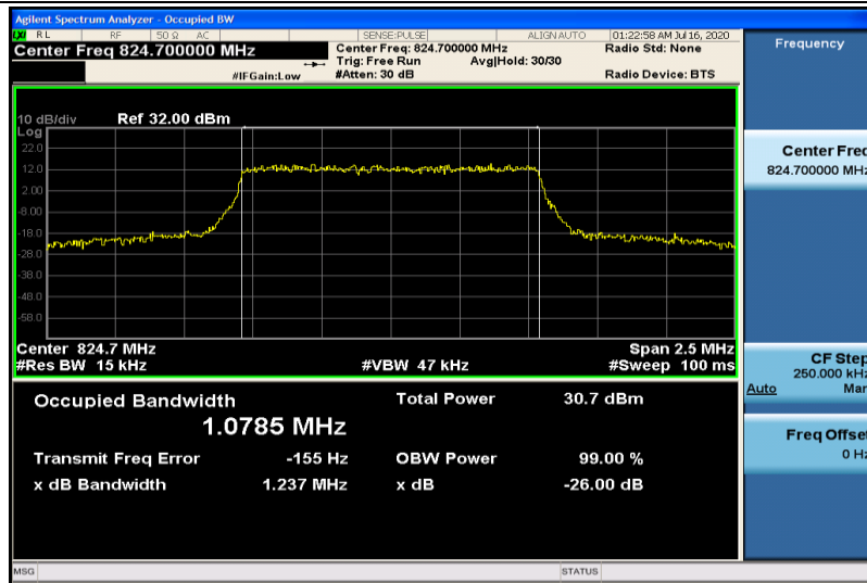
Band5-1.4MHz-QPSK-20407-6RB#0-1.0785
