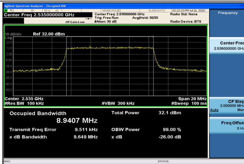
Band7-10MHz-QPSK-21100-50RB#0-8.9407
