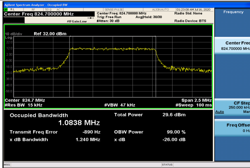
Band5-1.4MHz-16QAM-20407-6RB#0-1.0838
