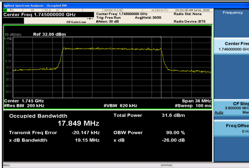
Band4-20MHz-QPSK-20300-100RB#0-17.849
