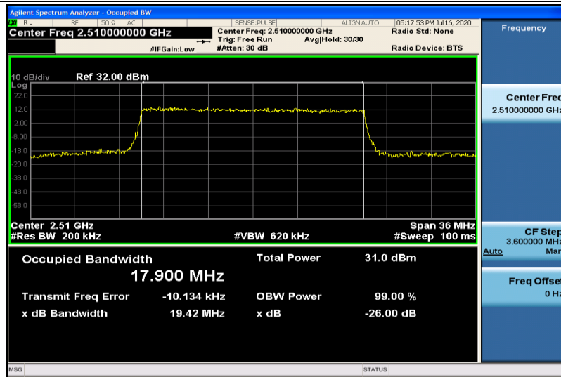
Band7-20MHz-16QAM-20850-100RB#0-17.900
