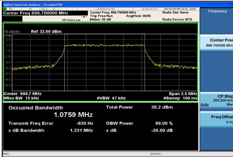
Band12-1.4MHz-QPSK-23017-6RB#0-1.0759
