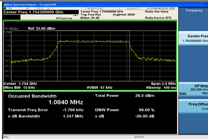
Band4-1.4MHz-16QAM-20393-6RB#0-1.0840
