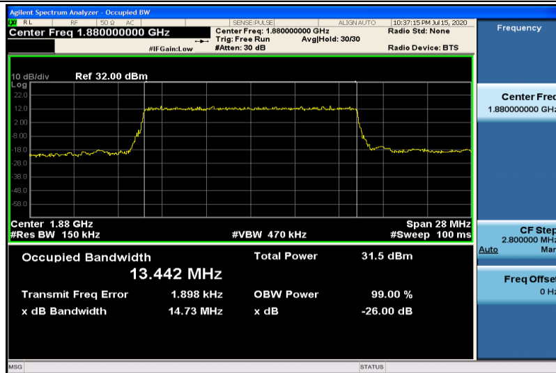
Band2-15MHz-QPSK-18900-75RB#0-13.442
