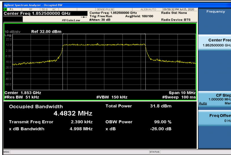
Band2-5MHz-QPSK-18625-25RB#0-4.4832
