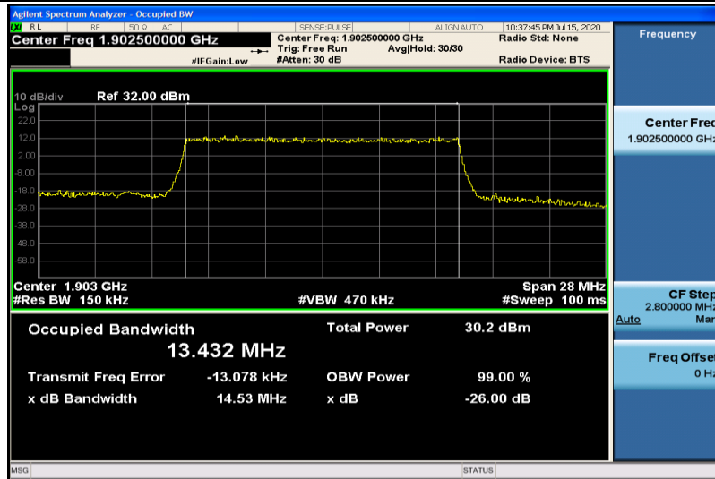
Band2-15MHz-16QAM-19125-75RB#0-13.432
