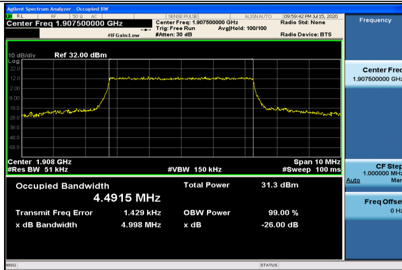
Band2-5MHz-QPSK-19175-25RB#0-4.4915
