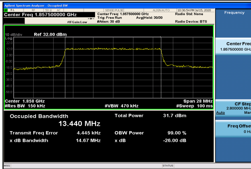
Band2-15MHz-QPSK-18675-75RB#0-13.440
