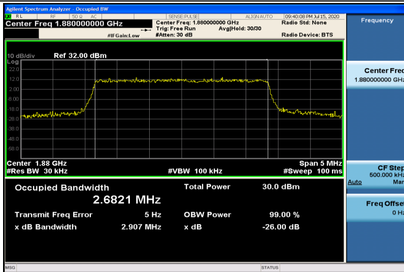
Band2-3MHz-16QAM-18900-15RB#0-2.6821
