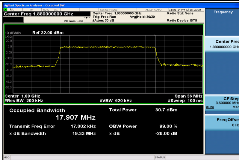
Band2-20MHz-16QAM-18900-100RB#0-17.907
