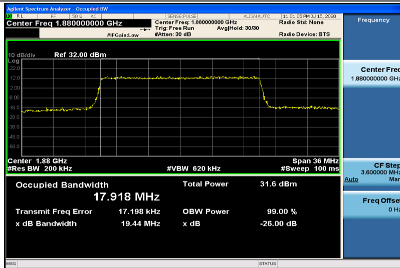
Band2-20MHz-QPSK-18900-100RB#0-17.918
