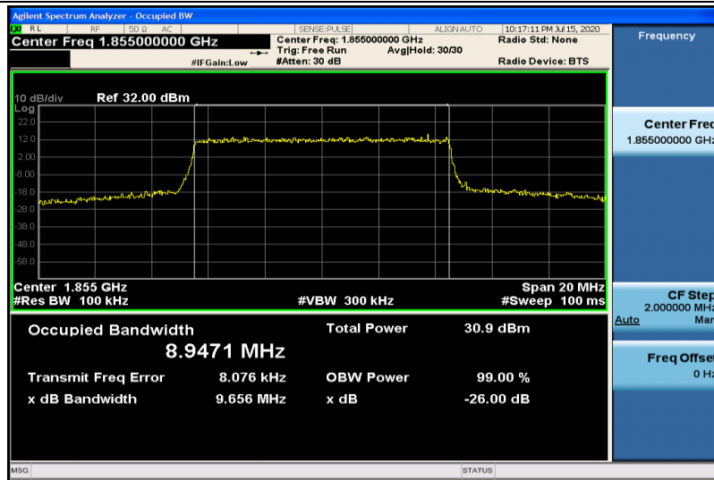
Band2-10MHz-16QAM-18650-50RB#0-8.9471
