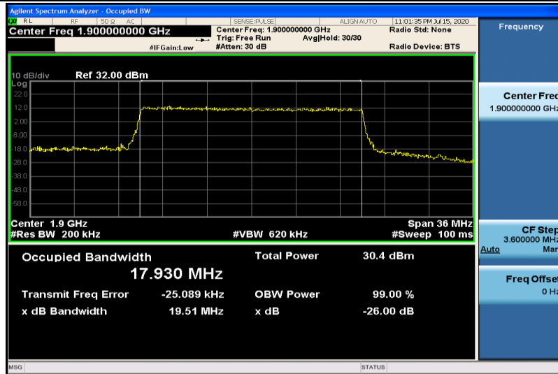
Band2-20MHz-16QAM-19100-100RB#0-17.930
