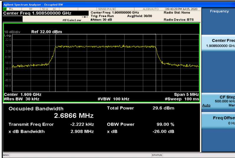
Band2-3MHz-16QAM-19185-15RB#0-2.6866
