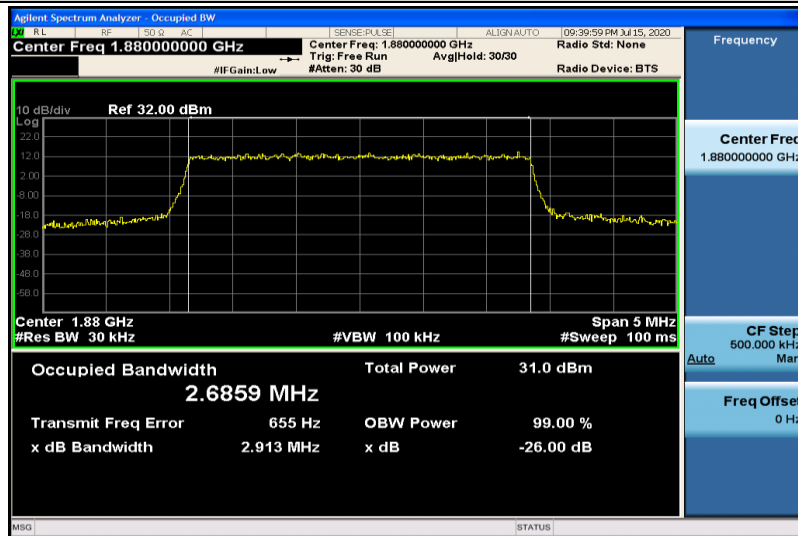
Band2-3MHz-QPSK-18900-15RB#0-2.6859
