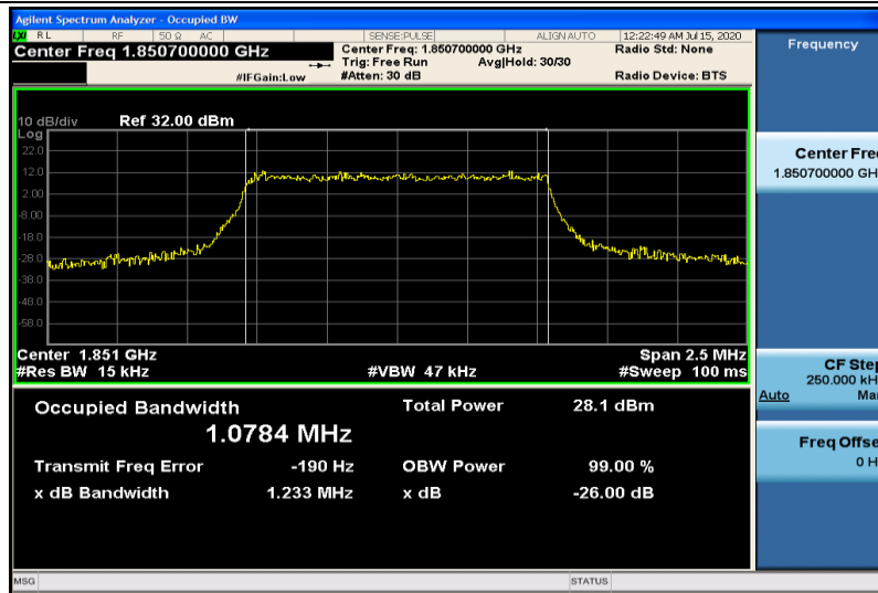
Band2-1.4MHz-16QAM-18607-6RB#0-1.0784
