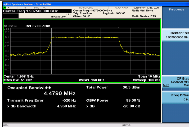
Band2-5MHz-16QAM-19175-25RB#0-4.4790
