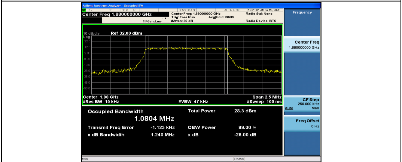
Band2-1.4MHz-QPSK-18900-6RB#0-1.0804
