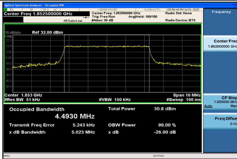
Band2-5MHz-16QAM-18525-25RB#0-4.4930
