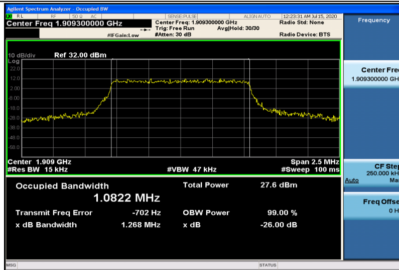
Band2-1.4MHz-16QAM-19193-6RB#0-1.0822
