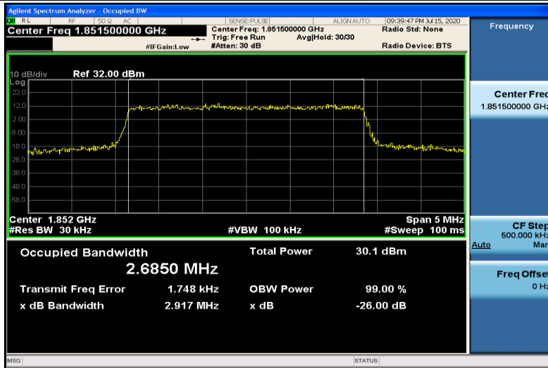
Band2-3MHz-16QAM-18615-15RB#0-2.6850
