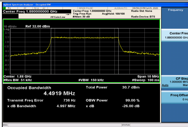
Band2-5MHz-16QAM-18900-25RB#0-4.4919
