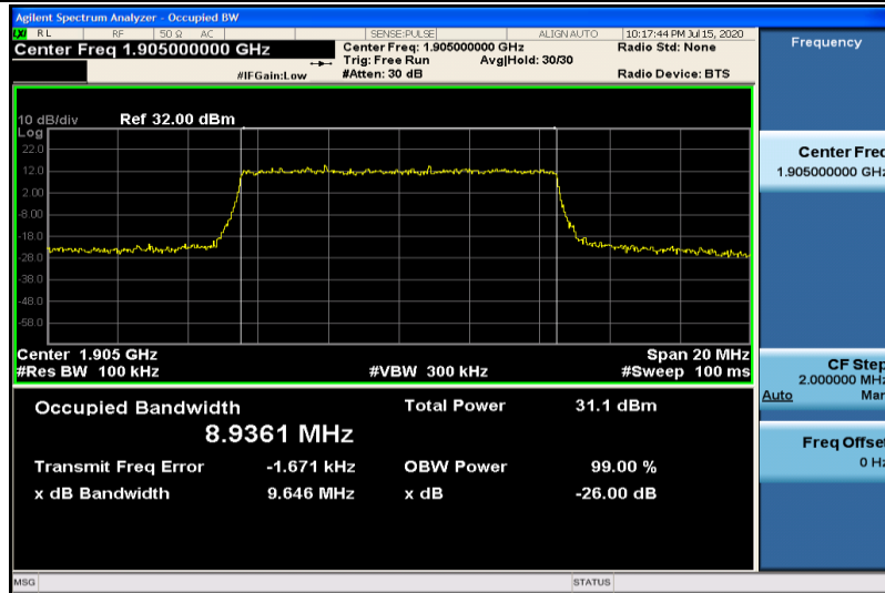
Band2-10MHz-QPSK-19150-50RB#0-8.9361
