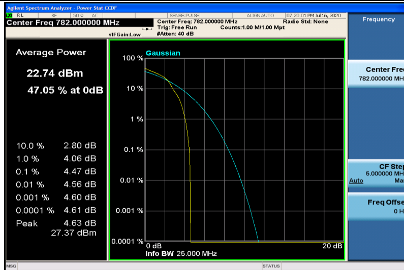
Band13-5MHz-16QAM-23230-1RB#0
