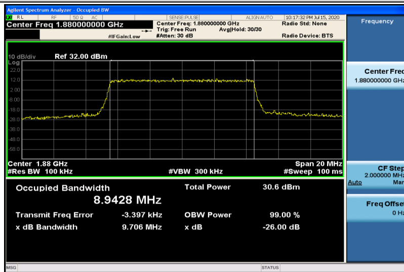
Band2-10MHz-16QAM-18900-50RB#0-8.9428
