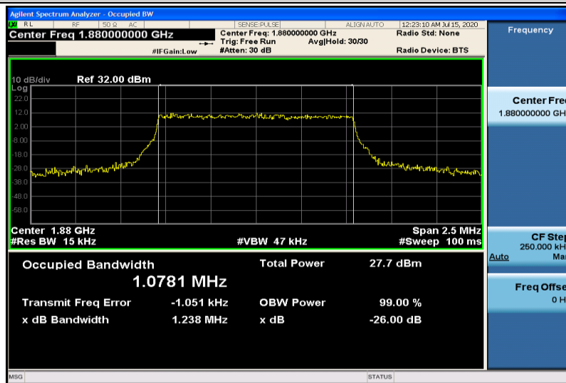
Band2-1.4MHz-16QAM-18900-6RB#0-1.0781
