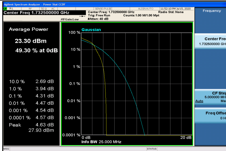
Band4-3MHz-16QAM-20175-1RB#0
